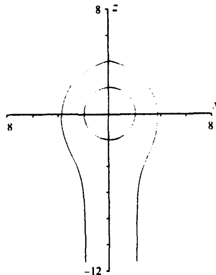
FIGURE 2. The zone of attraction around a sphere of radius a = 2.0 . The buoyancy parameter is \delta = 0.1 .
