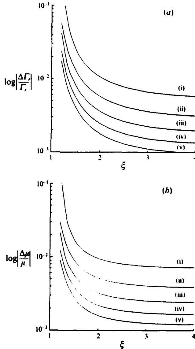
FIGURE 5. The relative error in calculation of (a) \Gamma , and (b) \mu for the example of a sphere of radius 1. The variation of this error with \xi is shown for the mesh sizes: (i) 14 \times 14 , (ii) 19 \times 19 , (iii) 24 \times 24 , (iv) 29 \times 29 , (v) 34 \times 34 .
