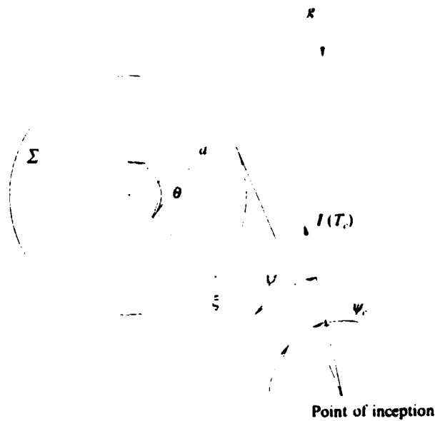
FIGURE 1. The geometry for buoyant cavity motion near a stationary, rigid sphere.
