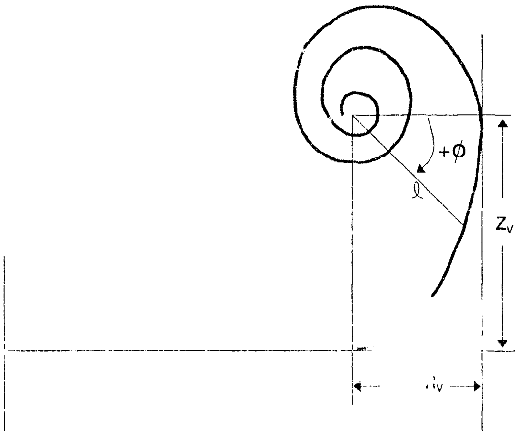
FIGURE 122 LOGARITHMIC SPIRAL REPRESENTATION OF VORTEX ROLLUP
