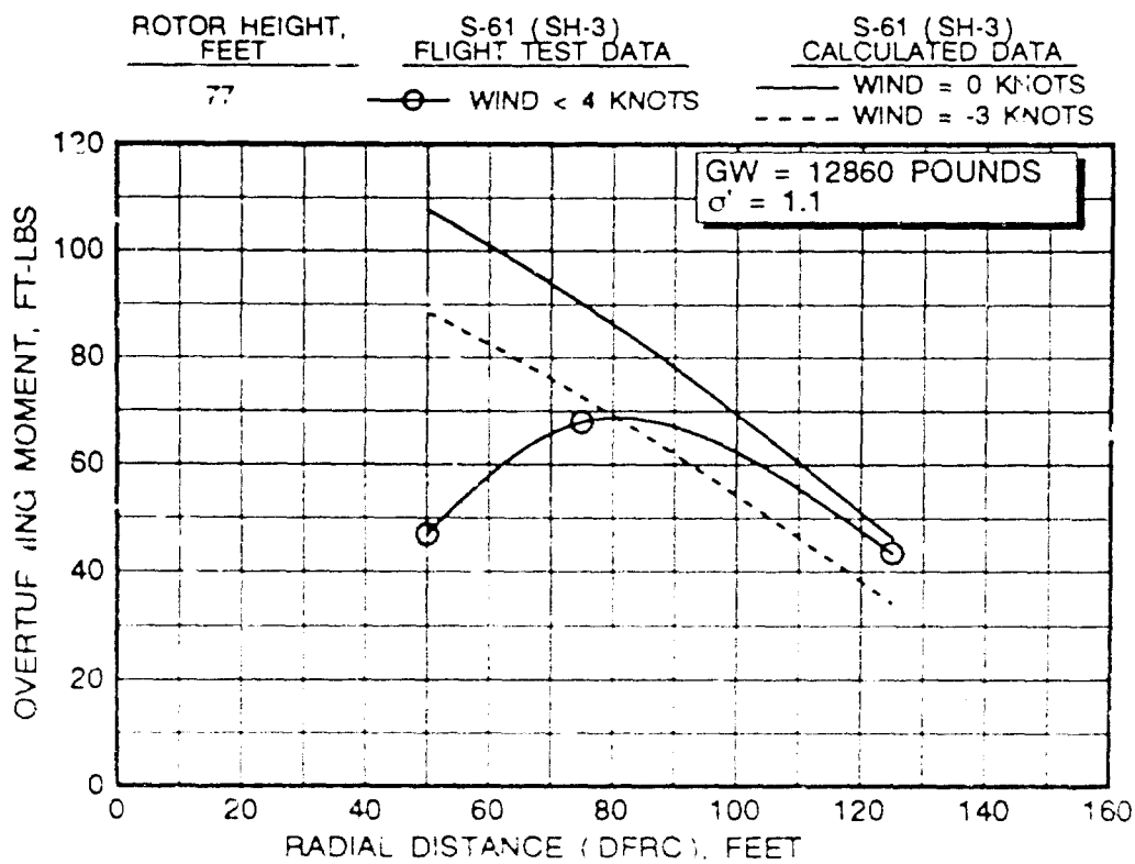
FIGURE 82 CORRELATION OF S-61 (SH-3) PEAK HORIZONTAL OUTWASH MOMENTS DURING HOVER AT ROTOR HEIGHTS OF 57 AND 77 FEET
