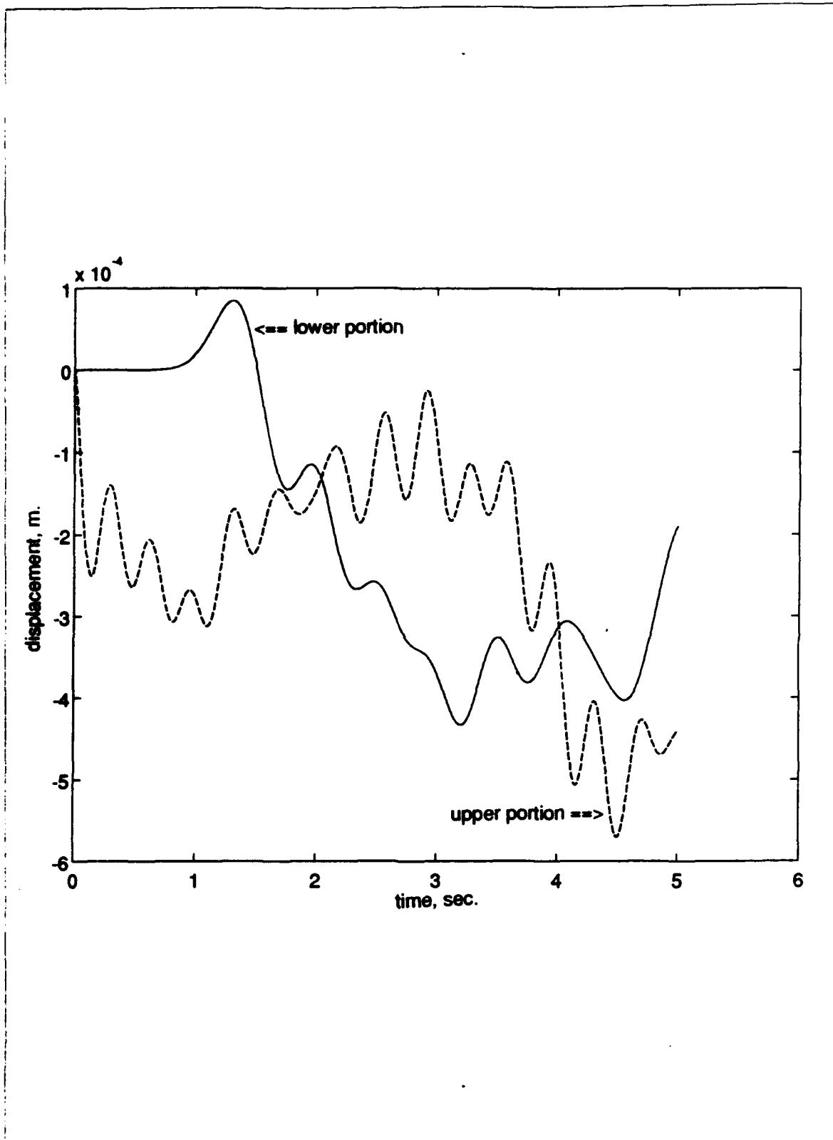
Figure 11 : Displacements of Mid-Points without Contact-Impact Conditions (Large Crack Size )
