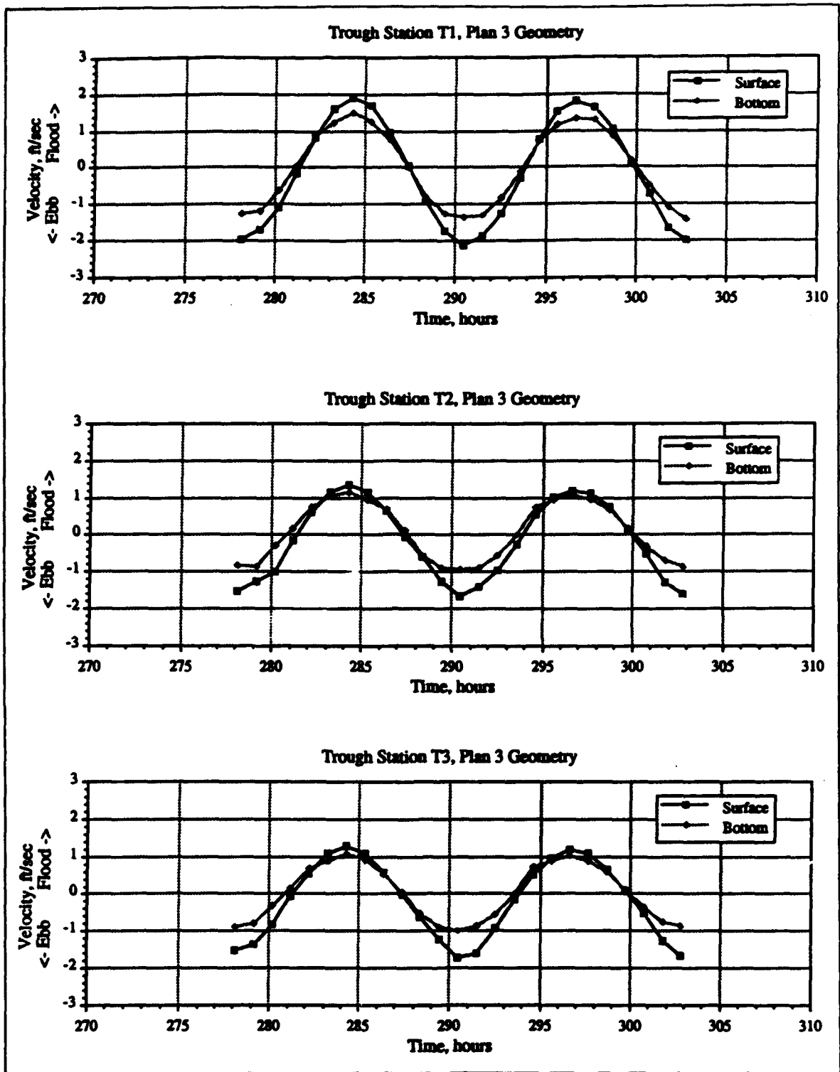
Figure 22. Plan 3 surface and bottom velocities, Stations T1-T3
