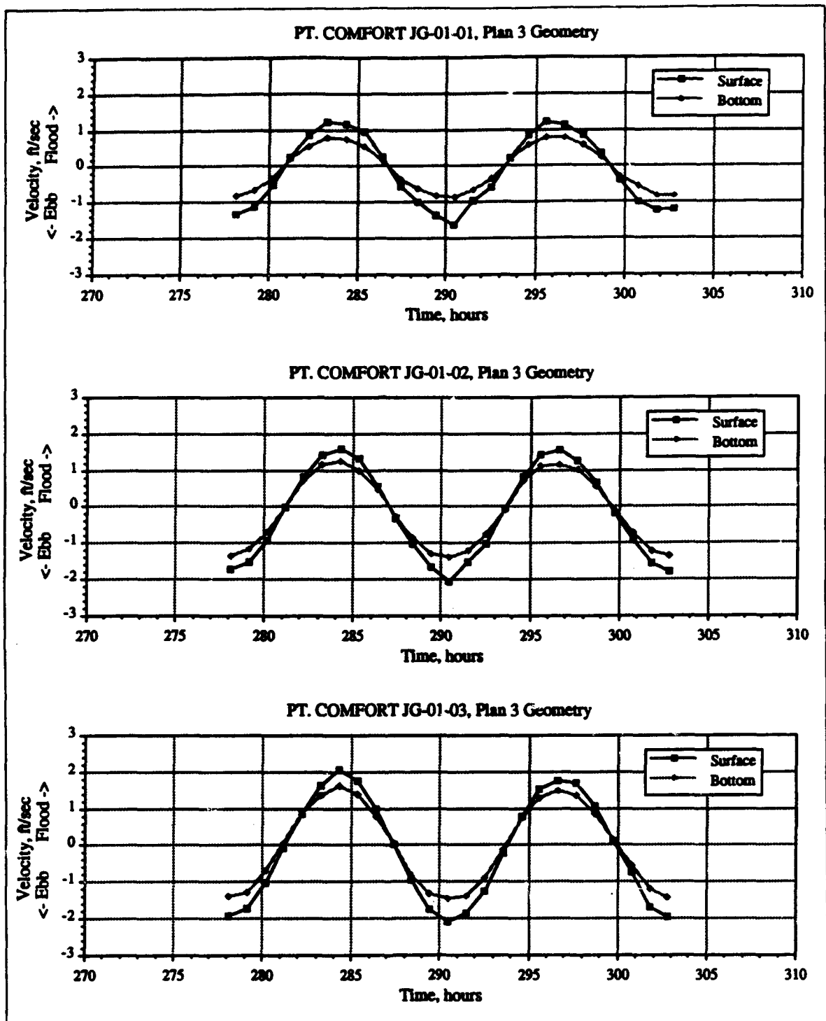
Figure 11. Pt. Comfort surface and bottom velocities, Plan 3
