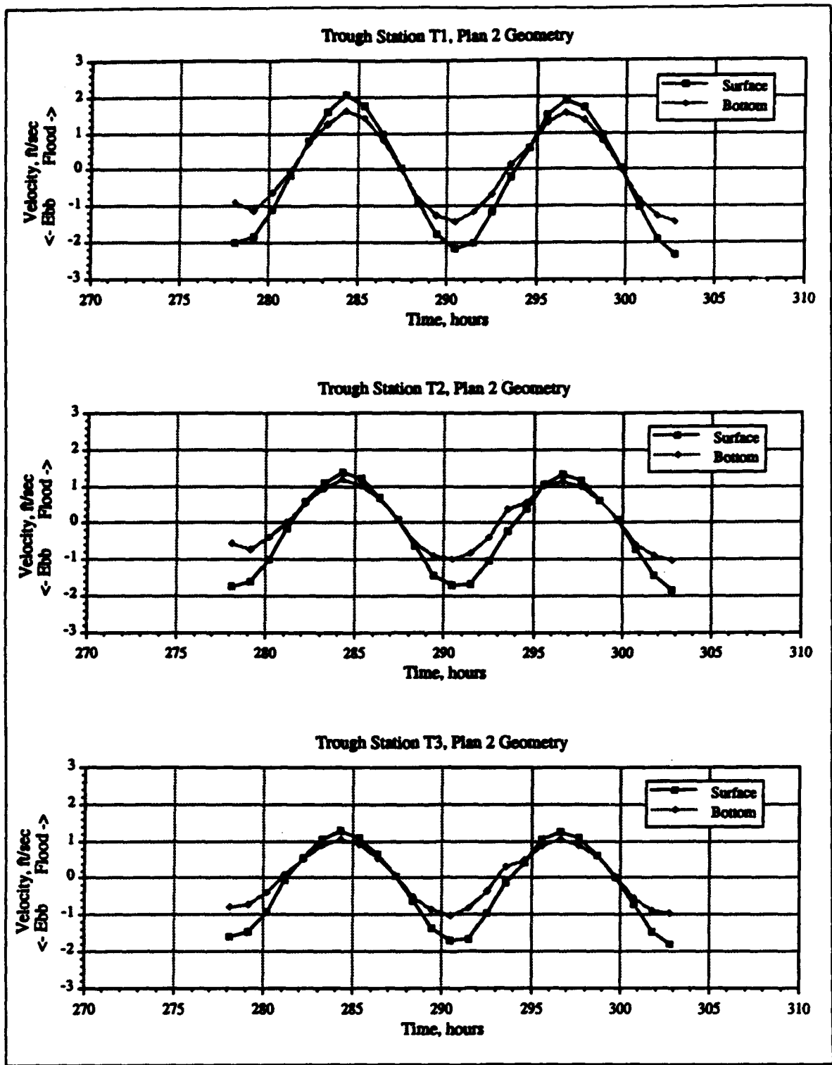
Figure 20. Plan 2 surface and bottom velocities, Stations T1-T3
