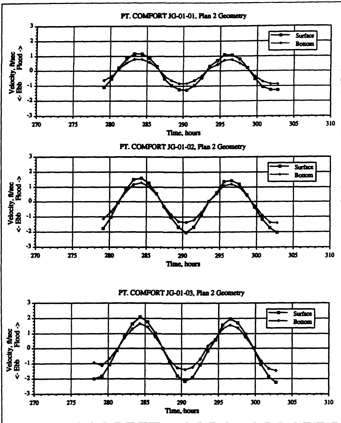
Figure 10. Pt. Comfort surface and bottom velocities, Plan 2
