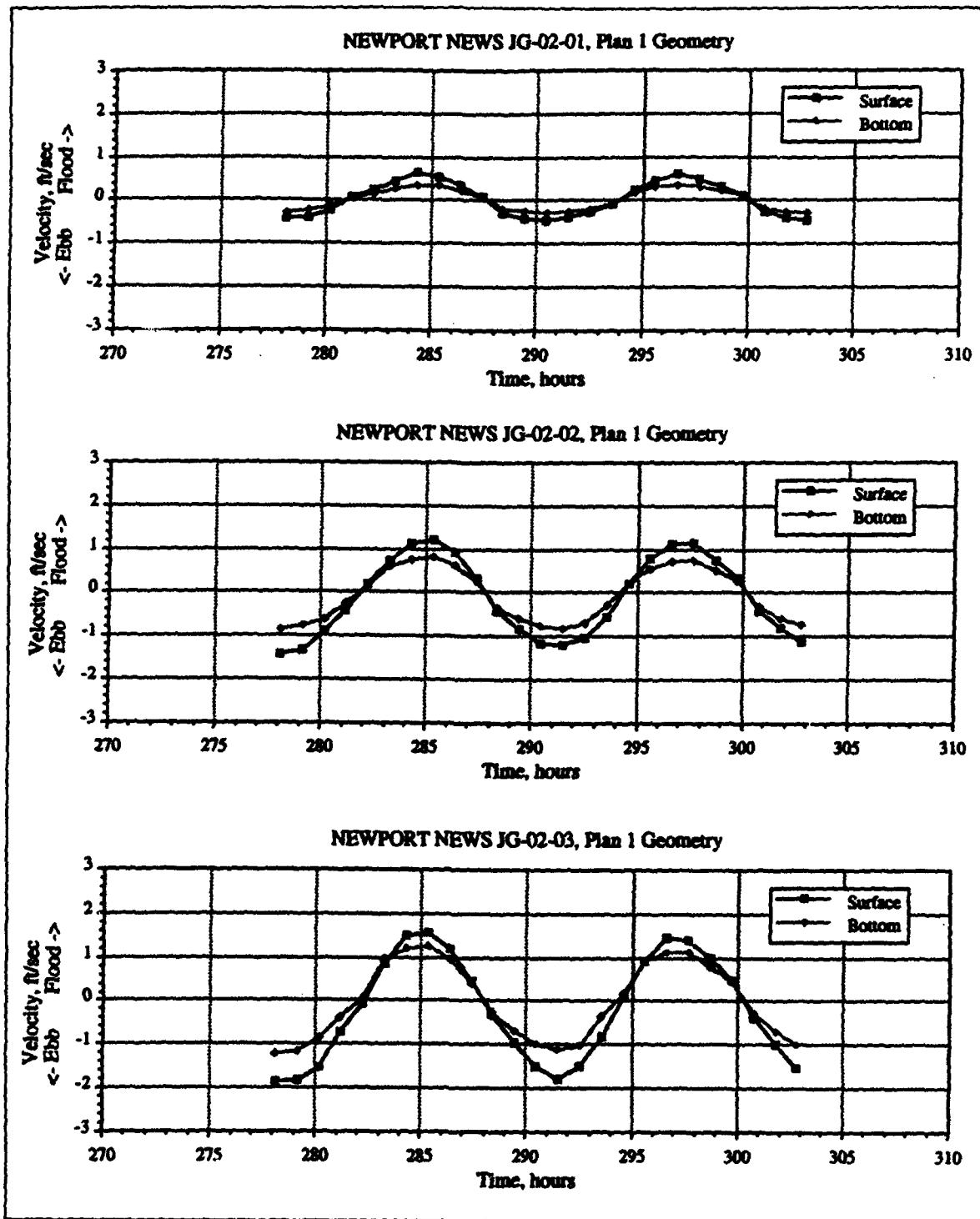
Figure 13. Newport News surface and bottom velocities, Plan 1
