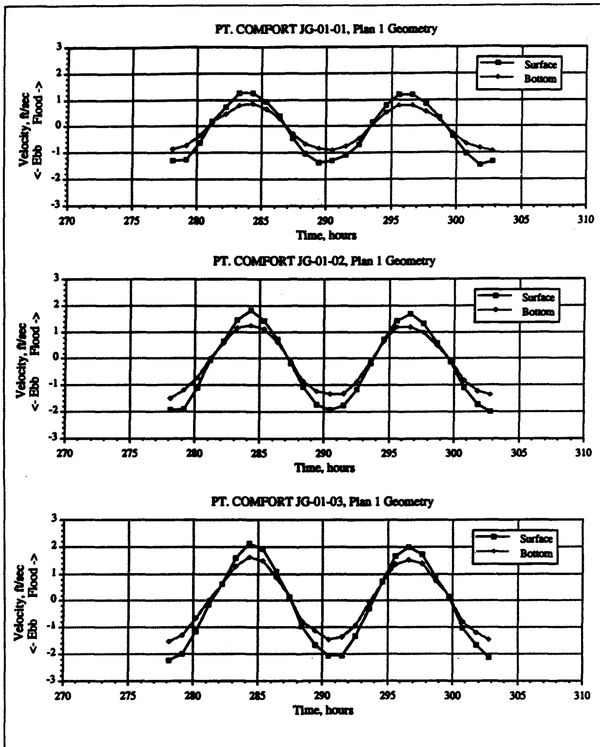
Figure 9. Pt. Comfort surface and bottom velocities, Plan 1
