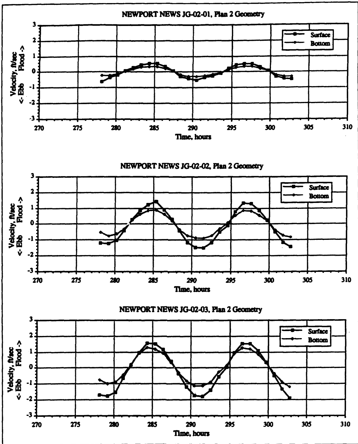
Figure 14. Newport News surface and bottom velocities, Plan 2
