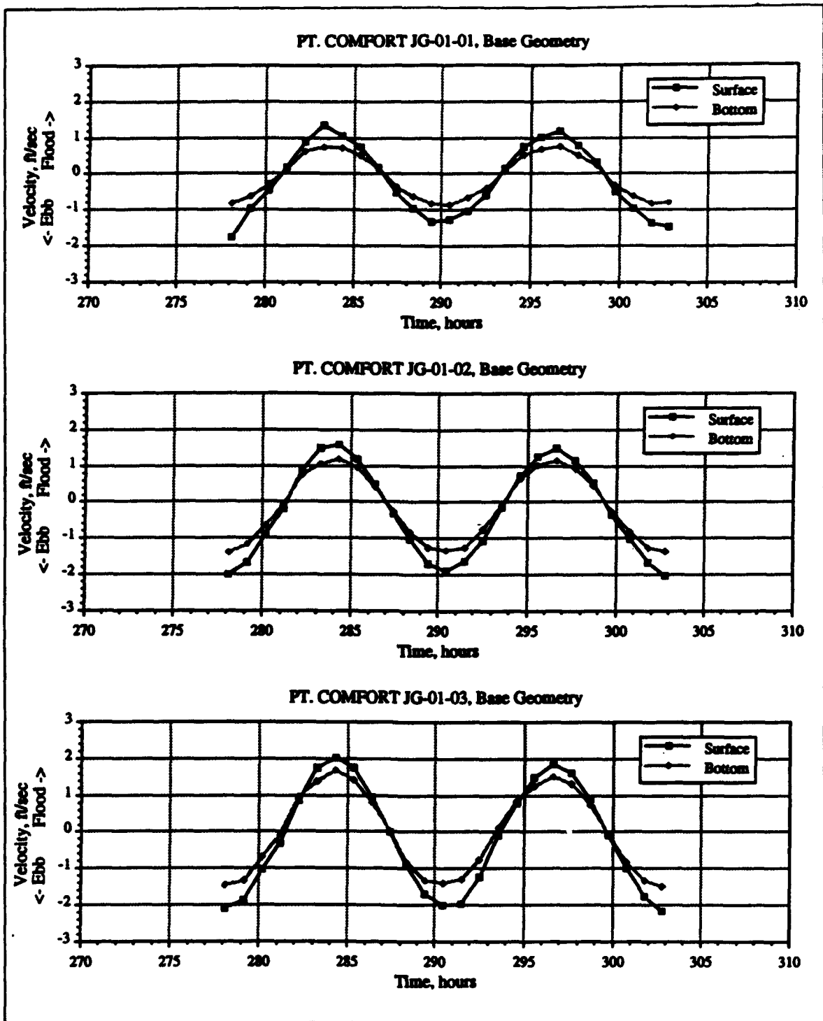
Figure 8. Pt. Comfort surface and bottom velocities, Base
