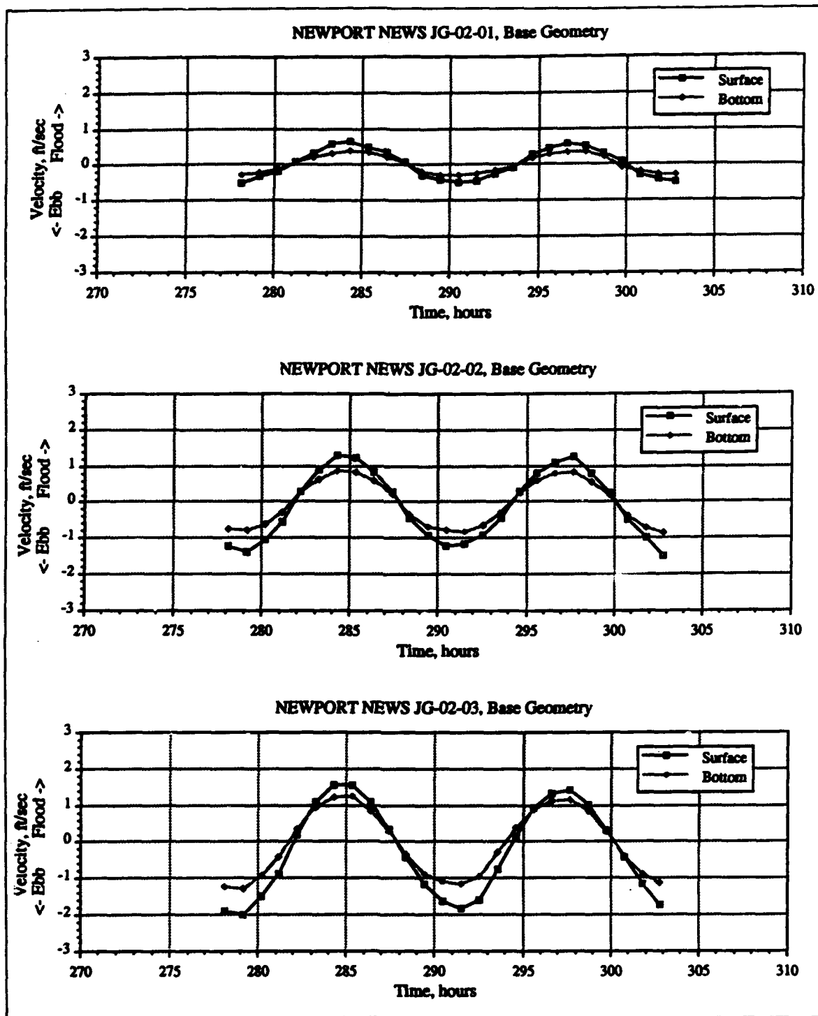
Figure 12. Newport News surface and bottom velocities, Base
