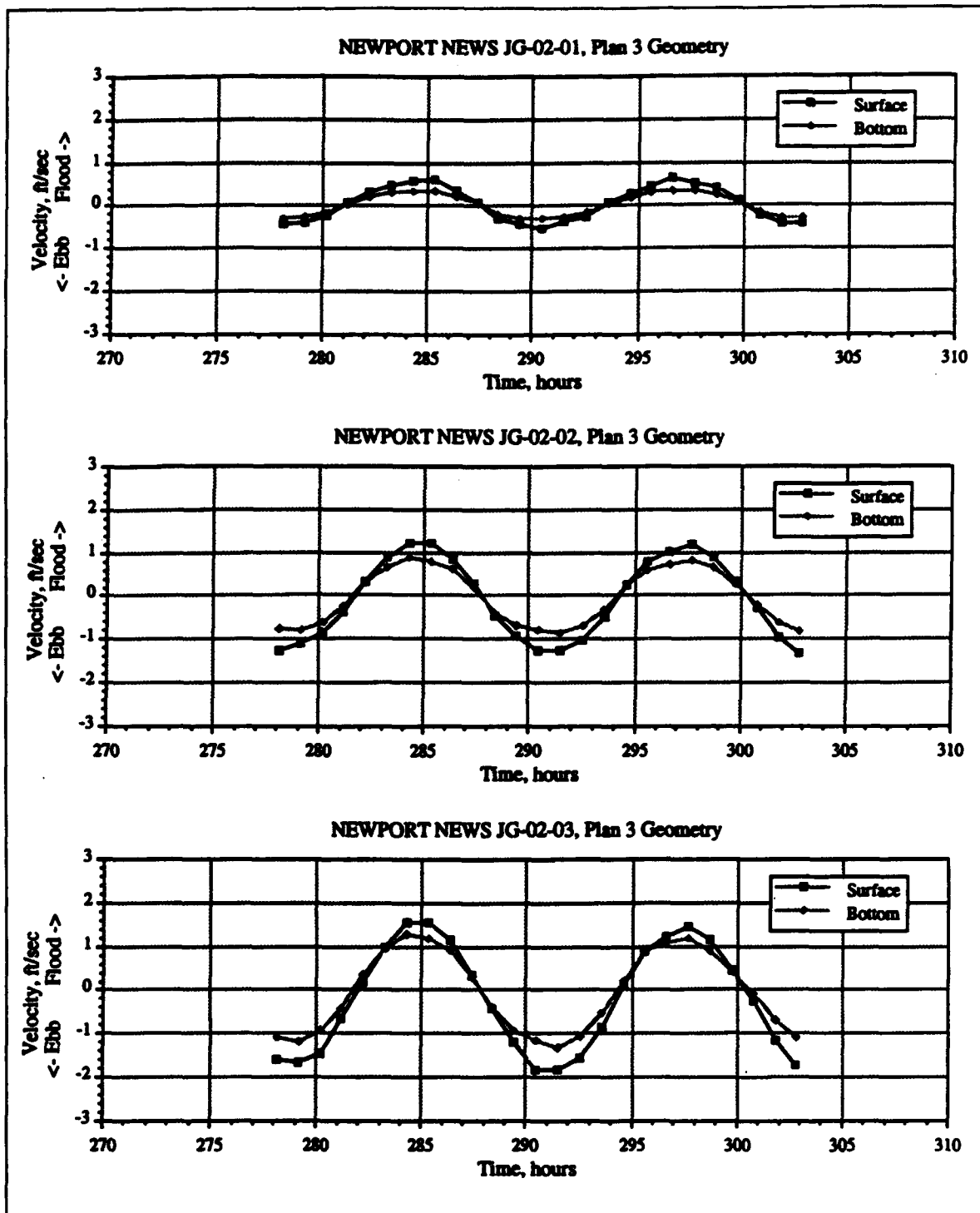
Figure 15. Newport News surface and bottom velocities, Plan 3
