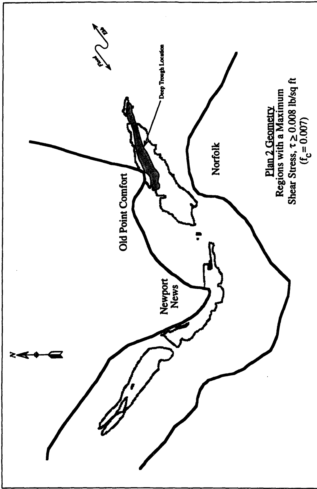
Figure 26. Plan 2 geometry - areas where \tau \geq 0.008 lb/sq ft during the tidal cycle
