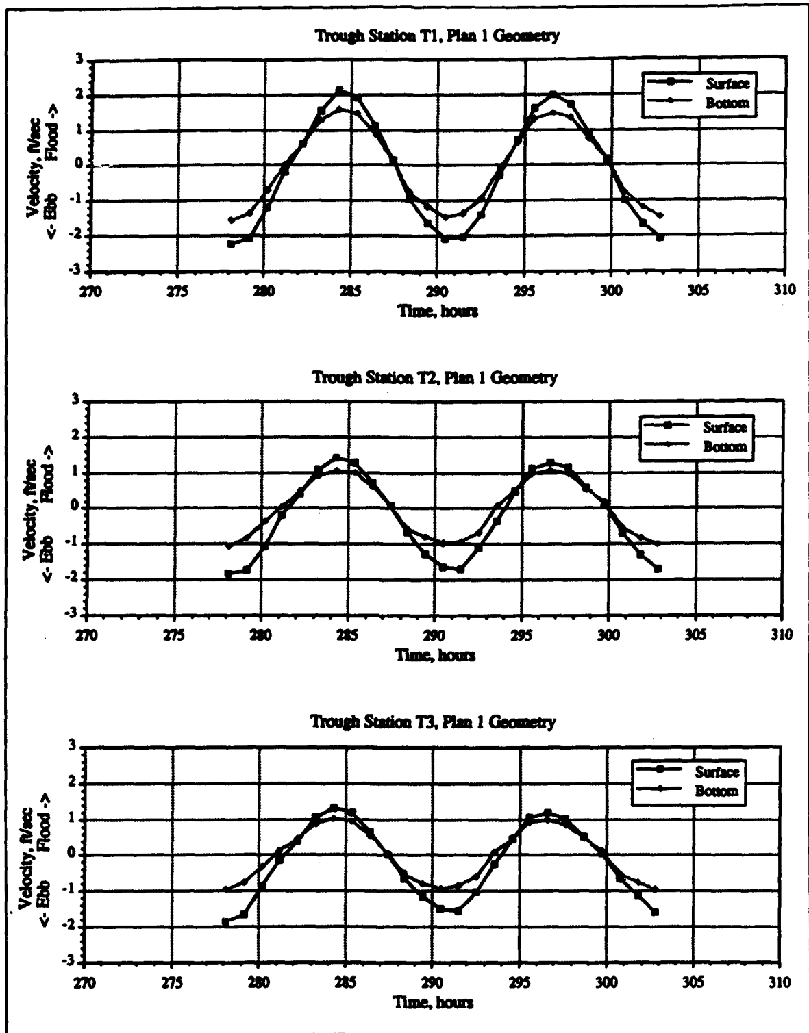
Figure 18. Plan 1 surface and bottom velocities, Stations T1-T3
