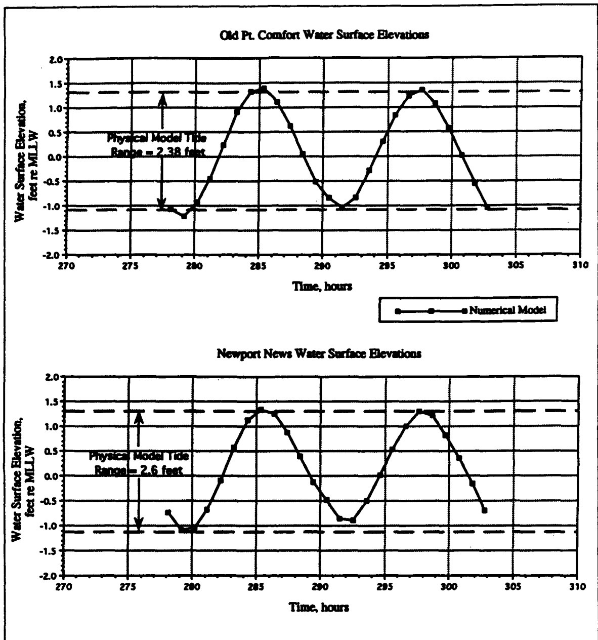
Figure 3. Numerical versus physical model tidal ranges, Lower James River
