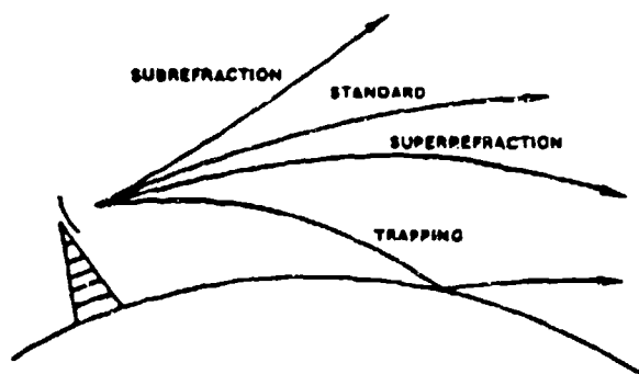
Figure 2-1: Refractive Conditions
