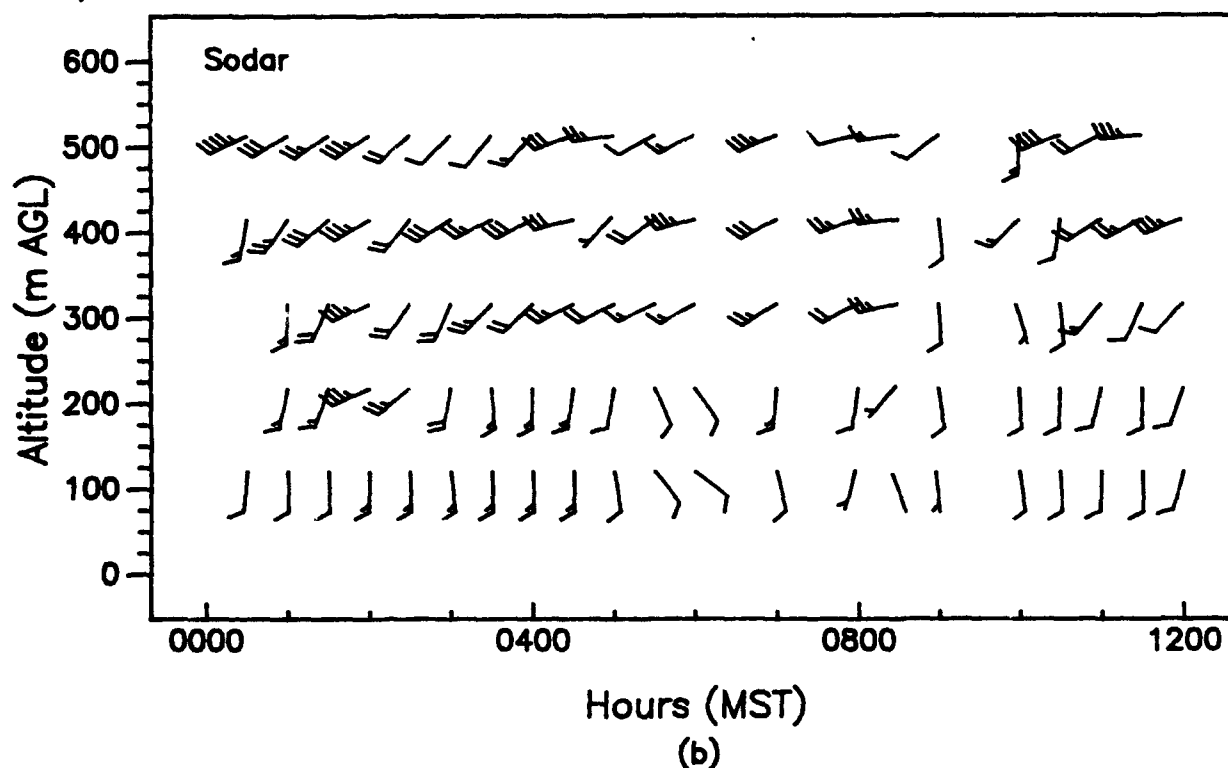
Figure 68. Vertical profiles of wind speed and wind direction, as measured with (a) a 924-MHz profiler and (b) a sodar, APRF site, WSMR, 0000 to 1200 MST, 21 August 1992 (15-min averages).
