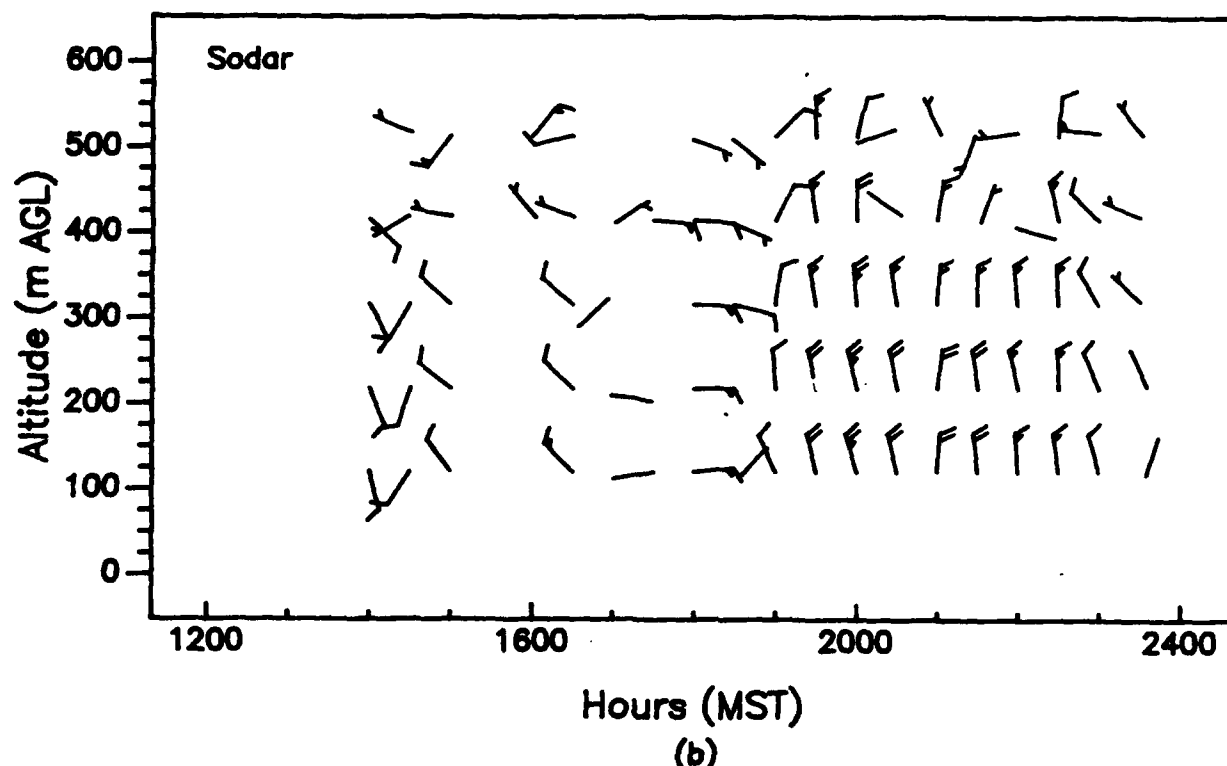
Figure 50. Vertical profiles of wind speed and wind direction, as measured with (a) a 924-MHz profiler and (b) a sodar, APRF site, WSMR, 1200 to 2400 MST, 9 July 1992 (15-min averages).
