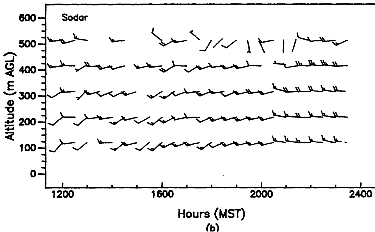
Figure 41. Vertical profiles of wind speed and wind direction, as measured with (a) a 924-MHz profiler and (b) a sodar, APRF site, WSMR, 1200 to 2400 MST, 1 July 1992 (15-min averages).
