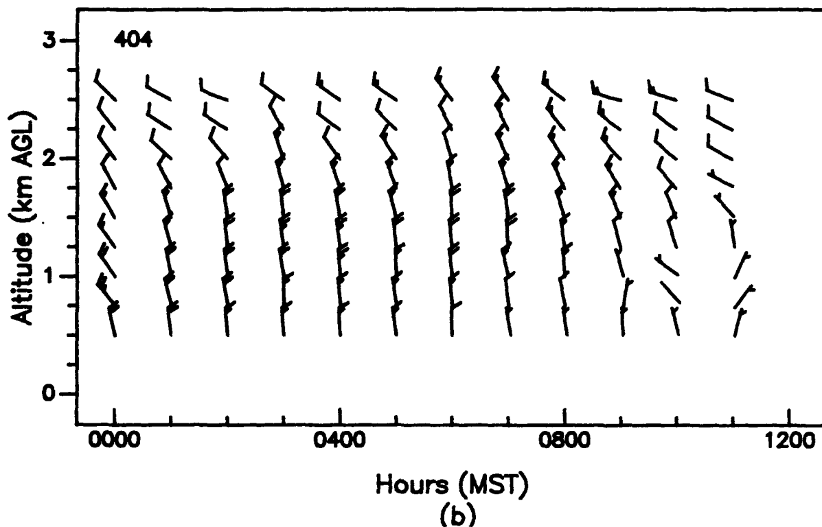
Figure 37. Vertical profiles of wind speed and wind direction, as measured with (a) a 924-MHz profiler and (b) a 404-MHz profiler, APRF site, WSMR, 0000 to 1200 MST, 25 June 1992 (1-h averages).
