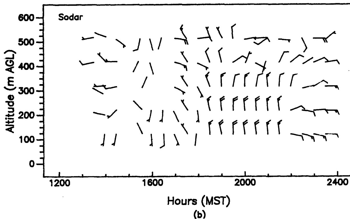
Figure 36. Vertical profiles of wind speed and wind direction, as measured with (a) a 924-MHz profiler and (b) a sodar, APRF site, WSMR, 1200 to 2400 MST, 25 June 1992 (15-min averages).
