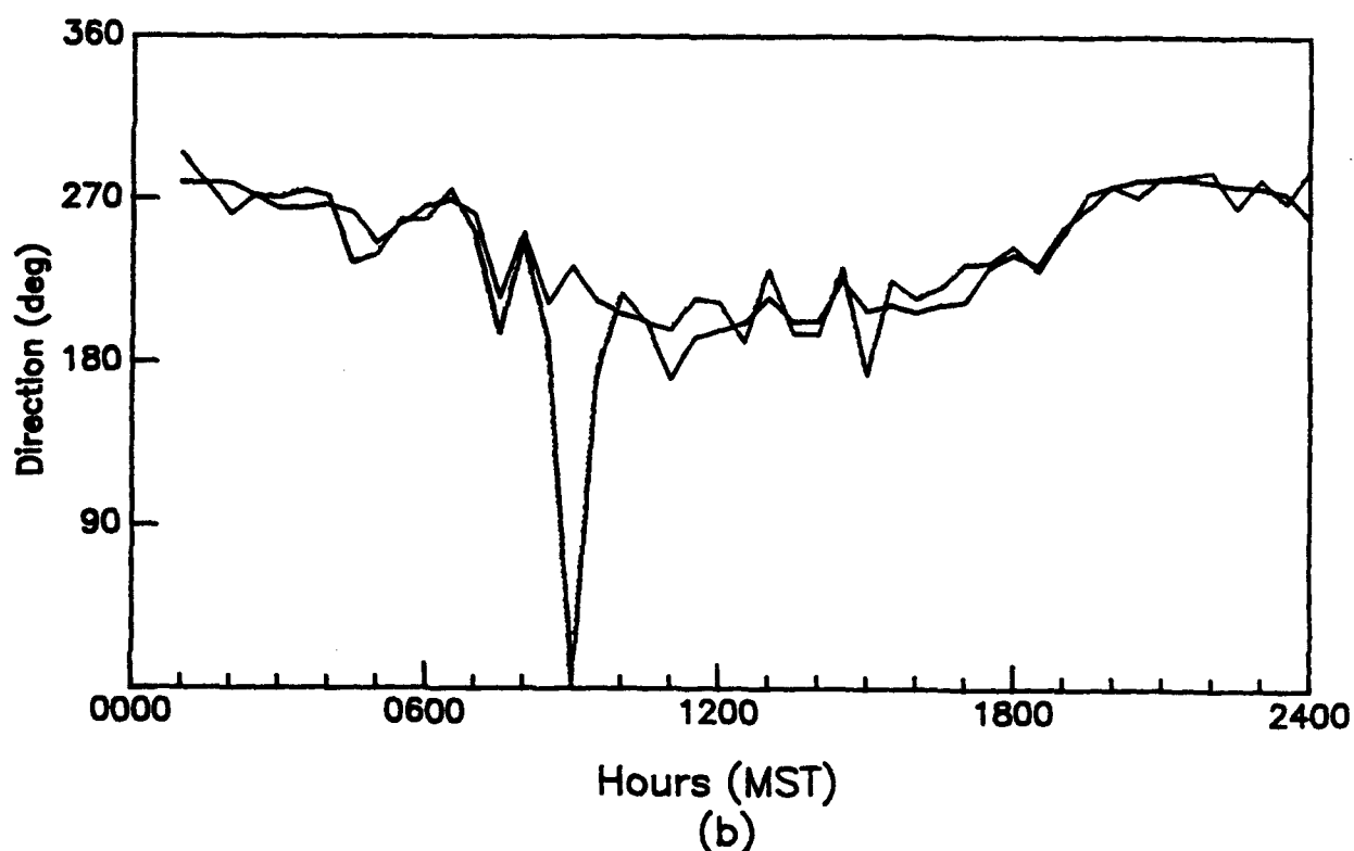
Figure 87. Diurnal variation of (a) wind speed and (b) wind direction as measured with a 924-MHz profiler at 218 m AGL and a sodar at 175, 200, 225, and 250 m AGL, APRF site, WSMR, 0000 to 2400 MST, 15 April 1992 (30-min averages).
