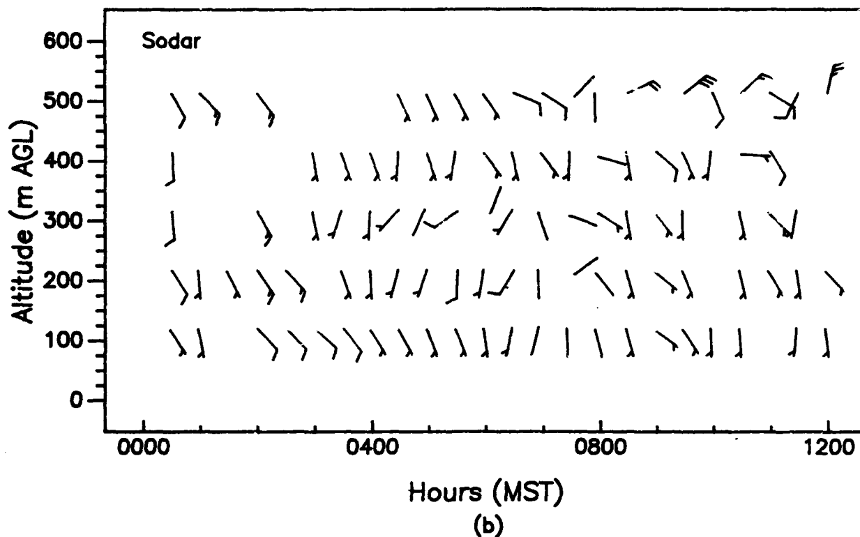
Figure 56. Vertical profiles of wind speed and wind direction, as measured with (a) a 924-MHz profiler and (b) a sodar, APRF site, WSMR, 0000 to 1200 MST, 19 August 1992 (15-min averages).
