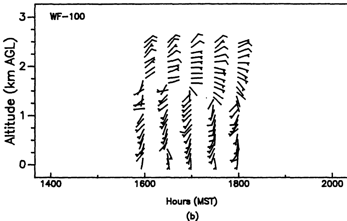
Figure 60. Vertical profiles of wind speed and wind direction, as measured with (a) a 924-MHz profiler at APRF site and (b) a WF-100 radar at Oasis site, WSMR, 1400 to 2000 MST, 20 August 1992 (15-min averages for the 924 data).
