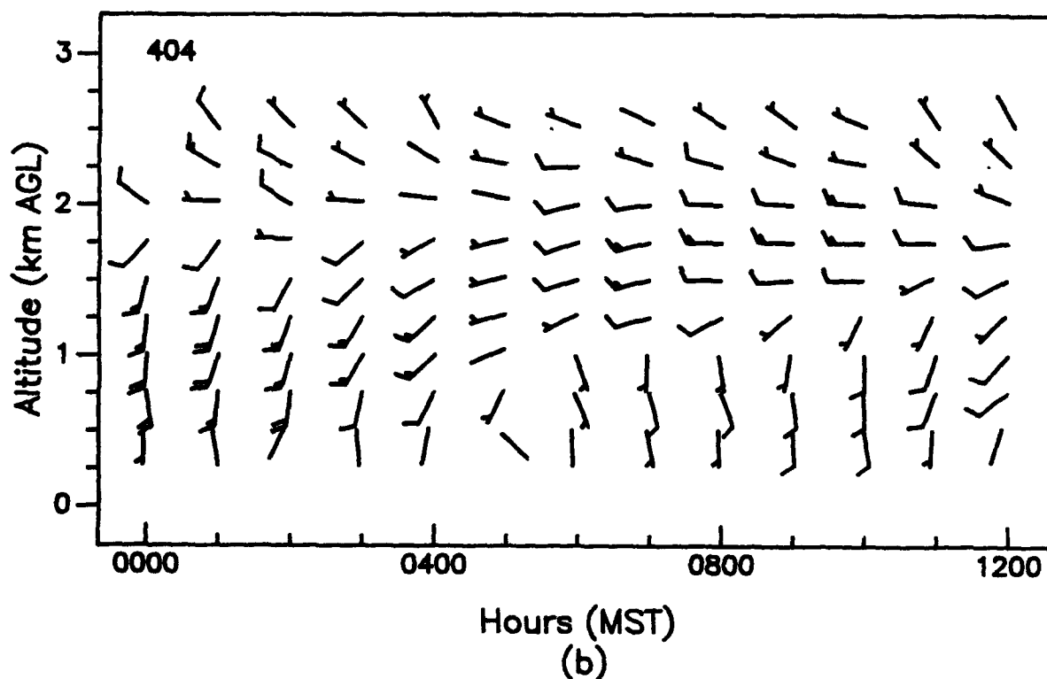
Figure 70. Vertical profiles of wind speed and wind direction, as measured with (a) a 924-MHz profiler and (b) a 404-MHz profiler, APRF site, WSMR, 0000 to 1200 MST, 21 August 1992 (1-h averages).
