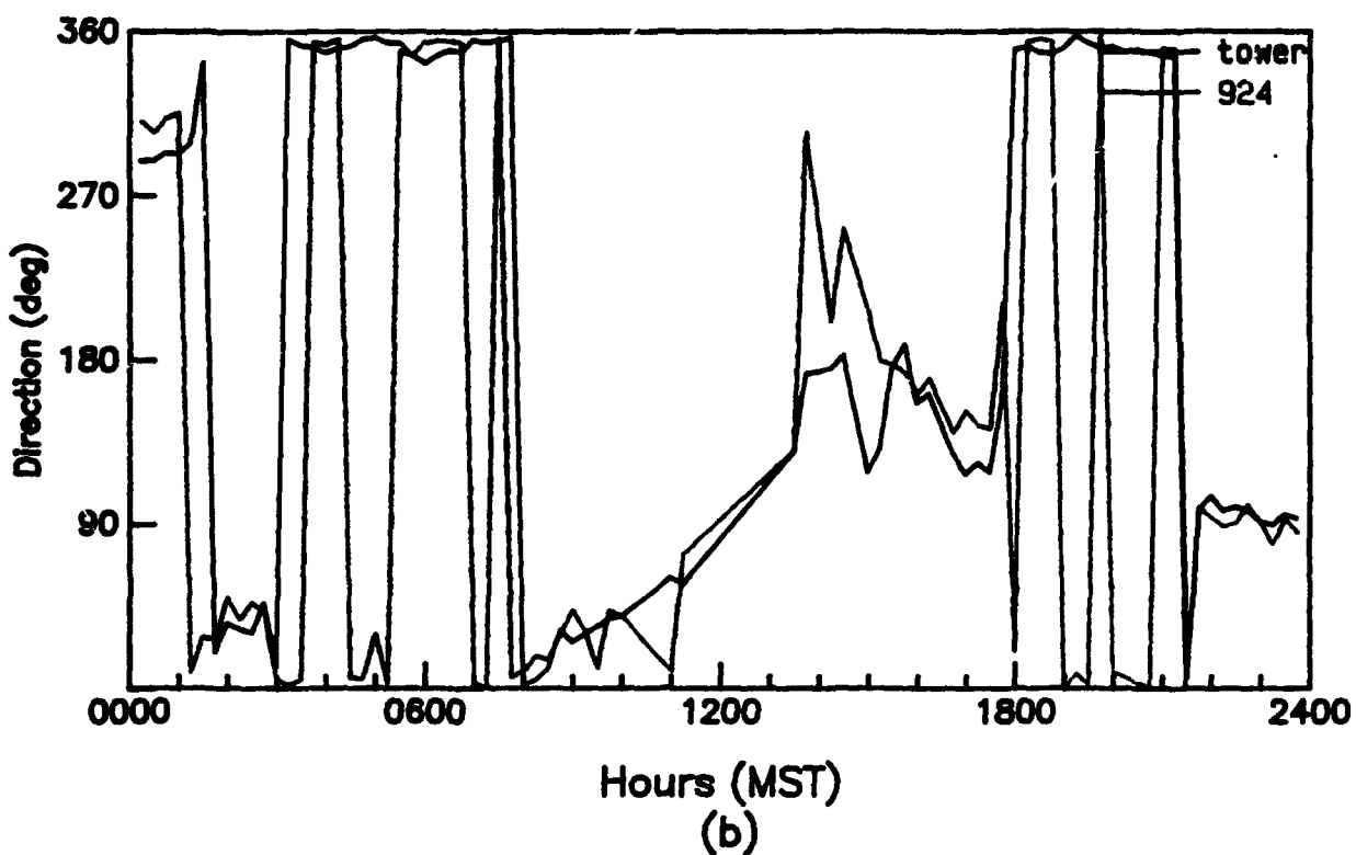
Figure 34. Diurnal variation of (a) wind speed and (b) wind direction as measured with a 924-MHz profiler at 120 m AGL (APRF site) and tower-mounted anemometers at 90, 120, and 150 m AGL (LC-35), WSMR, 0000 to 2400 MST, 25 June 1992 (15-min averages).
