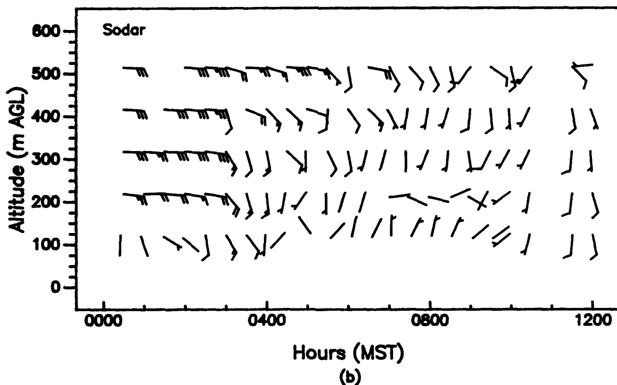
Figure 23. Vertical profiles of wind speed and wind direction, as measured with (a) a 924-MHz profiler and (b) a sodar, APRF site, WSMR, 0000 to 1200 MST, 18 June 1992 (15-min averages).
