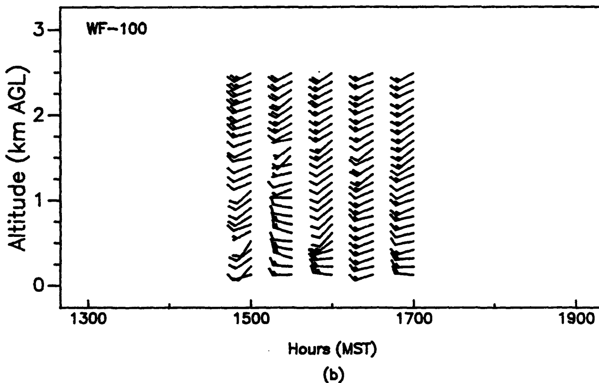
Figure 72. Vertical profiles of wind speed and wind direction, as measured with (a) a 924-MHz profiler at APRF site and (b) a WF-100 radar at Oasis site, WSMR, 1300 to 1900 MST, 24 August 1992 (15-min averages for the 924 data).
