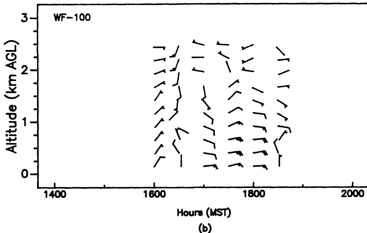
Figure 48. Vertical profiles of wind speed and wind direction, as measured with (a) a 924-MHz profiler at APRF site and (b) a WF-100 radar at Oasis site, WSMR, 1400 to 2000 MST, 9 July 1992 (15-min averages for the 924 data).
