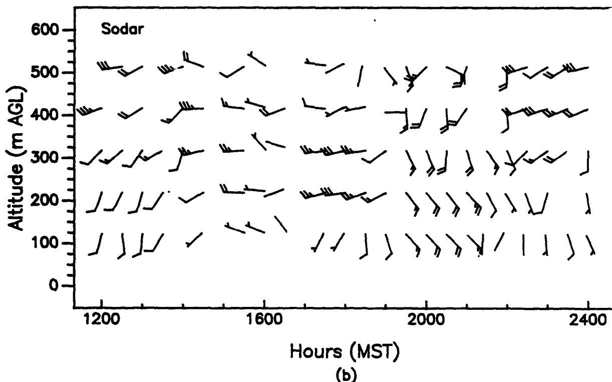
Figure 69. Vertical profiles of wind speed and wind direction, as measured with (a) a 924-MHz profiler and (b) a sodar, APRF site, WSMR, 1200 to 2400 MST, 21 August 1992 (15-min averages).
