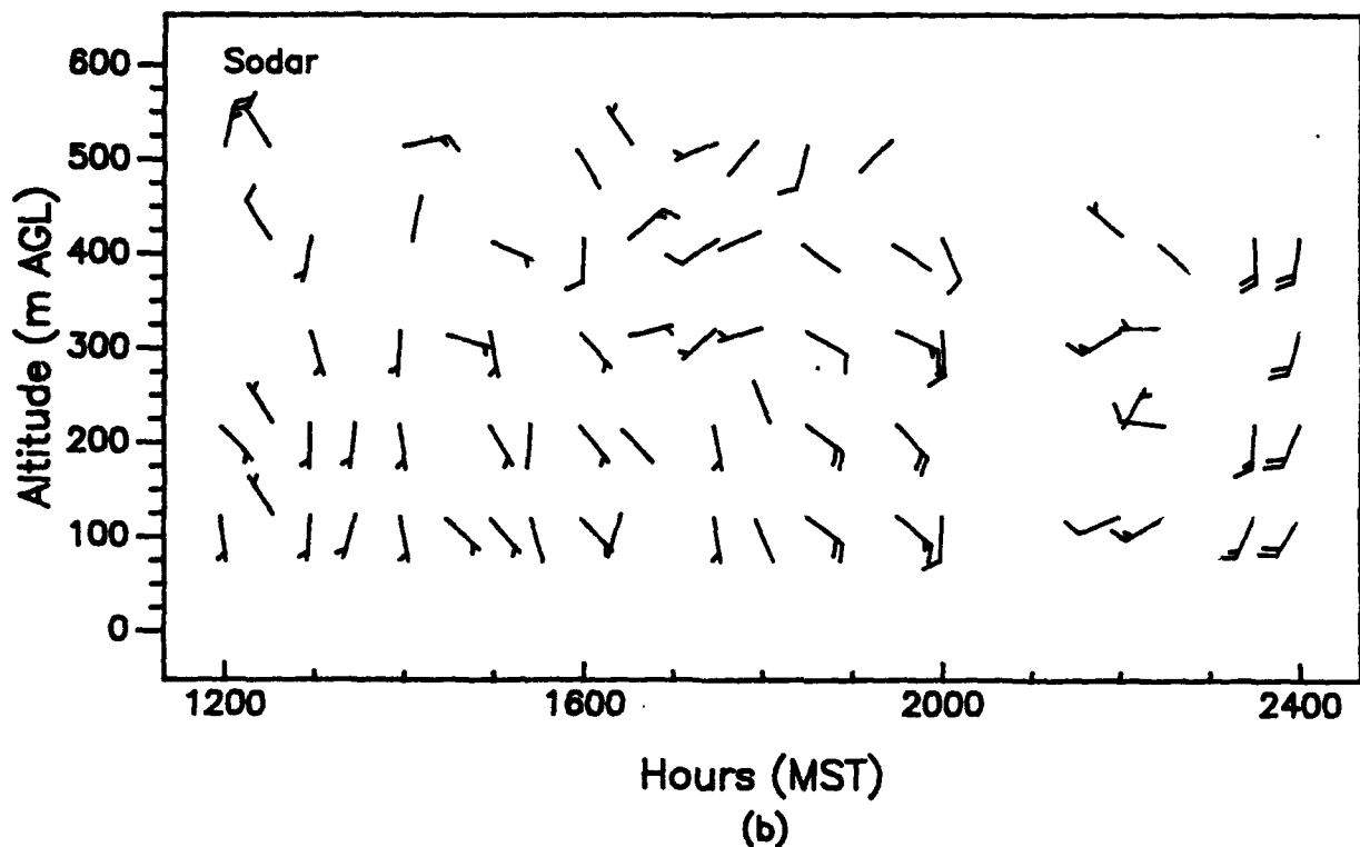
Figure 57. Vertical profiles of wind speed and wind direction, as measured with (a) a 924-MHz profiler and (b) a sodar, APRF site, WSMR, 1200 to 2400 MST, 19 August 1992 (15-min averages).
