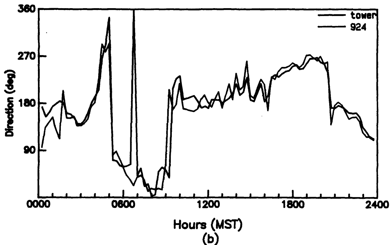
Figure 22. Diurnal variation of (a) wind speed and (b) wind direction as measured with a 924-MHz profiler at 120 m AGL (APRF site) and tower-mounted anemometers at 90, 120, and 150 m AGL (LC-35), WSMR, 0000 to 2400 MST, 18 June 1992 (15-min averages).
