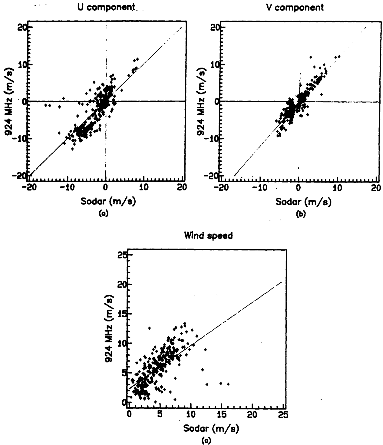
Figure E-2. Regression lines for (a) U component, (b) V component, and (c) resultant wind speed based on measurements with a 924-MHz wind profiler and a sodar, APRF site, WSMR, during 13 of 14 WF-100 measurement periods listed in table 3 (15-min averages).
