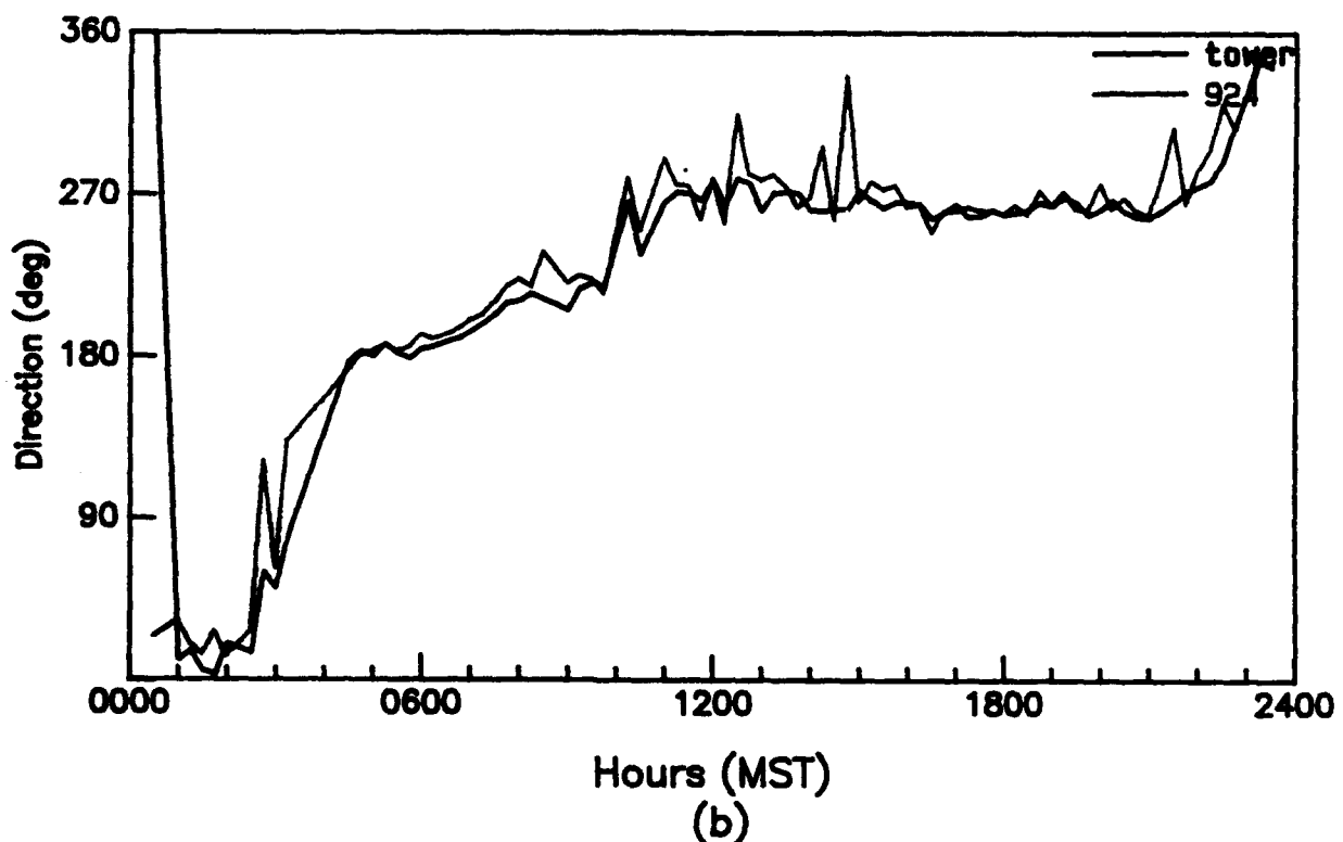
Figure 73. Diurnal variation of (a) wind speed and (b) wind direction as measured with a 924-MHz profiler at 120 m AGL (APRF site) and tower-mounted anemometers at 90, 120, and 150 m AGL (LC-35), WSMR, 0000 to 2400 MST, 24 August 1992 (15-min averages).
