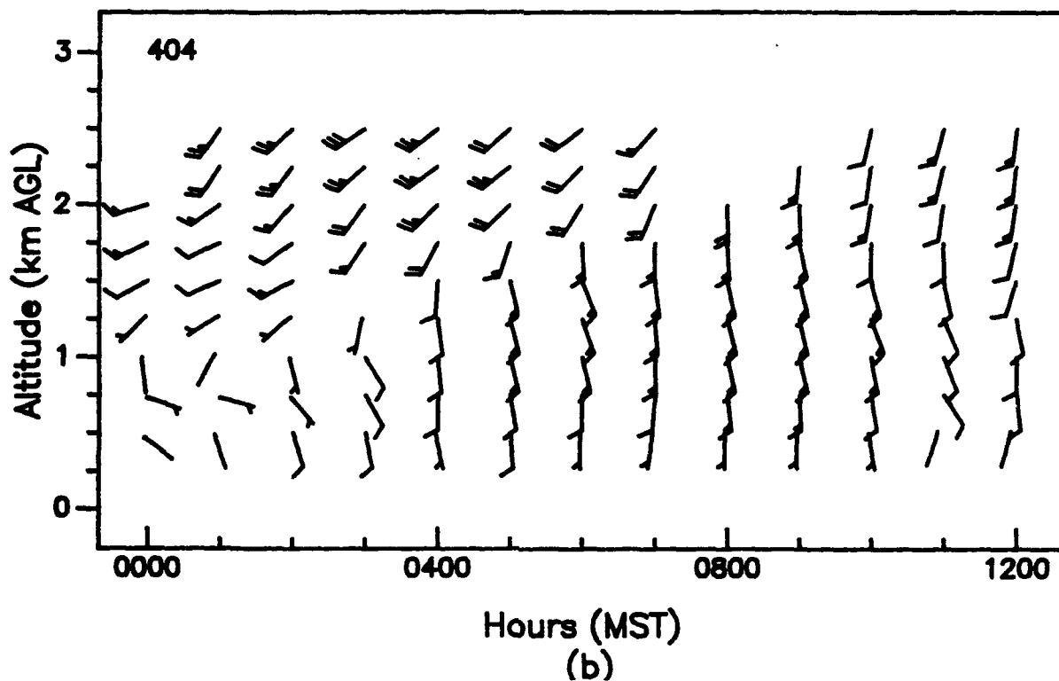
Figure 25. Vertical profiles of wind speed and wind direction, as measured with (a) a 924-MHz profiler and (b) a 404-MHz profiler, APRF site, WSMR, 0000 to 1200 MST, 18 June 1992 (1-h averages).
