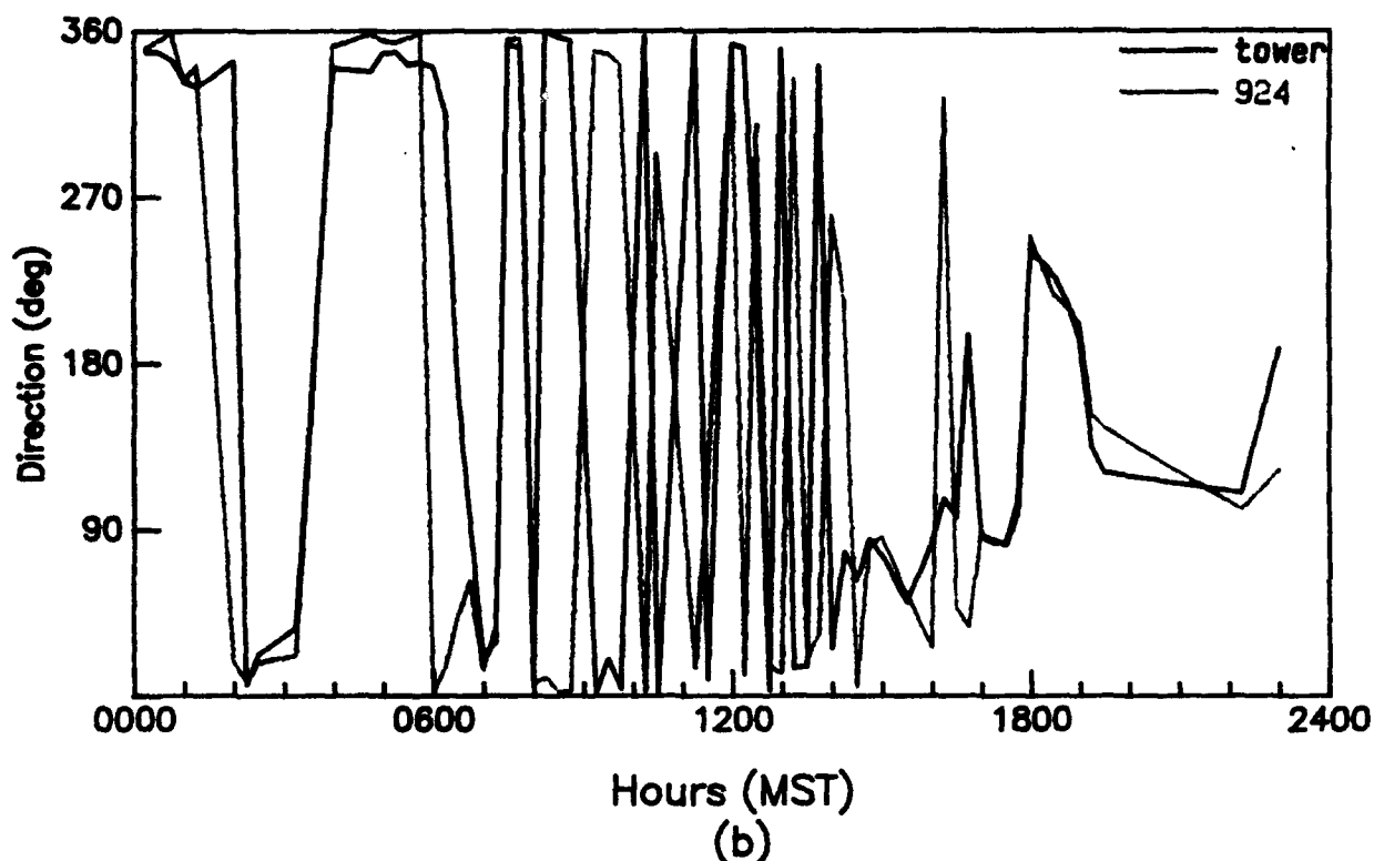
Figure 79. Diurnal variation of (a) wind speed and (b) wind direction as measured with a 924-MHz profiler at 120 m AGL (APRF site) and tower-mounted anemometers at 90, 120, and 150 m AGL (LC-35), WSMR, 0000 to 2400 MST, 25 August 1992 (15-min averages).
