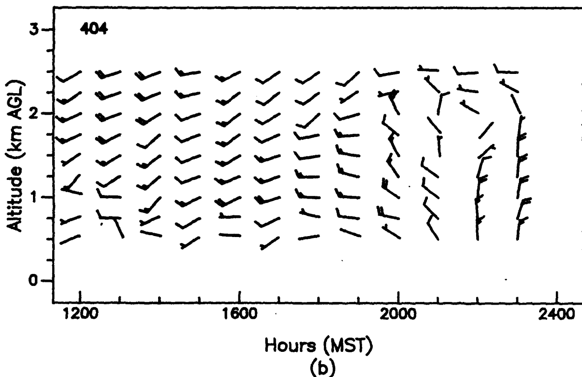
Figure 77. Vertical profiles of wind speed and wind direction, as measured with (a) a 924-MHz profiler and (b) a 404-MHz profiler, APRF site, WSMR, 1200 to 2400 MST, 24 August 1992 (1-h averages).
