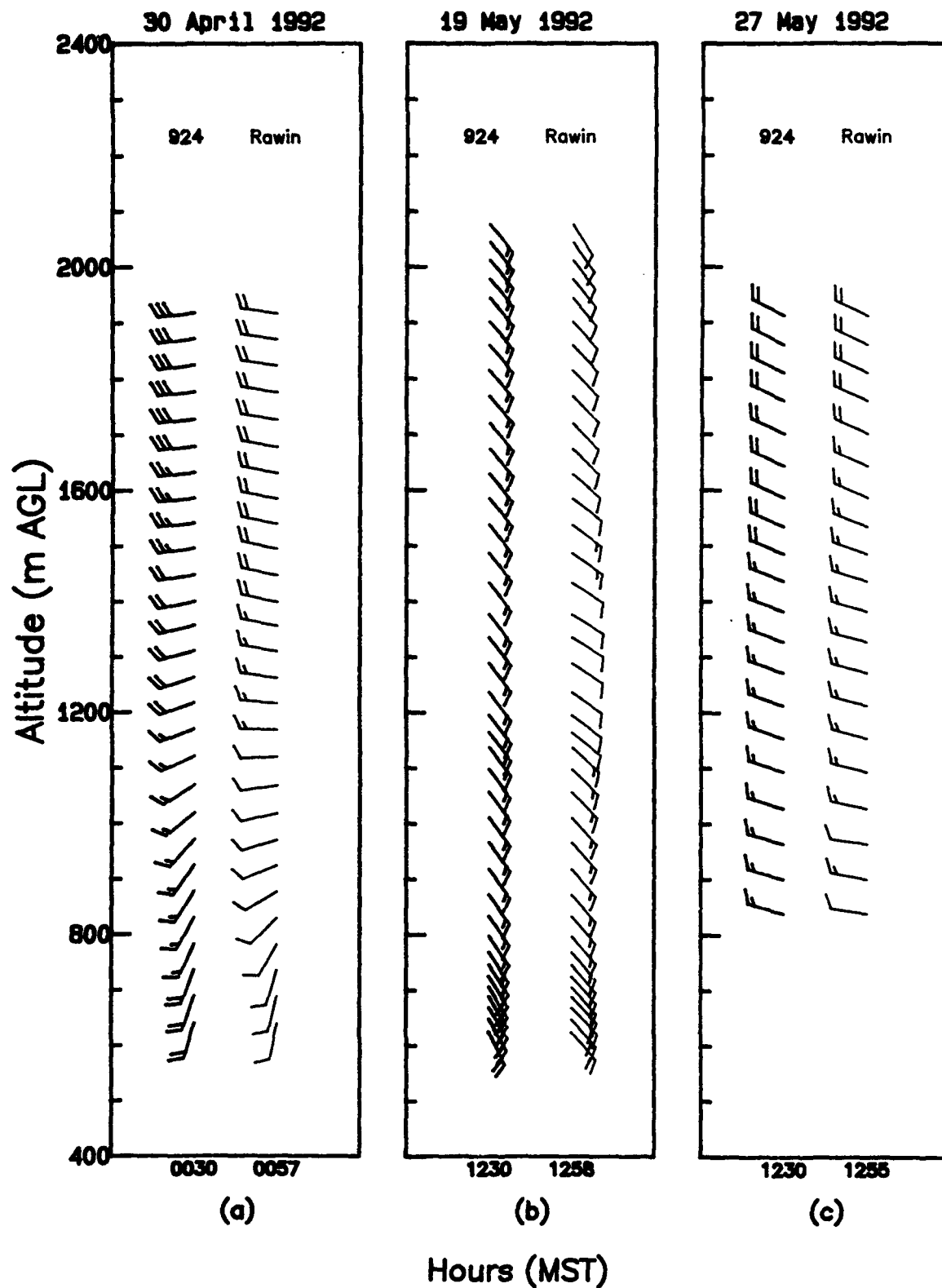
Figure 10. Comparison of volume-averaged wind profiles based on 924-MHz wind profiler and rawinsonde data during apparently uniform wind field conditions: (a) 30 April 1992, 0030-0100 MST, (b) 19 May 1992, 1230-1300 MST, and (c) 27 May 1992, 1230-1300 MST.
