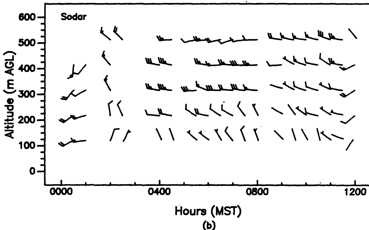
Figure 62. Vertical profiles of wind speed and wind direction, as measured with (a) a 924-MHz profiler and (b) a sodar, APRF site, WSMR, 0000 to 1200 MST, 20 August 1992 (15-min averages).
