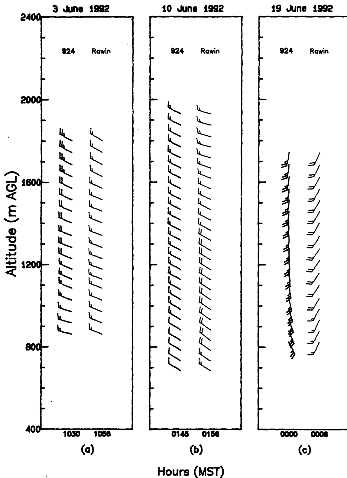
Figure 11. Comparison of volume-averaged wind profiles based on 924-MHz wind profiler and rawinsonde data during apparently uniform wind field conditions: (a) 3 June 1992, 1030-1100 MST, (b) 10 June 1992, 0145-0200 MST, and (c) 19 June 1992, 0000-0015 MST.
