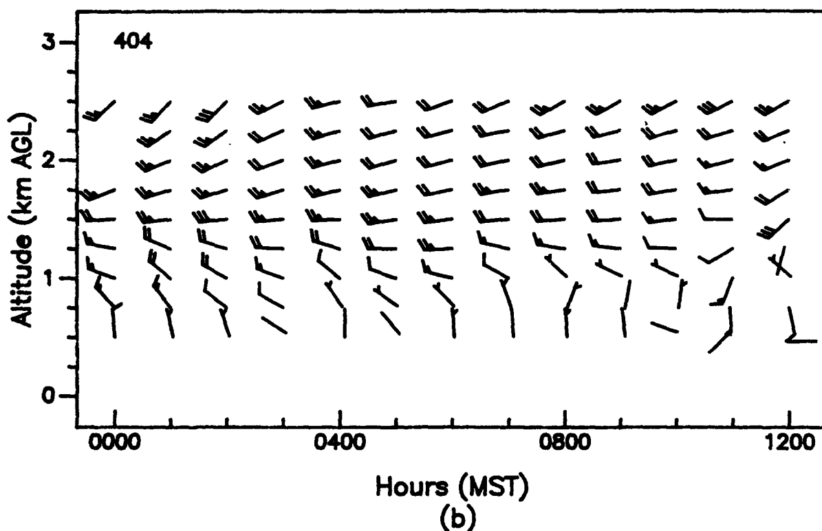
Figure 19. Vertical profiles of wind speed and wind direction, as measured with (a) a 924-MHz profiler and (b) a 404-MHz profiler, APRF site, WSMR, 0000 to 1200 MST, 17 June 1992 (1-h averages).
