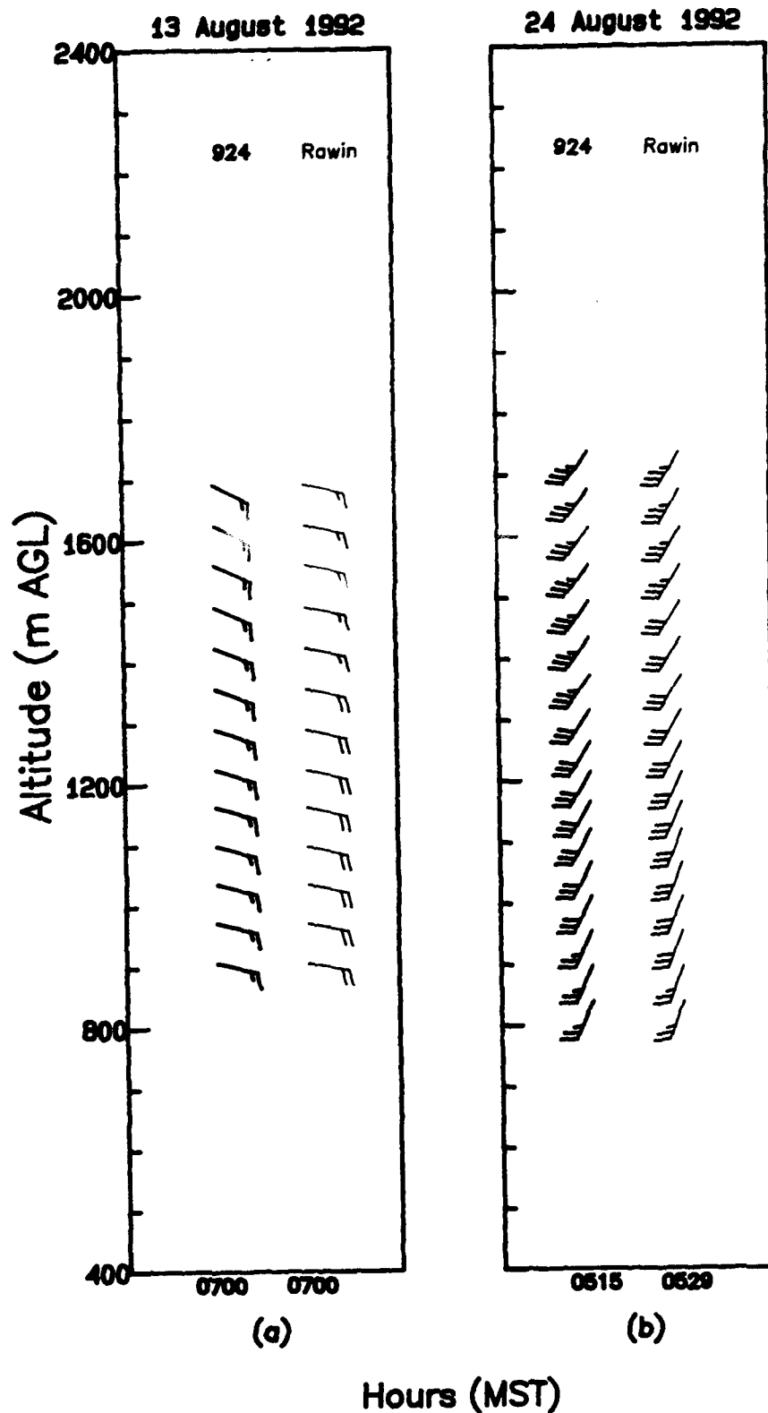
Figure 14. Comparison of volume-averaged wind profiles based on 924-MHz wind profiler and rawinsonde data during apparently uniform wind field conditions: (a) 13 August 1992, 0700-0715 MST, and (b) 24 August 1992, 0515-0530 MST.
