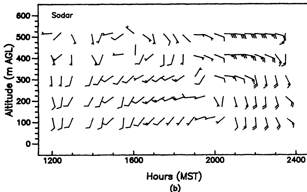
Figure 24. Vertical profiles of wind speed and wind direction, as measured with (a) a 924-MHz profiler and (b) a sodar, APRF site, WSMR, 1200 to 2400 MST, 18 June 1992 (15-min averages).
