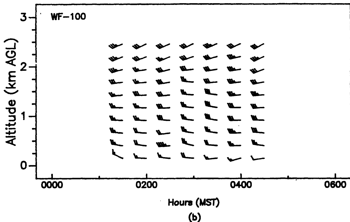
Figure 39. Vertical profiles of wind speed and wind direction, as measured with (a) a 924-MHz profiler at APRF site and (b) a WF-100 radar at Oasis site, WSMR, 0000 to 0600 MST, 1 July 1992 (15-min averages for the 924 data).
