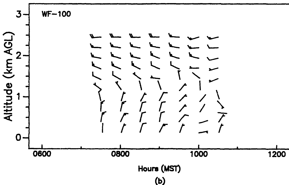
Figure 15. Vertical profiles of wind speed and wind direction, as measured with (a) a 924-MHz profiler at APRF site and (b) a WF-100 radar at Oasis site, WSMR, 0000 to 1200 MST, 17 June 1992 (15-min averages for the 924 data).
