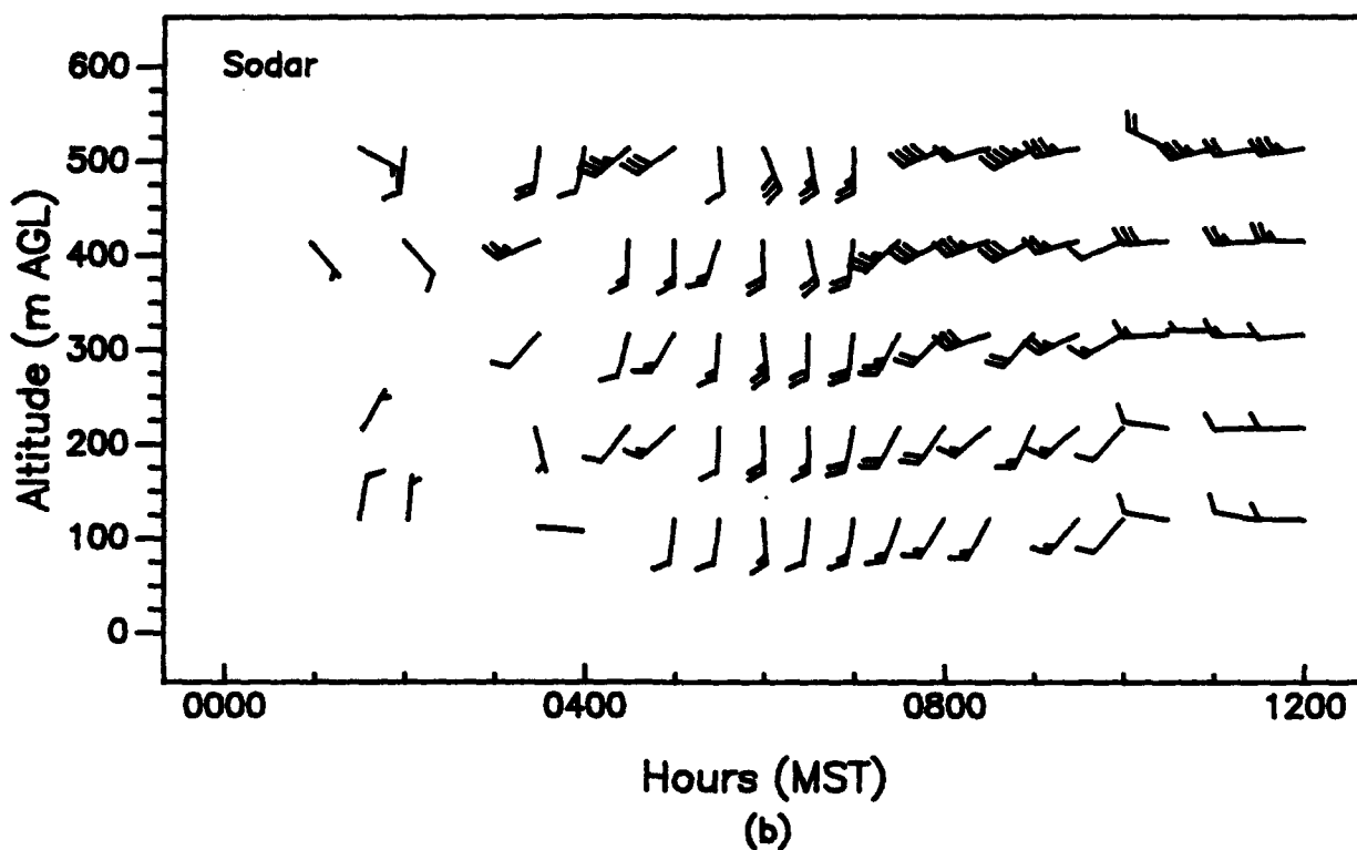
Figure 74. Vertical profiles of wind speed and wind direction, as measured with (a) a 924-MHz profiler and (b) a sodar, APRF site, WSMR, 0000 to 1200 MST, 24 August 1992 (15-min averages).
