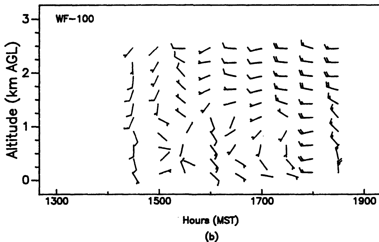
Figure 33. Vertical profiles of wind speed and wind direction, as measured with (a) a 924-MHz profiler at APRF site and (b) a WF-100 radar at Oasis site, WSMR, 1300 to 1900 MST, 25 June 1992 (15-min averages for the 924 data).
