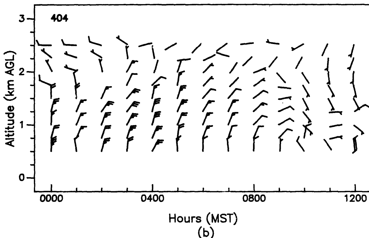
Figure 82. Vertical profiles of wind speed and wind direction, as measured with (a) a 924-MHz profiler and (b) a 404-MHz profiler, APRF site, WSMR, 0000 to 1200 MST, 25 August 1992 (1-h averages).
