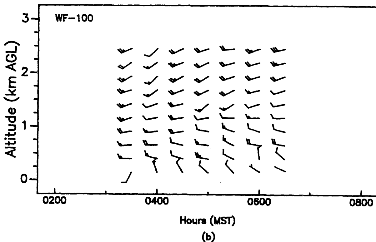
Figure 42. Vertical profiles of wind speed and wind direction, as measured with (a) a 924-MHz profiler at APRF site and (b) a WF-100 radar at Oasis site, WSMR, 0200 to 0800 MST, 2 July 1992 (15-min averages for the 924 data).
