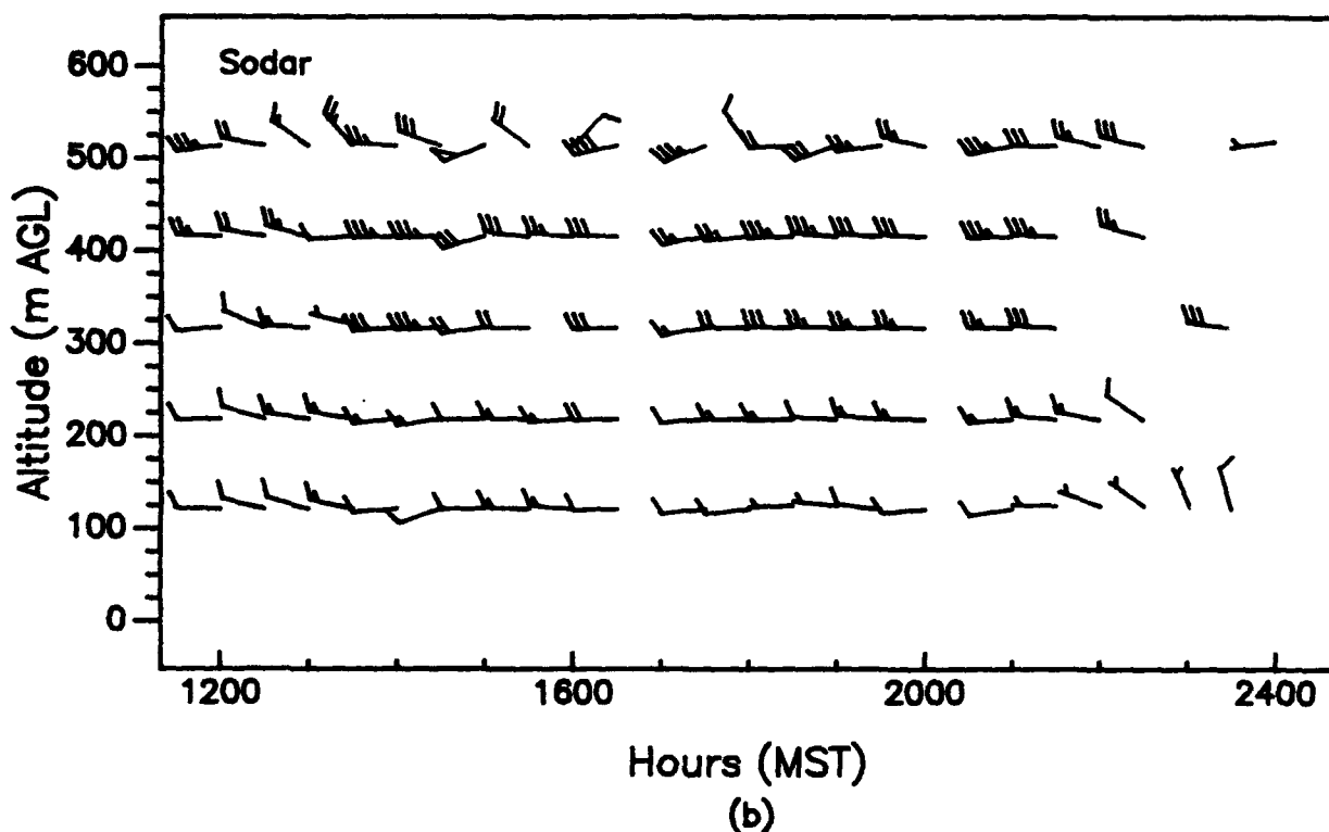
Figure 75. Vertical profiles of wind speed and wind direction, as measured with (a) a 924-MHz profiler and (b) a sodar, APRF site, WSMR, 1200 to 2400 MST, 24 August 1992 (15-min averages).
