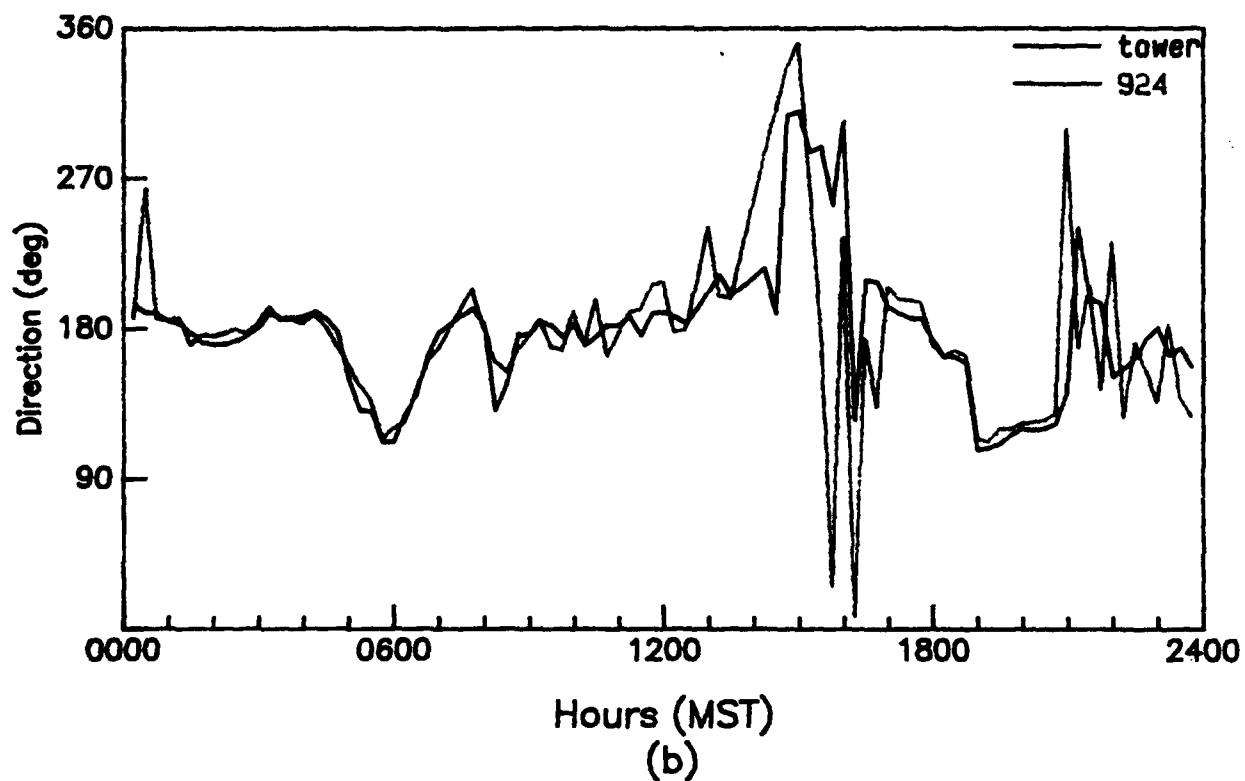
Figure 67. Diurnal variation of (a) wind speed and (b) wind direction as measured with a 924-MHz profiler at 120 m AGL (APRF site) and tower-mounted anemometers at 90, 120, and 150 m AGL (LC-35), WSMR, 0000 to 2400 MST, 21 August 1992 (15-min averages).
