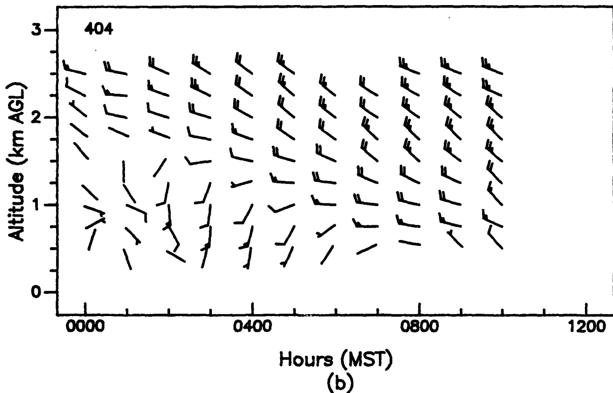
Figure 31. Vertical profiles of wind speed and wind direction, as measured with (a) a 924-MHz profiler and (b) a 404-MHz profiler, APRF site, WSMR, 0000 to 1200 MST, 24 June 1992 (1-h averages).
