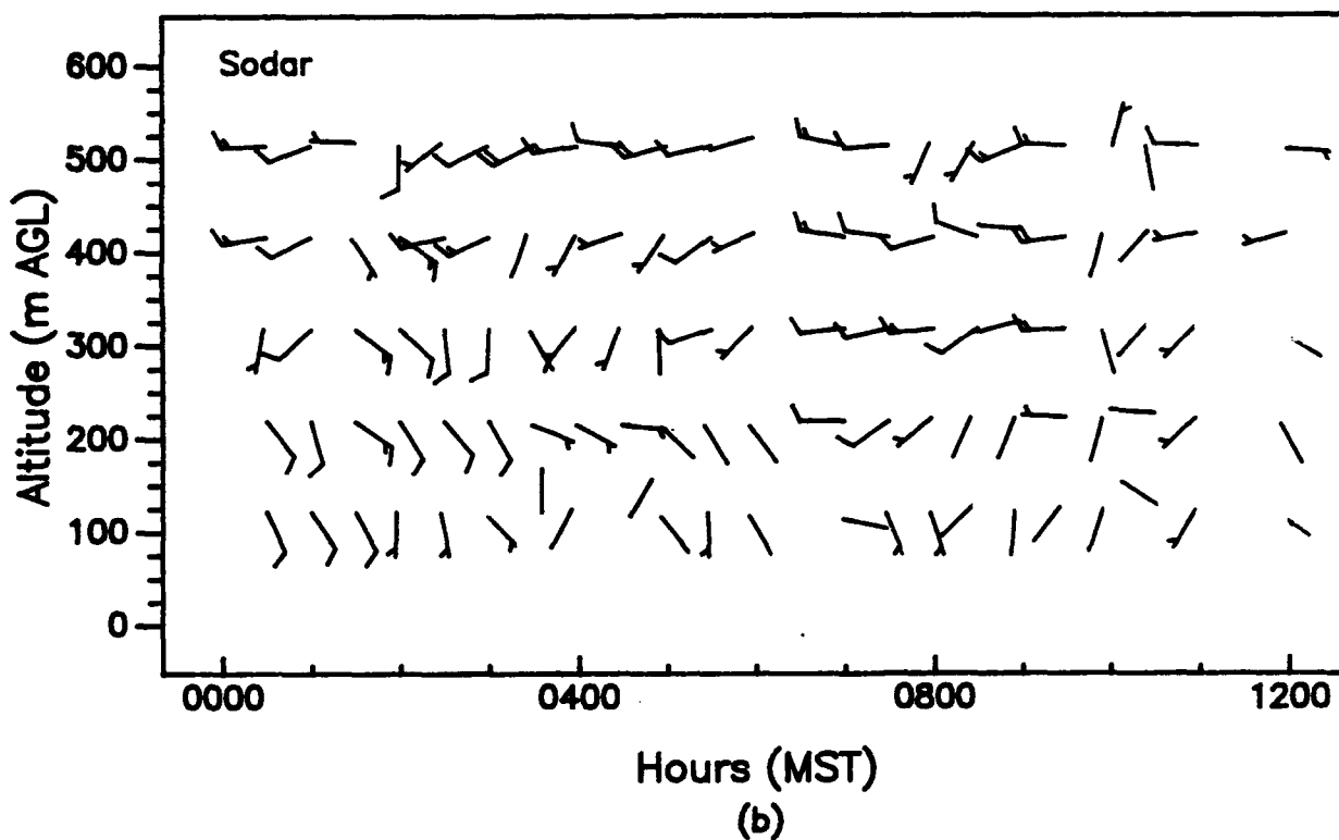
Figure 46. Vertical profiles of wind speed and wind direction, as measured with (a) a 924-MHz profiler and (b) a sodar, APRF site, WSMR, 0000 to 1200 MST, 8 July 1992 (15-min averages).
