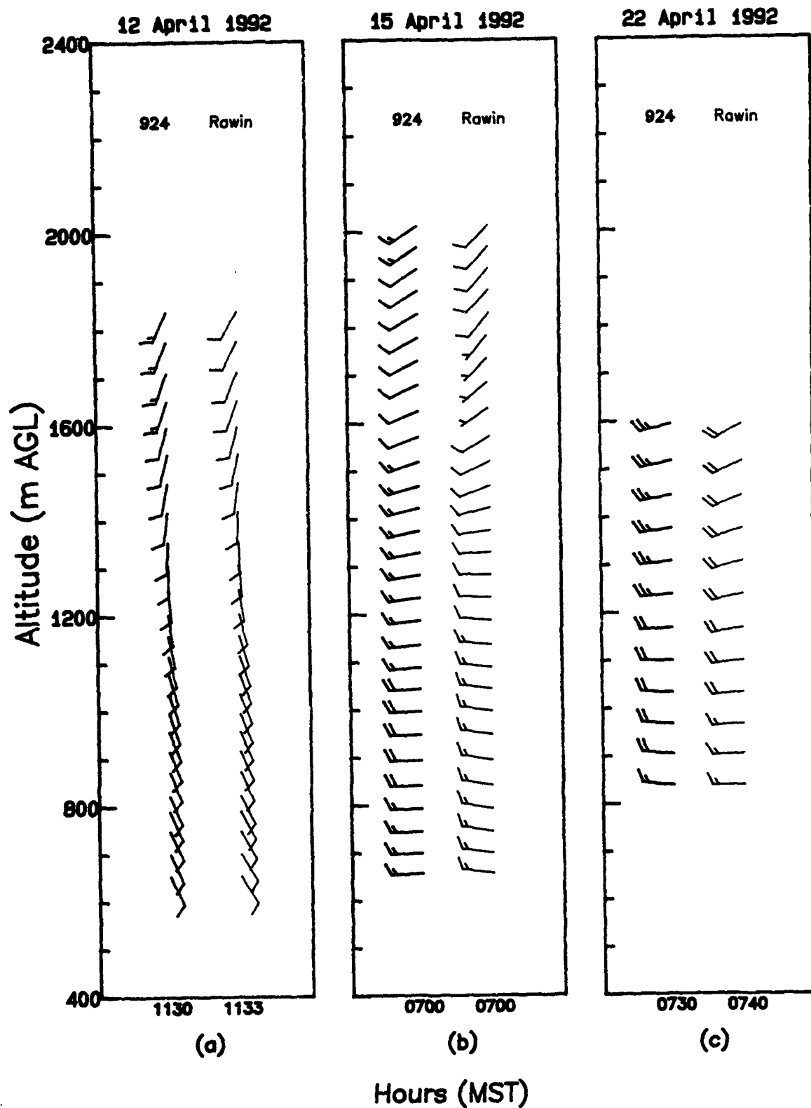
Figure 9. Comparison of volume-averaged wind profiles based on 924-MHz wind profiler and rawinsonde data during apparently uniform wind field conditions: (a) 12 April 1992, 1130-1200 MST, (b) 15 April 1992, 0700-0730 MST, and (c) 22 April 1992, 0730-0800 MST.
