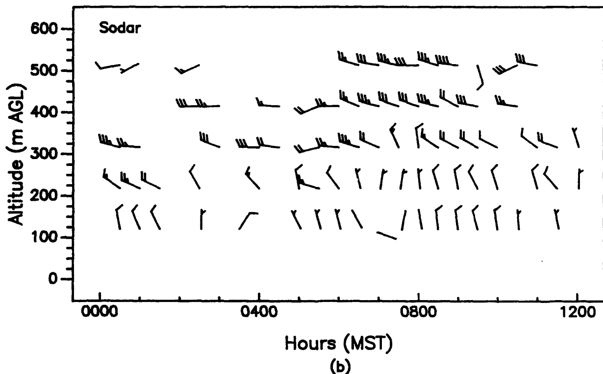
Figure 80. Vertical profiles of wind speed and wind direction, as measured with (a) a 924-MHz profiler and (b) a sodar, APRF site, WSMR, 0000 to 1200 MST, 25 August 1992 (15-min averages).
