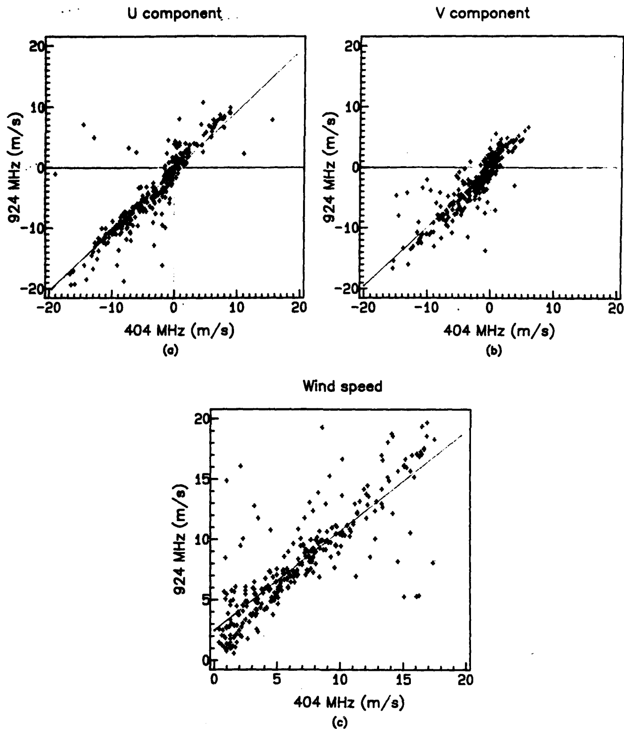
Figure E-4. Regression lines for (a) U component, (b) V component, and (c) resultant wind speed based on measurements with a 924-MHz wind profiler and a 404-MHz wind profiler, APRF site, WSMR, during 19 of 23 days of expected uniform wind fields listed in table 4 (60-min averages).
