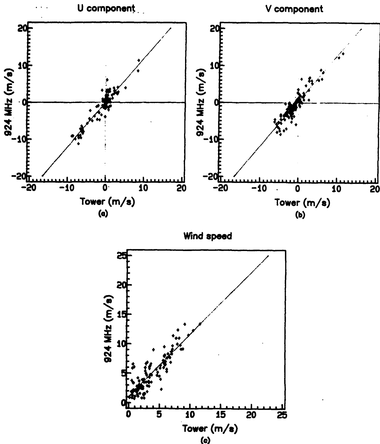
Figure E-1. Regression lines for (a) U component, (b) V component, and (c) resultant wind speed based on measurements with a 924-MHz wind profiler at 120 m AGL (APRF site) and tower-mounted anemometers at 90, 120, and 150 m AGL (LC-35), WSMR, during 9 of 14 WF-100 measurement periods listed in table 3 (15-min averages).
