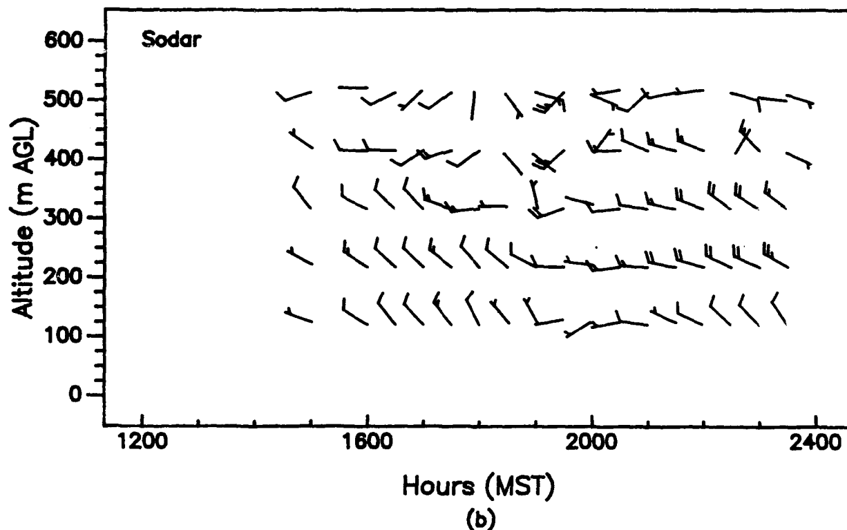
Figure 30. Vertical profiles of wind speed and wind direction, as measured with (a) a 924-MHz profiler and (b) a sodar, APRF site, WSMR, 1200 to 2400 MST, 24 June 1992 (15-min averages).
