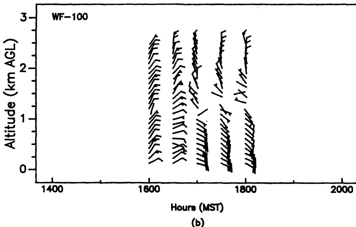
Figure 51. Vertical profiles of wind speed and wind direction, as measured with (a) a 924-MHz profiler at APRF site and (b) a WF-100 radar at Oasis site, WSMR, 1400 to 2000 MST, 18 August 1992 (15-min averages for the 924 data).
