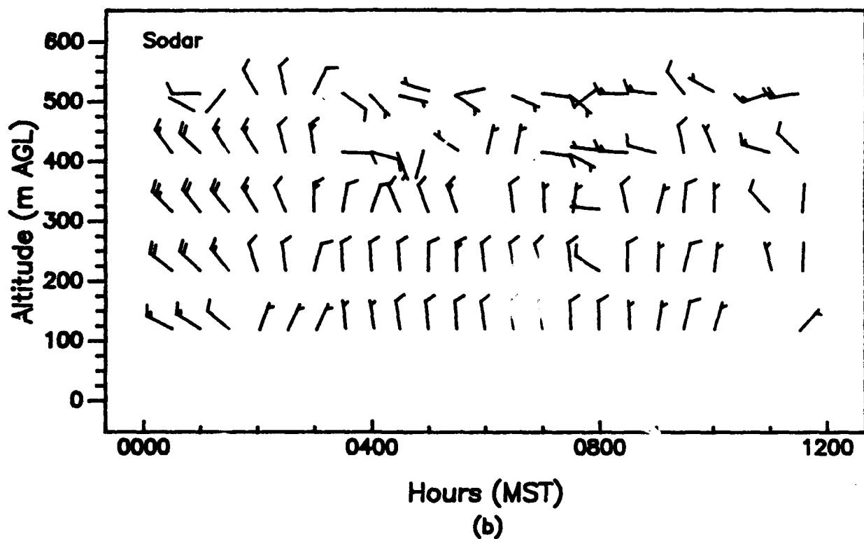
Figure 35. Vertical profiles of wind speed and wind direction, as measured with (a) a 924-MHz profiler and (b) a sodar, APRF site, WSMR, 0000 to 1200 MST, 25 June 1992 (15-min averages).
