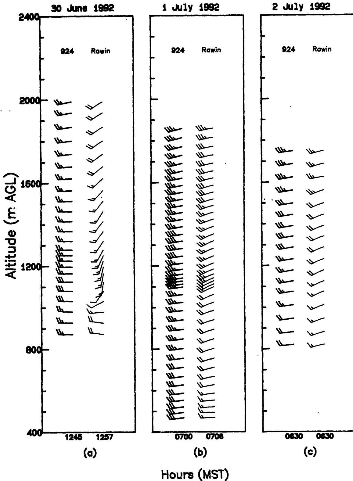
Figure 12. Comparison of volume-averaged wind profiles based on 924-MHz wind profiler and rawinsonde data during apparently uniform wind field conditions: (a) 30 June 1992, 1245-1300 MST, (b) 1 July 1992, 0700-0715 MST, and (c) 2 July 1992, 0630-0645 MST.
