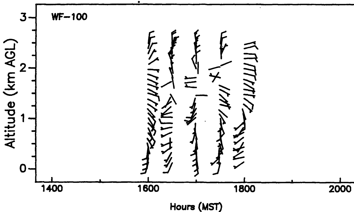
Figure 54. Vertical profiles of wind speed and wind direction, as measured with (a) a 924-MHz profiler at APRF site and (b) a WF-100 radar at Oasis site, WSMR, 1400 to 2000 MST, 19 August 1992 (15-min averages for the 924 data).
