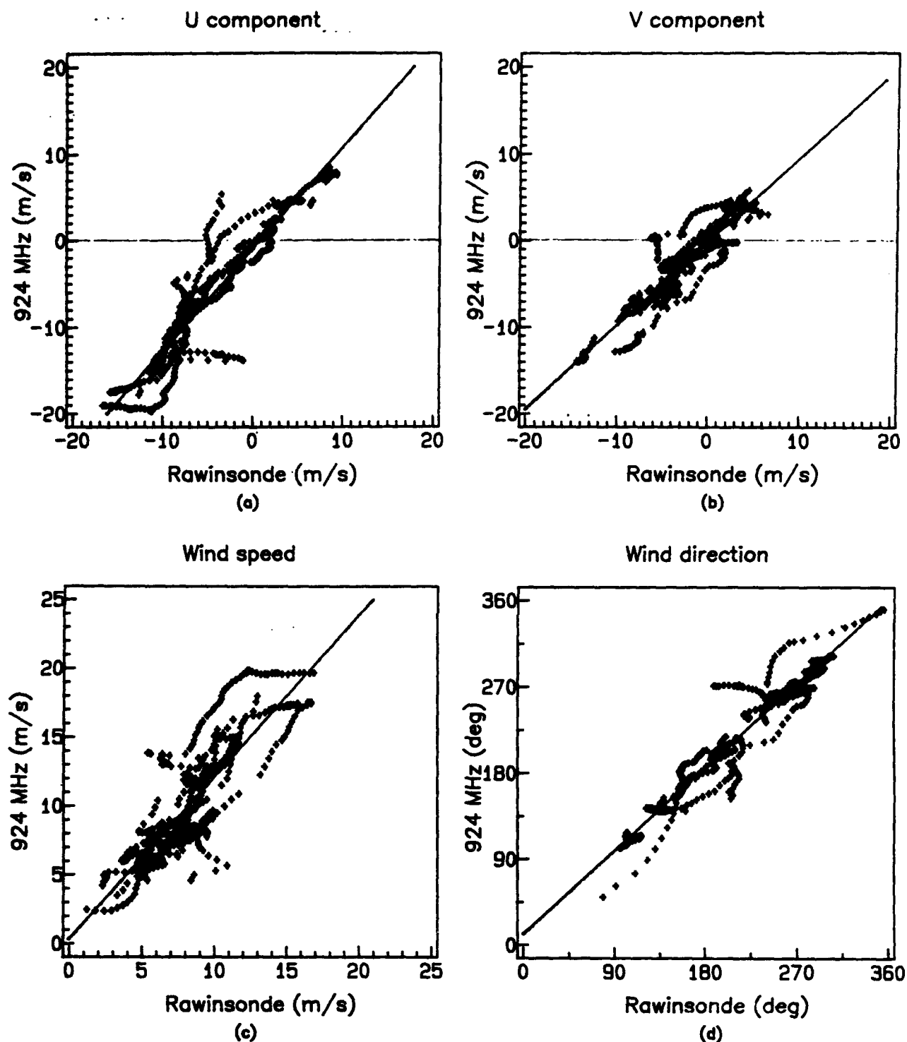
Figure E-3. Regression lines for (a) U component, (b) V component, (c) resultant wind speed, and (d) wind direction based on measurements with a 924-MHz wind profiler (APRF site) and rawinsondes (Oasis site), WSMR, during the 23 days of expected uniform wind fields listed in table 4 (30-min 924 averages before 5 June and 15-min averages after 5 June).
