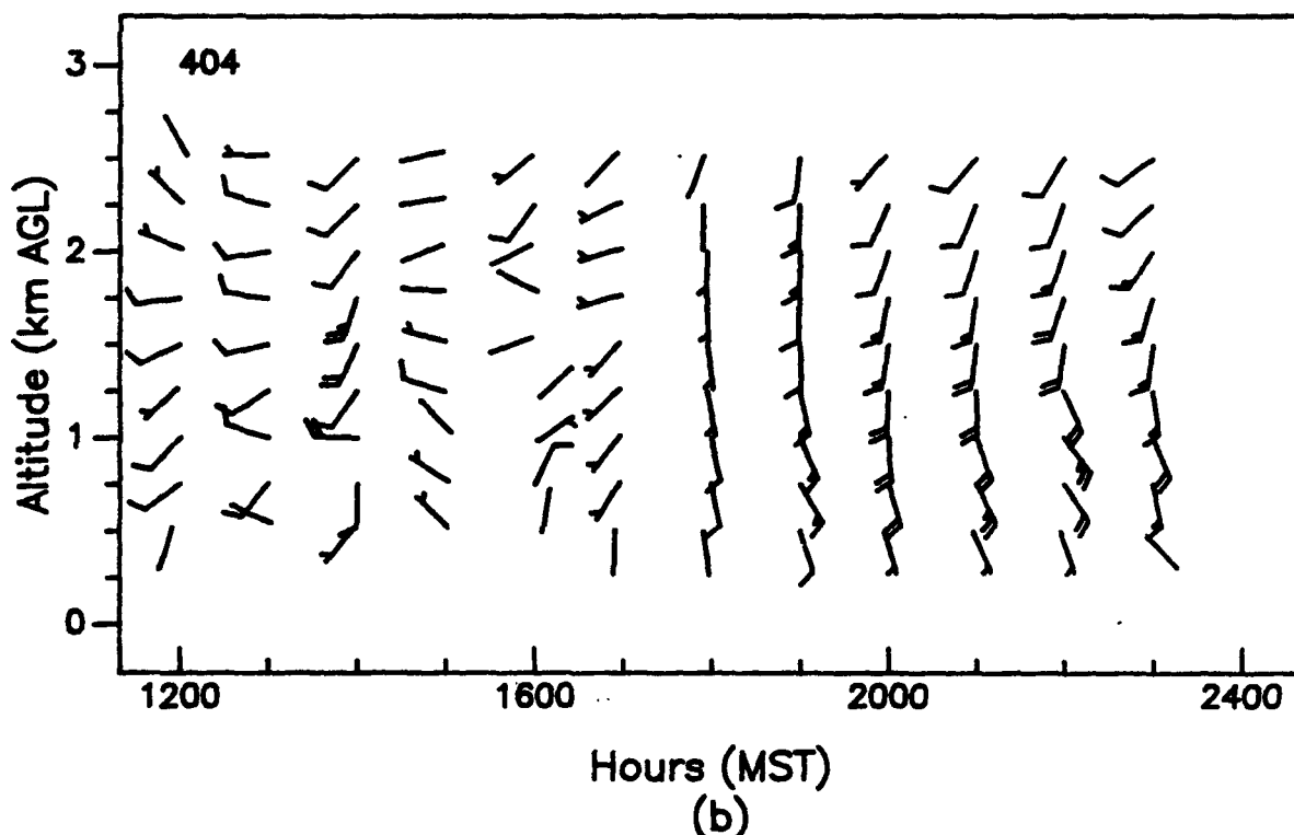
Figure 71. Vertical profiles of wind speed and wind direction, as measured with (a) a 924-MHz profiler and (b) a 404-MHz profiler, APRF site, WSMR, 1200 to 2400 MST, 21 August 1992 (1-h averages).
