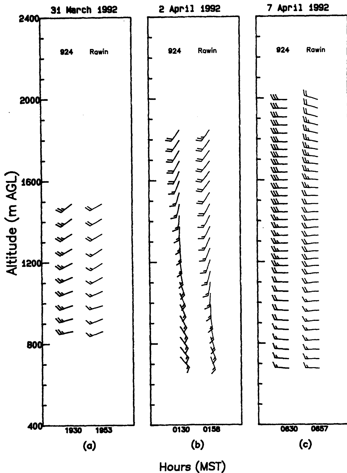
Figure 8. Comparison of volume-averaged wind profiles based on 924-MHz wind profiler and rawinsonde data during apparently uniform wind field conditions: (a) 31 March 1992, 1930-2000 MST, (b) 2 April 1992, 0130-0200 MST, and (c) 7 April 1992, 0630-0700 MST.
