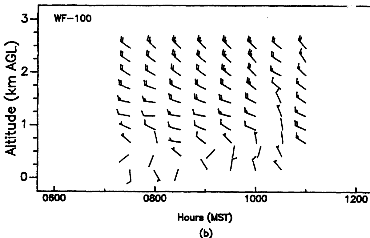
Figure 27. Vertical profiles of wind speed and wind direction, as measured with (a) a 924-MHz profiler at APRF site and (b) a WF-100 radar at Oasis site, WSMR, 0600 to 1200 MST, 24 June 1992 (15-min averages for the 924 data).
