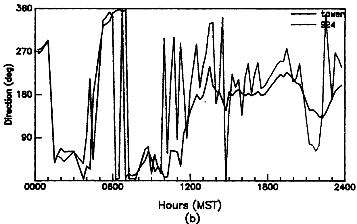
Figure 61. Diurnal variation of (a) wind speed and (b) wind direction as measured with a 924-MHz profiler at 120 m AGL (APRF site) and tower-mounted anemometers at 90, 120, and 150 m AGL (LC-35), WSMR, 0000 to 2400 MST, 20 August 1992 (15-min averages).
