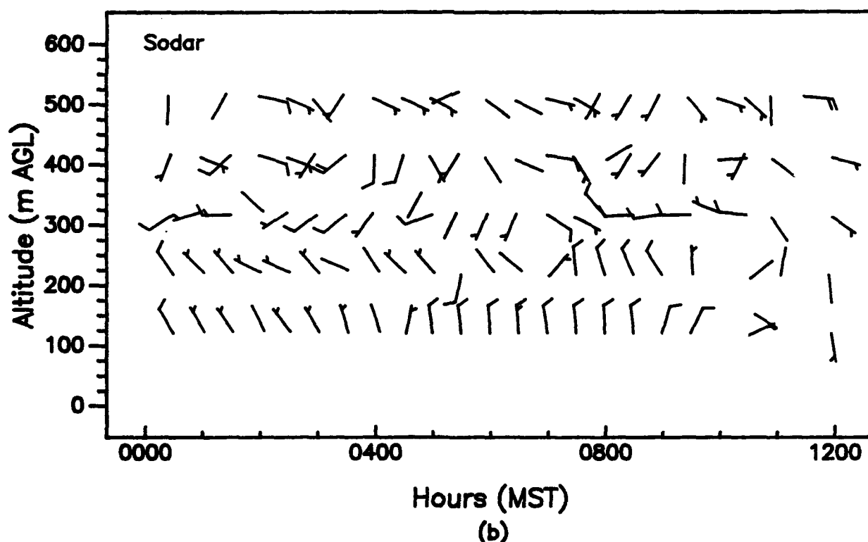
Figure 17. Vertical profiles of wind speed and wind direction, as measured with (a) a 924-MHz profiler and (b) a sodar, APRF site, WSMR, 0000 to 1200 MST, 17 June 1992 (15-min averages).
