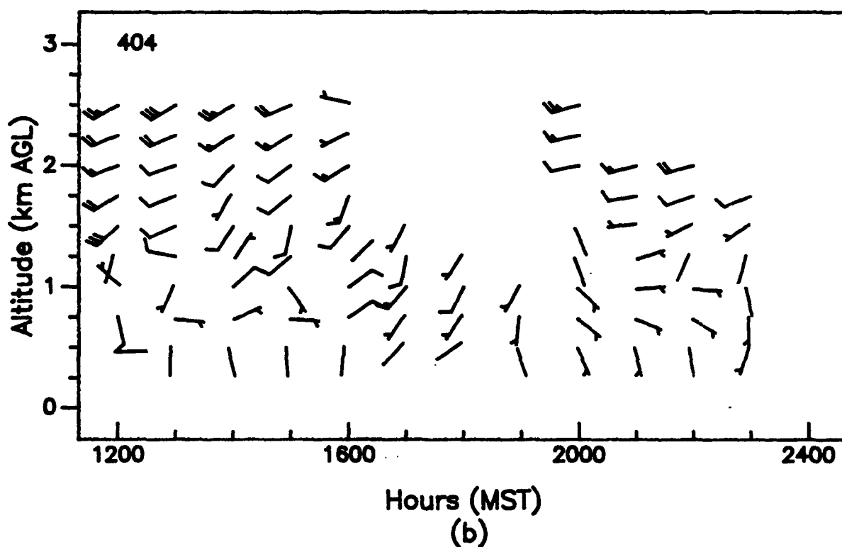
Figure 20. Vertical profiles of wind speed and wind direction, as measured with (a) a 924-MHz profiler and (b) a 404-MHz profiler, APRF site, WSMR, 1200 to 2400 MST, 17 June 1992 (1-h averages).
