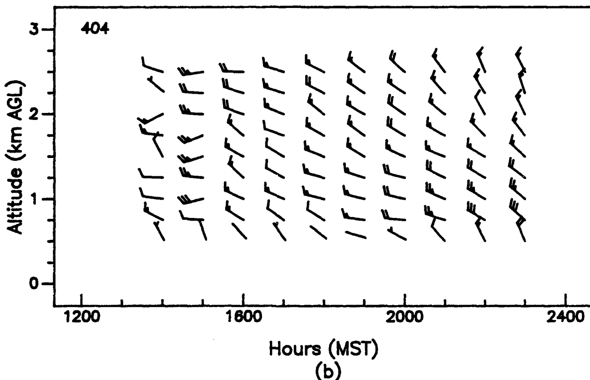
Figure 32. Vertical profiles of wind speed and wind direction, as measured with (a) a 924-MHz profiler and (b) a 404-MHz profiler, APRF site, WSMR, 1200 to 2400 MST, 24 June 1992 (1-h averages).
