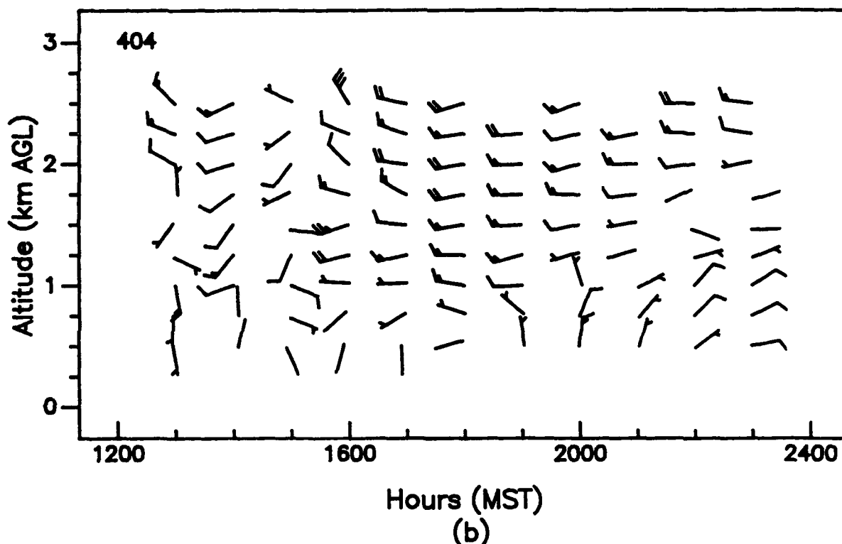
Figure 38. Vertical profiles of wind speed and wind direction, as measured with (a) a 924-MHz profiler and (b) a 404-MHz profiler, APRF site, WSMR, 1200 to 2400 MST, 25 June 1992 (1-h averages).
