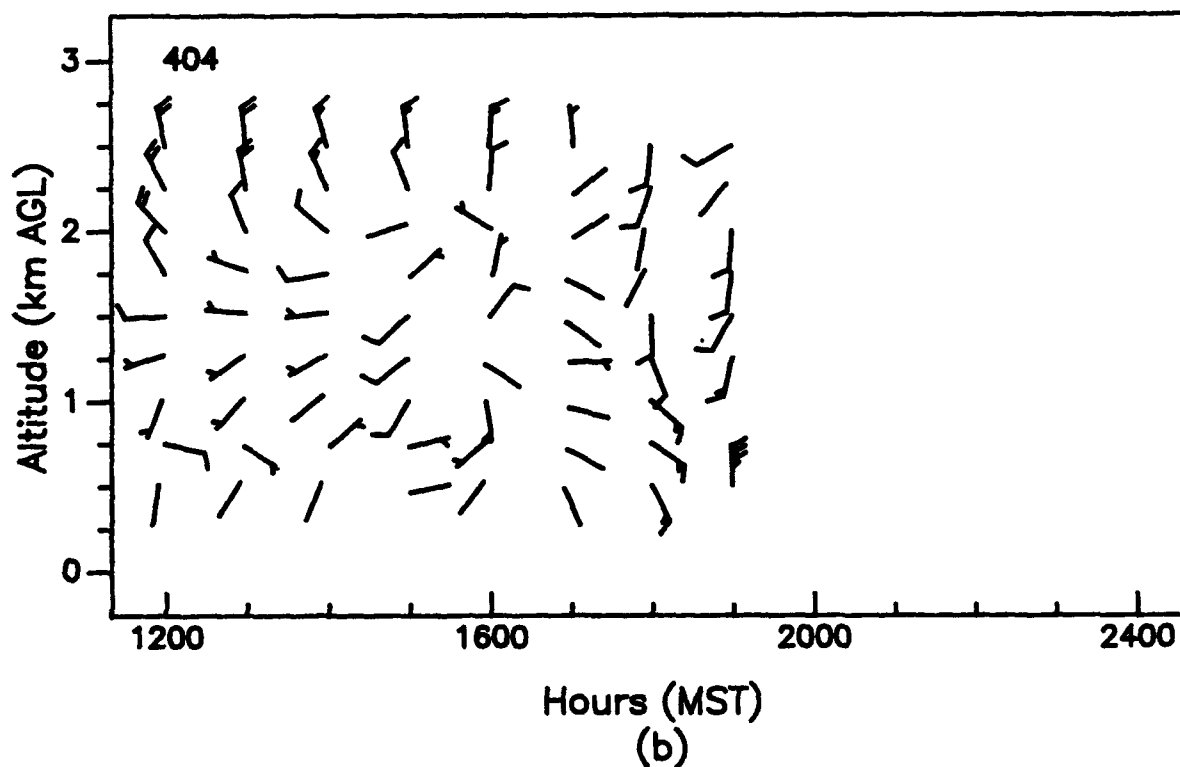
Figure 59. Vertical profiles of wind speed and wind direction, as measured with (a) a 924-MHz profiler and (b) a 404-MHz profiler, APRF site, WSMR, 1200 to 2400 MST, 19 August 1992 (1-h averages).
