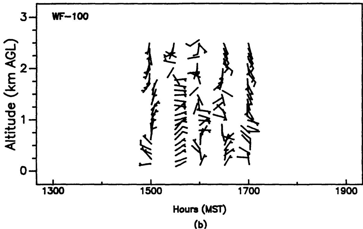
Figure 78. Vertical profiles of wind speed and wind direction, as measured with (a) a 924-MHz profiler at APRF site and (b) a WF-100 radar at Oasis site, WSMR, 1300 to 1900 MST, 25 August 1992 (15-min averages for the 924 data).
