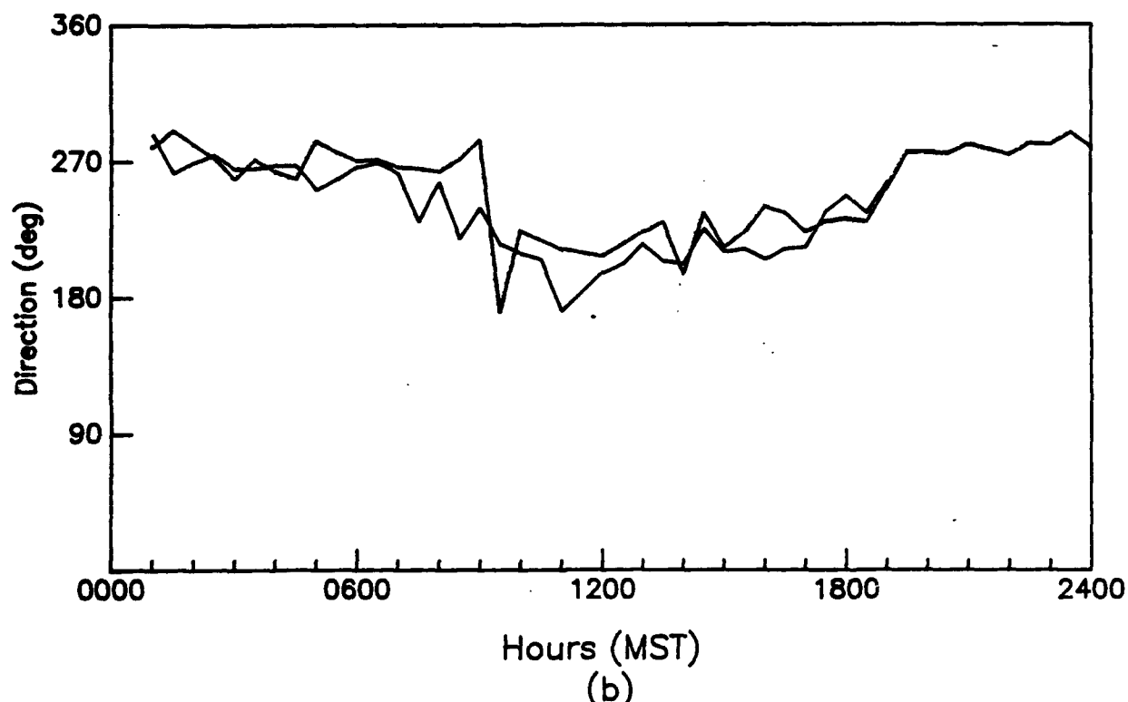
Figure 90. Diurnal variation of (a) wind speed and (b) wind direction as measured with a 924-MHz profiler at 514 m AGL and a sodar at 475 and 500 m AGL, APRF site, WSMR, 0000 to 2400 MST, 15 April 1992 (30-min averages).
