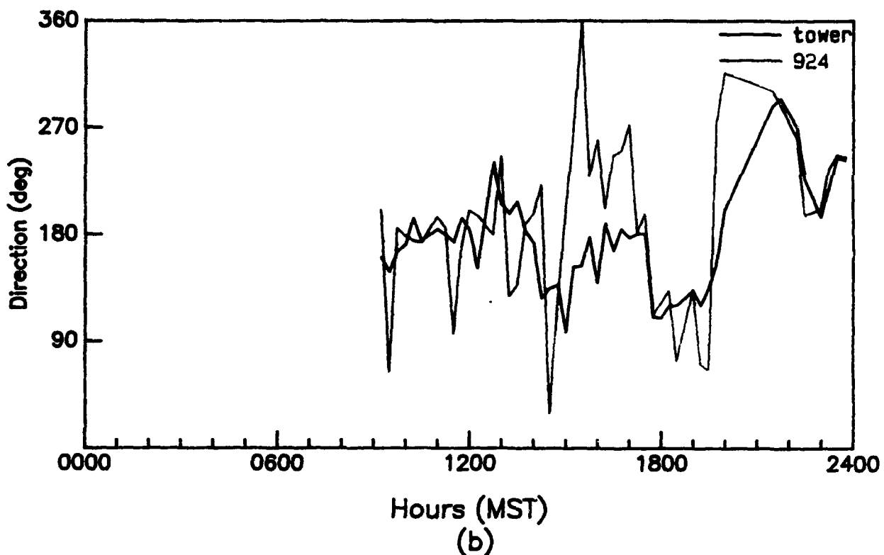
Figure 55. Diurnal variation of (a) wind speed and (b) wind direction as measured with a 924-MHz profiler at 120 m AGL (APRF site) and tower-mounted anemometers at 90, 120, and 150 m AGL (LC-35), WSMR, 0000 to 2400 MST, 19 August 1992 (15-min averages).
