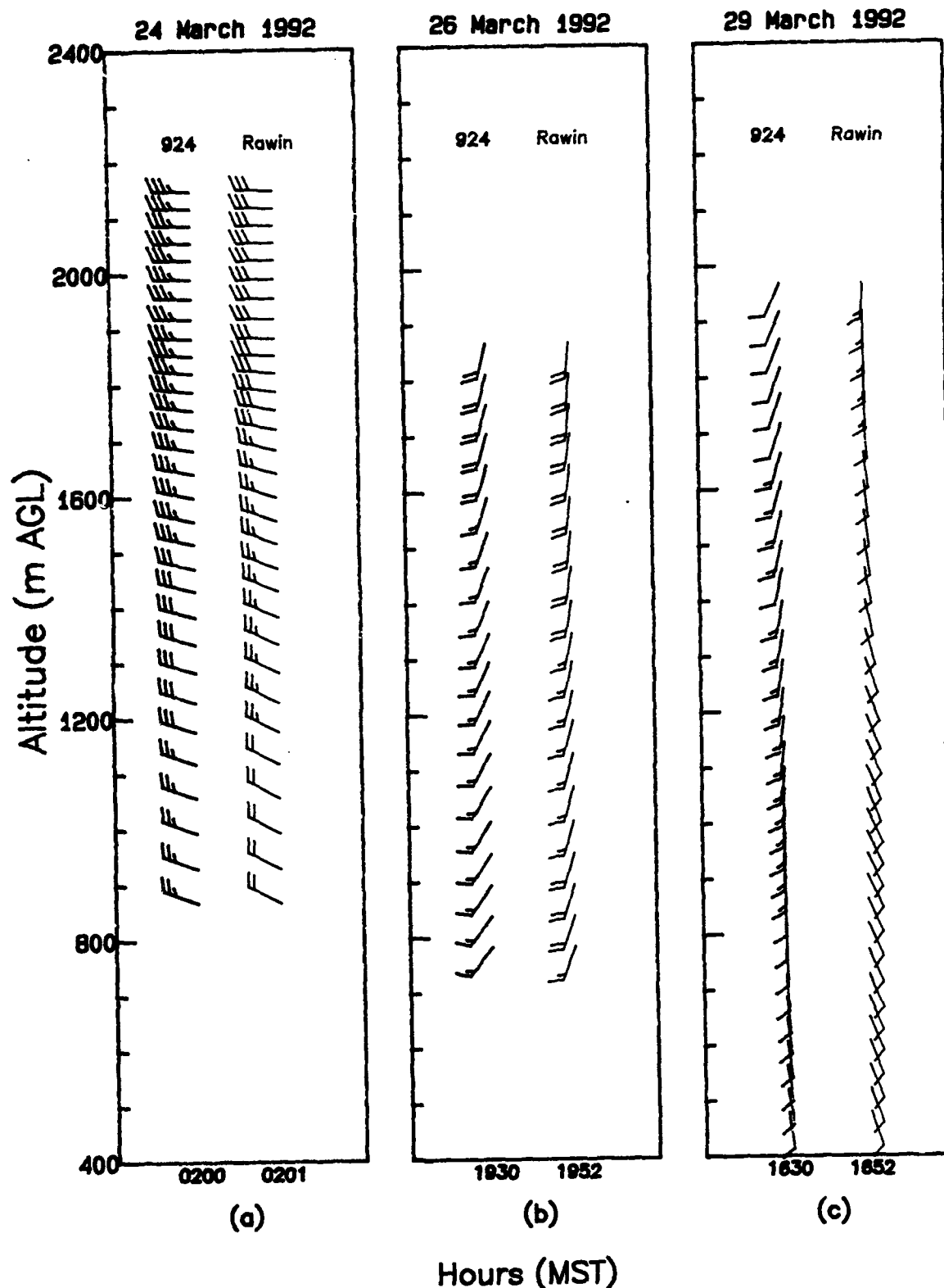
Figure 7. Comparison of volume-averaged wind profiles based on 924-MHz wind profiler and rawinsonde data during apparently uniform wind field conditions: (a) 24 March 1992, 0200-0230 MST, (b) 26 March 1992, 1930-2000 MST, and (c) 29 March 1992, 1630-1700 MST.
