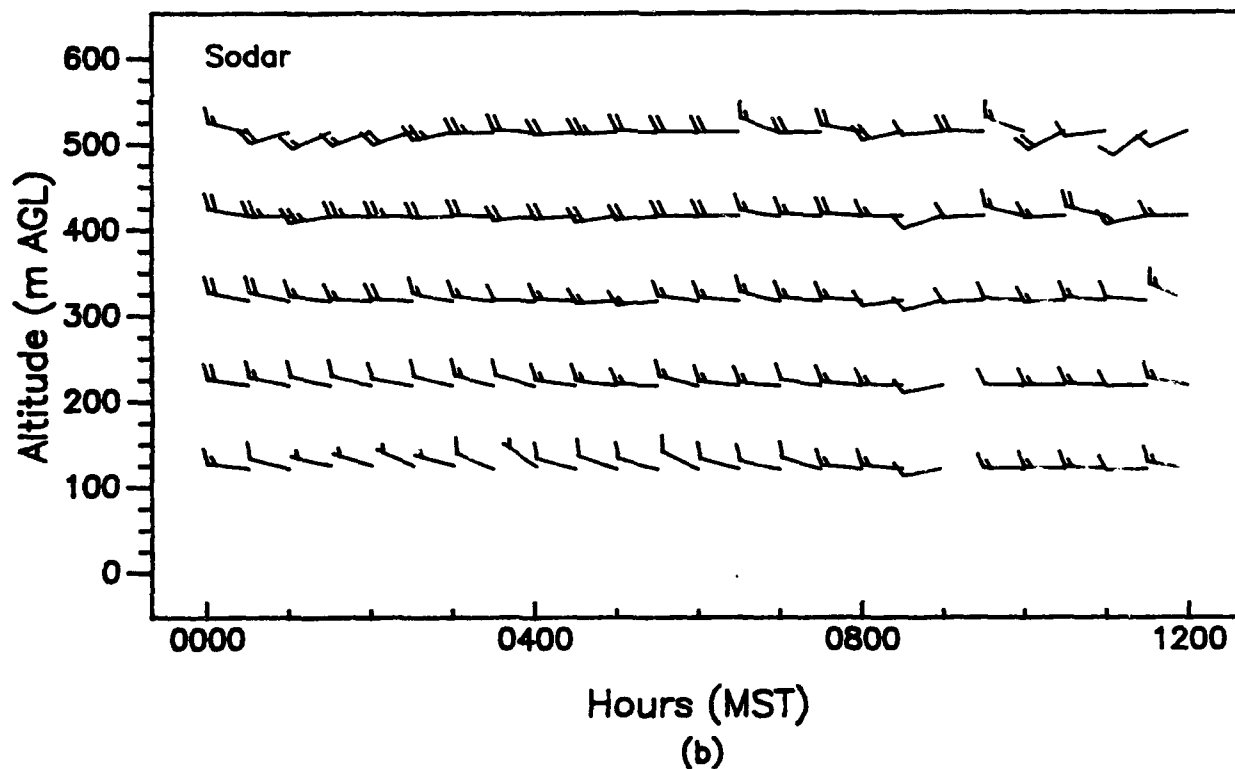
Figure 43. Vertical profiles of wind speed and wind direction, as measured with (a) a 924-MHz profiler and (b) a sodar, APRF site, WSMR, 0000 to 1200 MST, 2 July 1992 (15-min averages).
