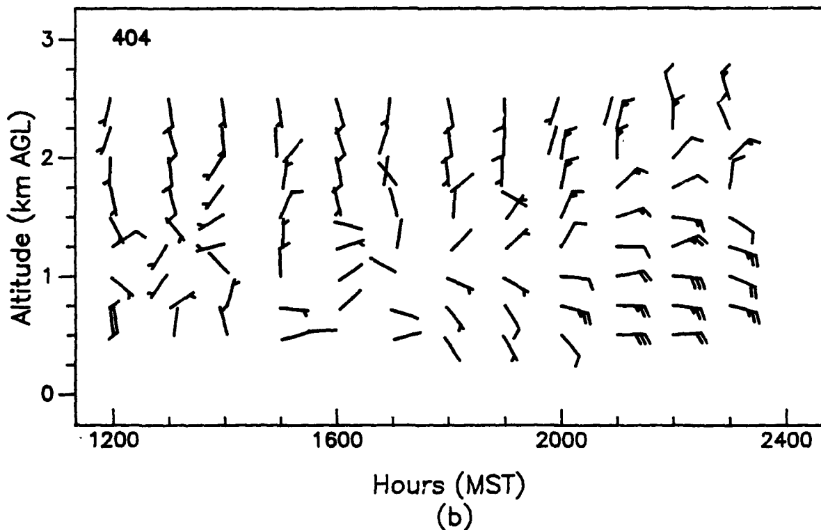
Figure 83. Vertical profiles of wind speed and wind direction, as measured with (a) a 924-MHz profiler and (b) a 404-MHz profiler, APRF site, WSMR, 1200 to 2400 MST, 25 August 1992 (1-h averages).
