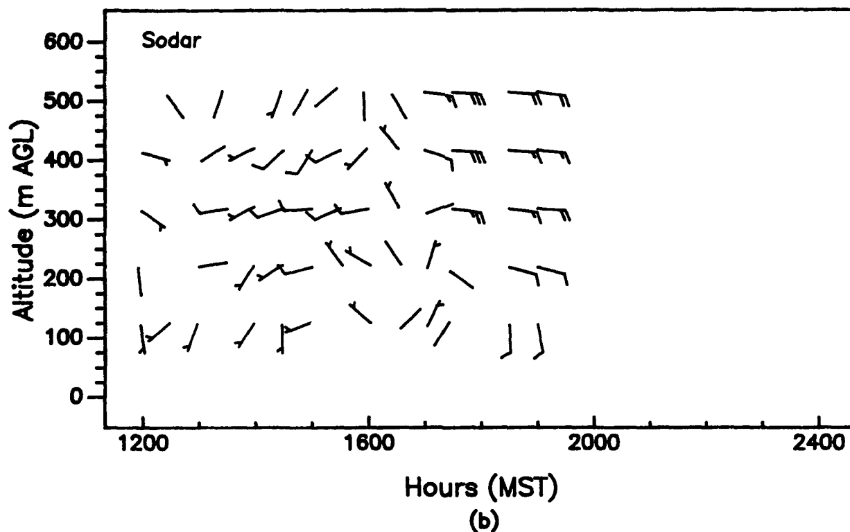
Figure 18. Vertical profiles of wind speed and wind direction, as measured with (a) a 924-MHz profiler and (b) a sodar, APRF site, WSMR, 1200 to 2400 MST, 17 June 1992 (15-min averages).
