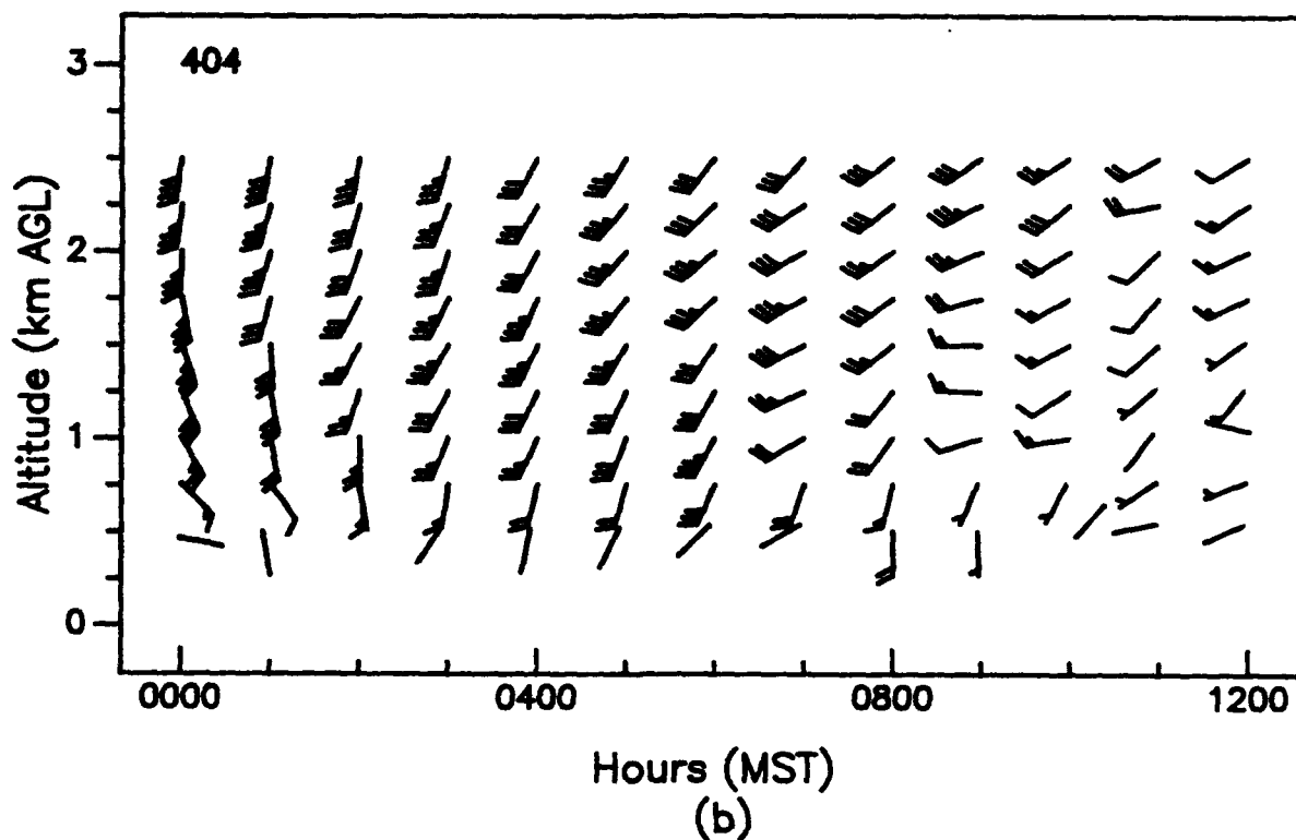
Figure 76. Vertical profiles of wind speed and wind direction, as measured with (a) a 924-MHz profiler and (b) a 404-MHz profiler, APRF site, WSMR, 0000 to 1200 MST, 24 August 1992 (1-h averages).
