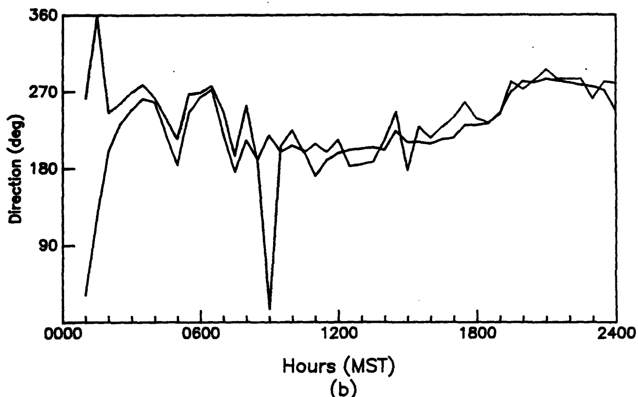
Figure 86. Diurnal variation of (a) wind speed and (b) wind direction as measured with a 924-MHz profiler at 120 m AGL and a sodar at 75, 100, 125, and 150 m AGL, APRF site, WSMR, 0000 to 2400 MST, 15 April 1992 (30-min averages).
