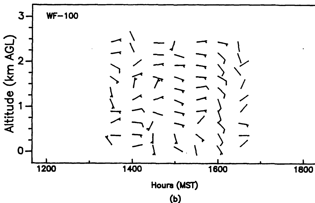
Figure 45. Vertical profiles of wind speed and wind direction, as measured with (a) a 924-MHz profiler at APRF site and (b) a WF-100 radar at Oasis site, WSMR, 1200 to 1800 MST, 8 July 1992 (15-min averages for the 924 data).
