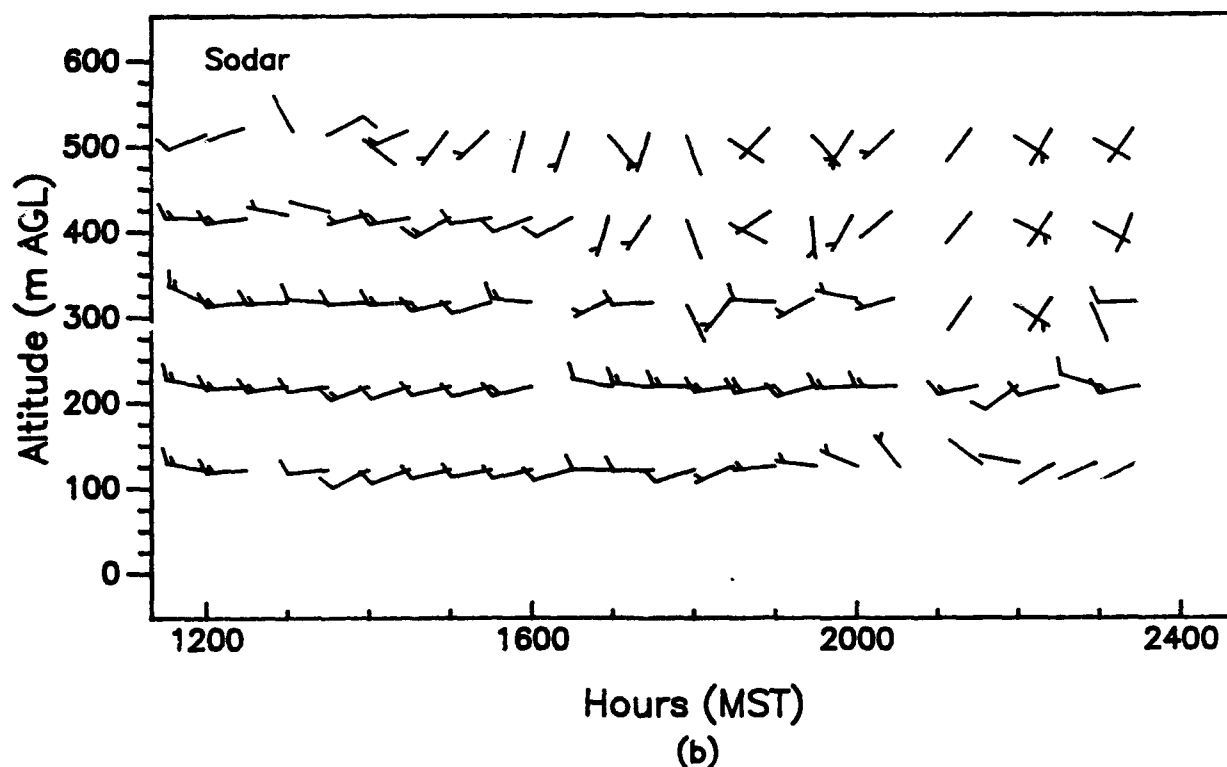
Figure 44. Vertical profiles of wind speed and wind direction, as measured with (a) a 924-MHz profiler and (b) a sodar, APRF site, WSMR, 1200 to 2400 MST, 2 July 1992 (15-min averages).
