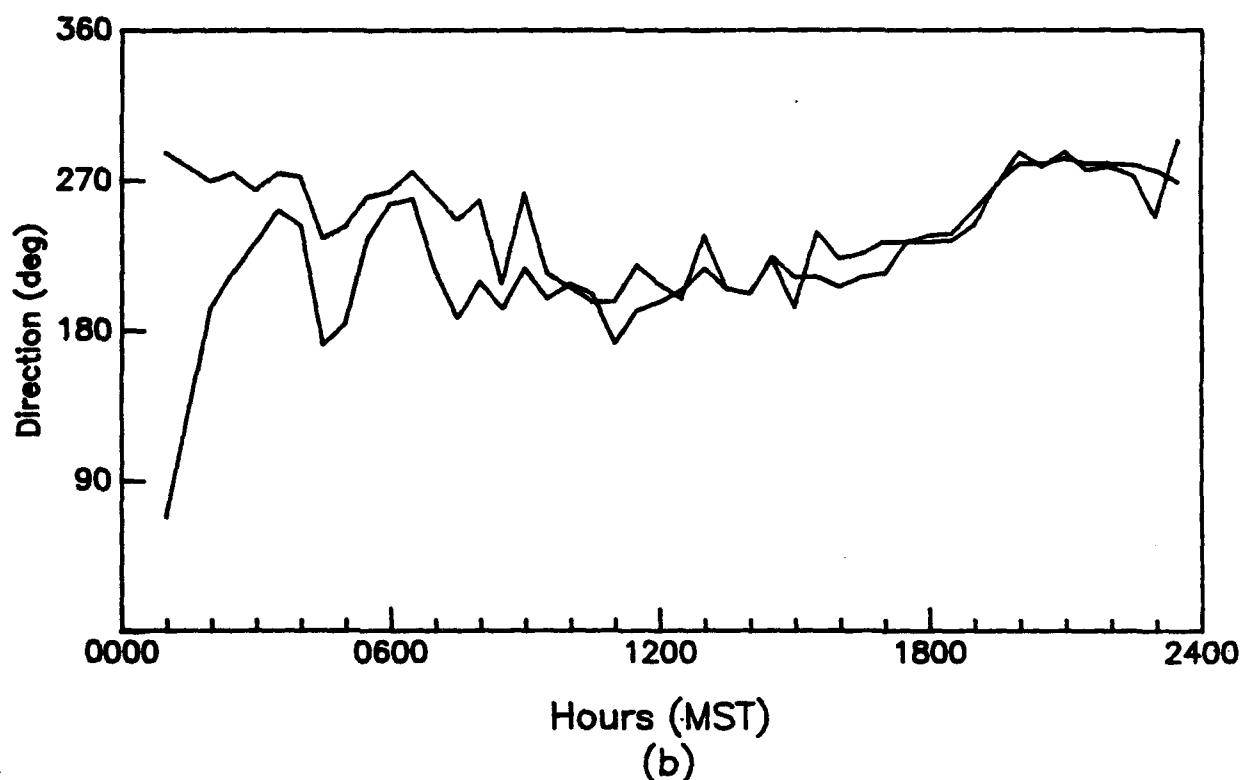
Figure 88. Diurnal variation of (a) wind speed and (b) wind direction as measured with a 924-MHz profiler at 317 m AGL and a sodar at 275, 300, 325, and 350 m AGL, APRF site, WSMR, 0000 to 2400 MST, 15 April 1992 (30-min averages).
