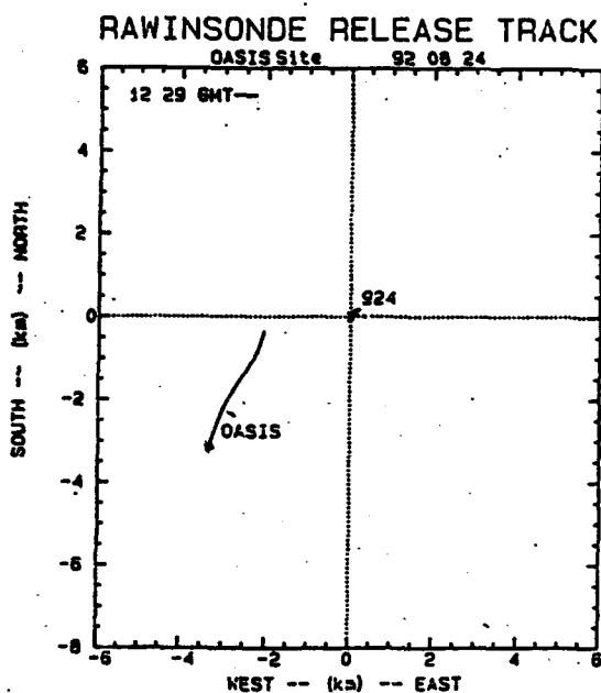
Figure 6. Horizontal projection of the trajectory of rawinsondes released from Oasis during the spring and summer of 1992: (a) 24 March, 0201 MST, (b) 19 May, 1258 MST, (c) 24 August, 0529 MST, and (d) composite of all 23 rawinsondes (924 = APRF complex).
