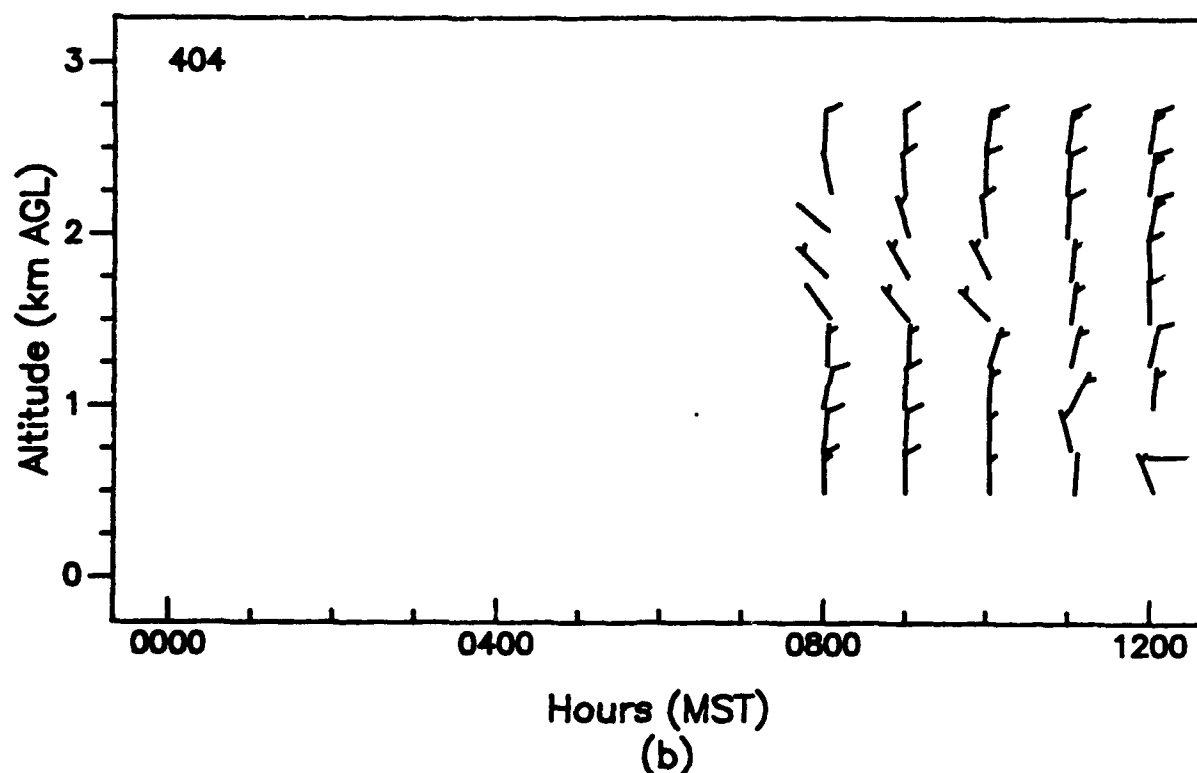
Figure 52. Vertical profiles of wind speed and wind direction, as measured with (a) a 924-MHz profiler and (b) a 404-MHz profiler, APRF site, WSMR, 0000 to 1200 MST, 18 August 1992 (1-h averages).
