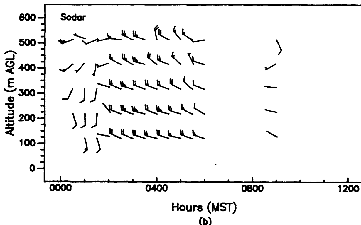
Figure 49. Vertical profiles of wind speed and wind direction, as measured with (a) a 924-MHz profiler and (b) a sodar, APRI site, WSMR, 0000 to 1200 MST, 9 July 1992 (15-min averages).
