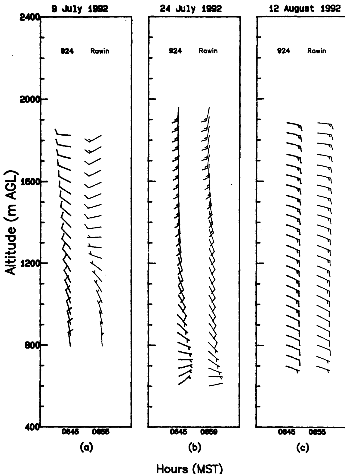
Figure 13. Comparison of volume-averaged wind profiles based on 924-MHz wind profiler and rawinsonde data during apparently uniform wind field conditions: (a) 9 July 1992, 0645-0700 MST, (b) 24 July 1992, 0645-0700 MST, and (c) 12 August 1992, 0645-0700 MST.
