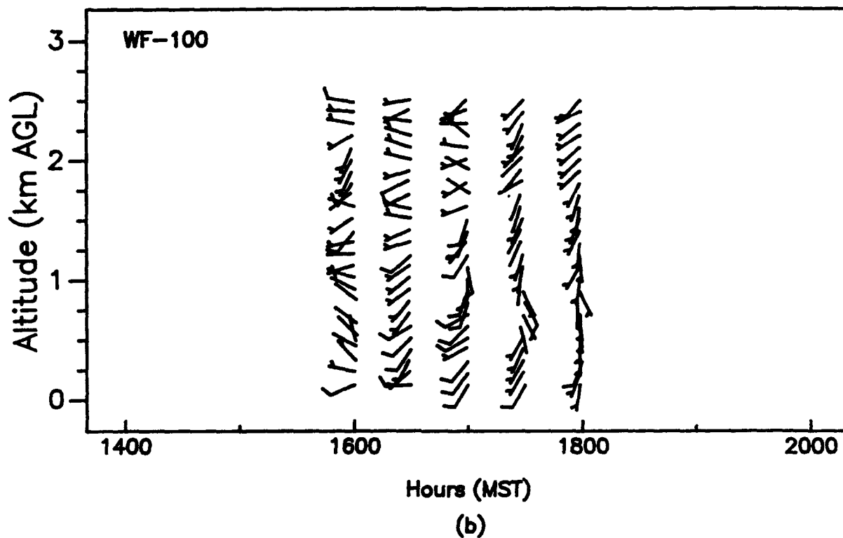
Figure 66. Vertical profiles of wind speed and wind direction, as measured with (a) a 924-MHz profiler at APRF site and (b) a WF-100 radar at Oasis site, WSMR, 1400 to 2000 MST, 21 August 1992 (15-min averages for the 924 data).
