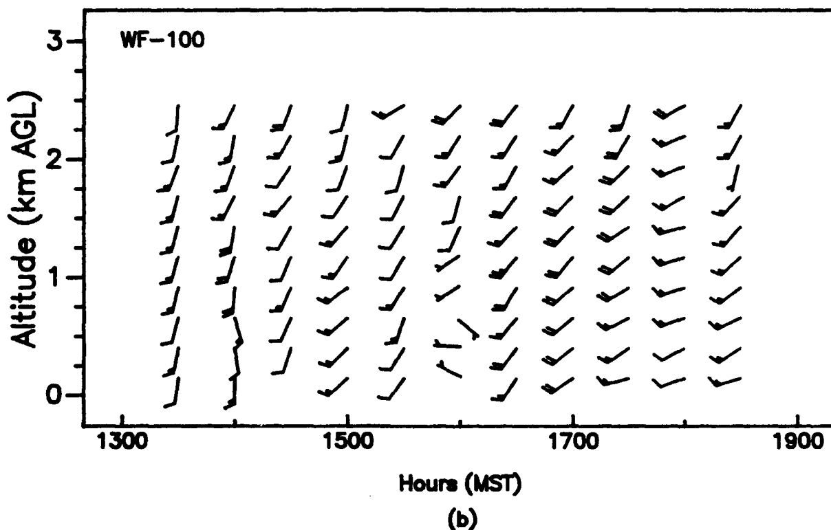
Figure 21. Vertical profiles of wind speed and wind direction, as measured with (a) a 924-MHz profiler at APRF site and (b) a WF-100 radar at Oasis site, WSMR, 1300 to 1900 MST, 18 June 1992 (15-min averages for the 924 data).
