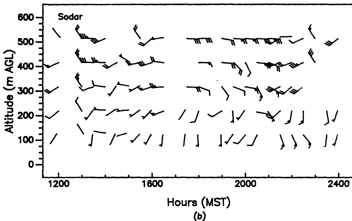
Figure 63. Vertical profiles of wind speed and wind direction, as measured with (a) a 924-MHz profiler and (b) a sodar, APRF site, WSMR, 1200 to 2400 MST, 20 August 1992 (15-min averages).
