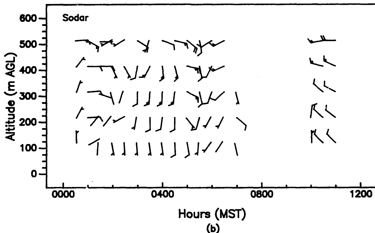
Figure 29. Vertical profiles of wind speed and wind direction, as measured with (a) a 924-MHz profiler and (b) a sodar, APRF site, WSMR, 0000 to 1200 MST, 24 June 1992 (15-min averages).
