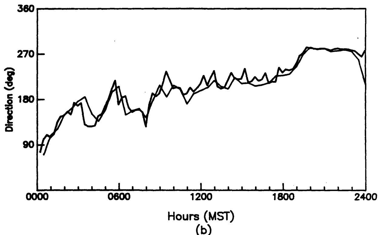
Figure 85. Diurnal variation of (a) wind speed and (b) wind direction as measured with tower-mounted anemometers at 40 and 50 m AGL (LC-35) and a sodar at 50 m AGL (APRF site), WSMR, 0000 to 2400 MST, 15 April 1992 (30-min averages).
