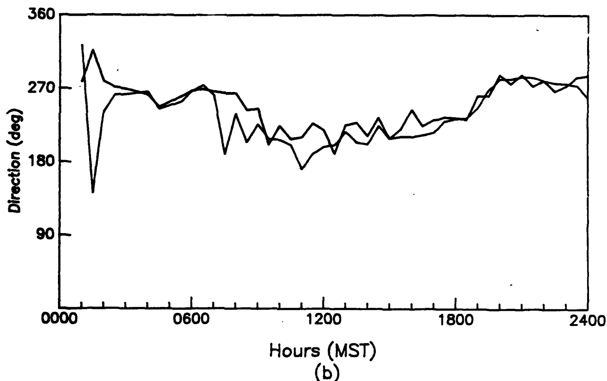
Figure 89. Diurnal variation of (a) wind speed and (b) wind direction as measured with a 924-MHz profiler at 416 m AGL and a sodar at 375, 400, 425, and 450 m AGL, APRF site, WSMR, 0000 to 2400 MST, 15 April 1992 (30-min averages).
