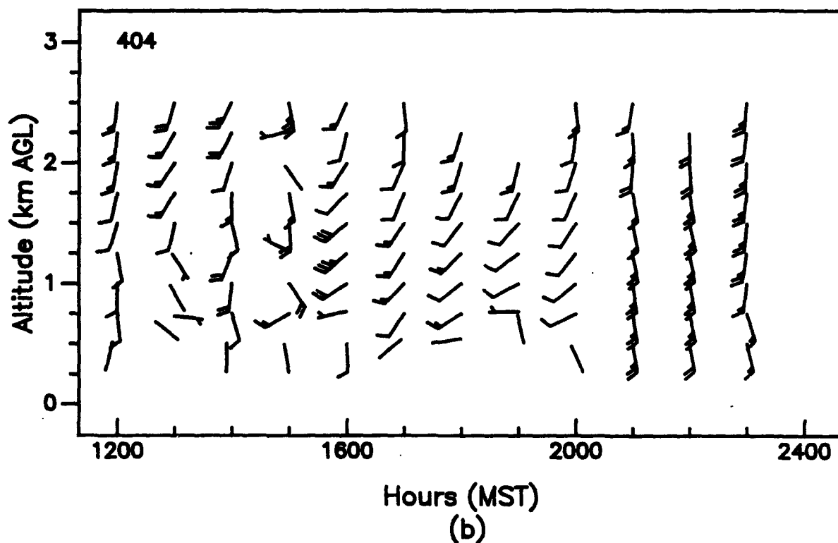
Figure 26. Vertical profiles of wind speed and wind direction, as measured with (a) a 924-MHz profiler and (b) a 404-MHz profiler, APRF site, WSMR, 1200 to 2400 MST, 18 June 1992 (1-h averages).
