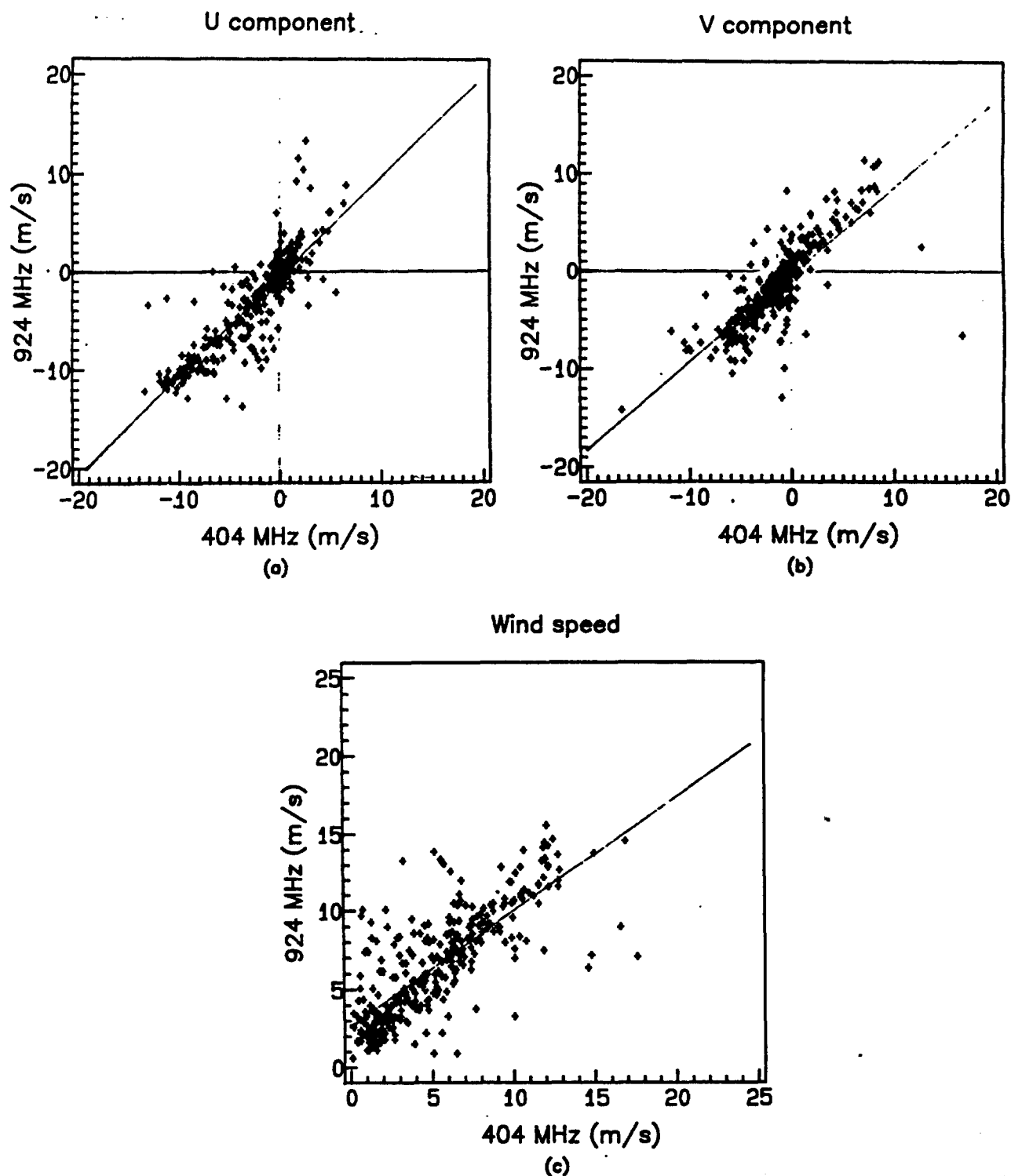
Figure E-5. Regression lines for (a) U component, (b) V component, and (c) resultant wind speed based on measurements with a 924-MHz wind profiler and a 404-MHz wind profiler, APRF site, during 10 of 14 WF-100 measurement periods listed in table 3 (60-min averages).
