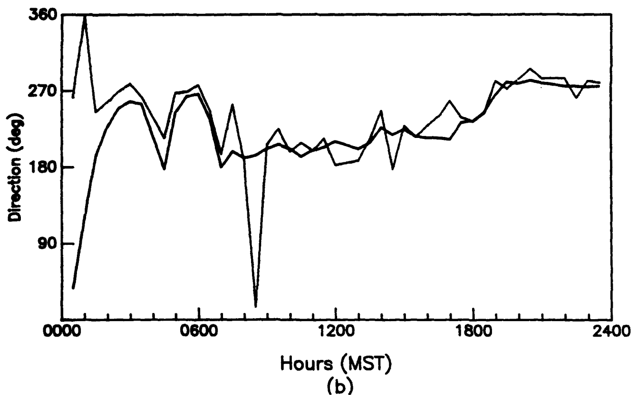
Figure 84. Diurnal variation of (a) wind speed and (b) wind direction as measured with a 924-MHz profiler at 120 m AGL (APRF site) and tower-mounted anemometers at 90, 120, and 150 m AGL (LC-35), WSMR, 0000 to 2400 MST, 15 April 1992 (30-min averages).
