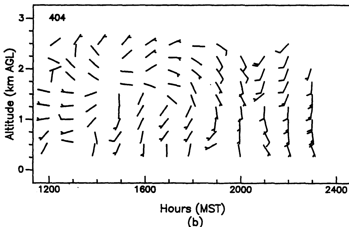
Figure 65. Vertical profiles of wind speed and wind direction, as measured with (a) a 924-MHz profiler and (b) a 404-MHz profiler, APRF site, WSMR, 1200 to 2400 MST, 20 August 1992 (1-h averages).
