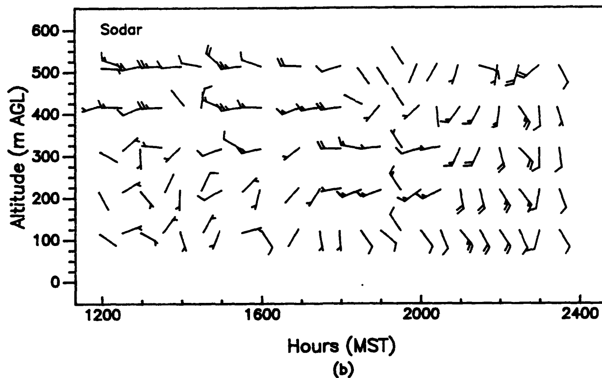
Figure 47. Vertical profiles of wind speed and wind direction, as measured with (a) a 924-MHz profiler and (b) a sodar, APRF site, WSMR, 1200 to 2400 MST, 8 July 1992 (15-min averages).
