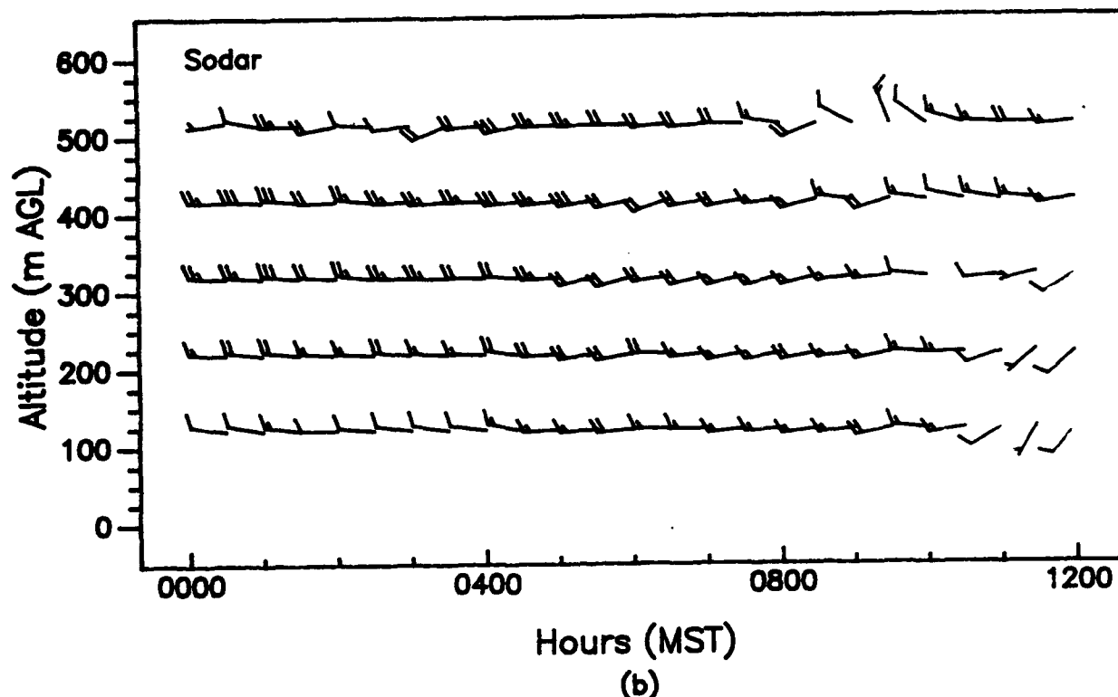
Figure 40. Vertical profiles of wind speed and wind direction, as measured with (a) a 924-MHz profiler and (b) a sodar, APRF site, WSMR, 0000 to 1200 MST, 1 July 1992 (15-min averages).
