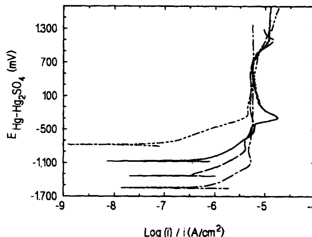
FIGURE 1. Polarization curves for AA 7075-T6 (—), AA 2090-T8E41 (---), AA 8090-T851 (----), and AA 8090-T82551 (-----) alloys after 3 h immersion in aerated 0.5 M Na_2SO_4 . Scan rate = 1 mV/s.
