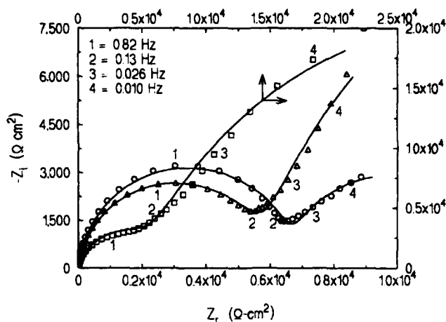
FIGURE 5. Experimental (points) and calculated (lines) impedances for various Al alloys in deaerated 3.5% NaCl: AA 2090-T8E41, after 4 h of immersion (□); AA 2090-T8E41, 5 days (○); and AA 8090-T851, 2 days (Δ).
