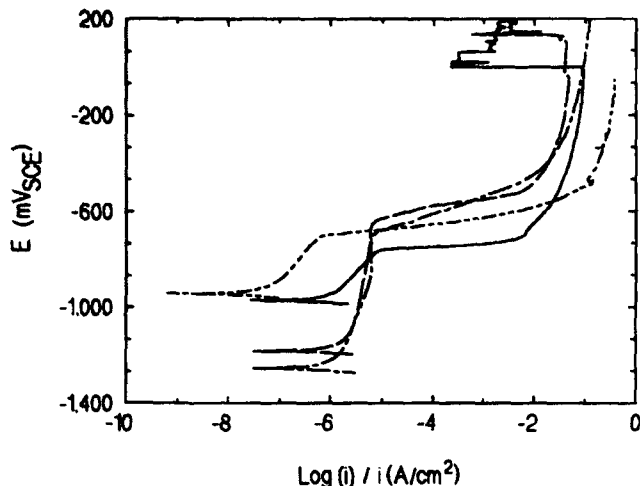
FIGURE 3. Polarization curves for AA 7075-T6 (—), AA 2090-T8E41 (---), AA 8090-T851 (----), and AA 8090-T82551 (-----) alloys after 3 h immersion in deaerated 3.5% NaCl. Scan rate = 1 mV/s.
