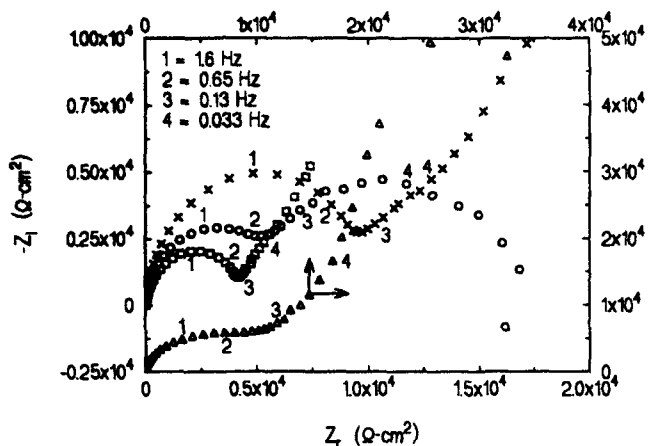
FIGURE 7. Experimental impedances for various Al alloys in aerated 3.5% NaCl: AA 2090-T8E41, after 3 h of immersion (○); AA 2090-T8E41, 3 days (□); AA 8090-T851, 1 day (△); and AA 8090-T82551, 4 days (X).
