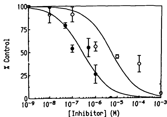
FIG. 5. Inhibition of the NaCN-induced [Ca^{2+}]_i by amiloride (○) and dichlorobenzamil (●). Cells were exposed to NaCN (10 mM, 10 min) in Na^+ Hanks' solution containing different concentrations of either inhibitor. Cells were then washed thoroughly before [Ca^{2+}]_i measurements. Two sigmoid-curved fits are presented. The calculated K_{1/2} for amiloride and dichlorobenzamil are 5.4 and 0.28 \mu M , respectively.
