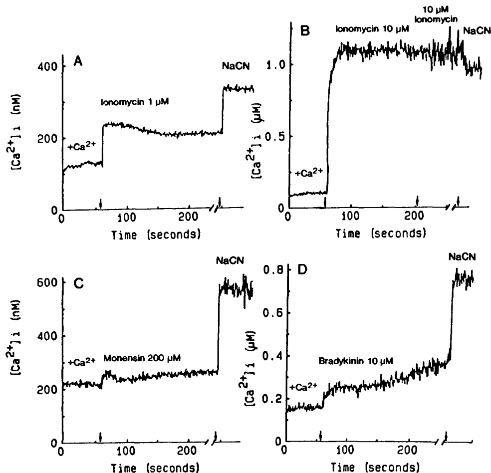
FIG. 7. Depletion of only the ionomycin-sensitive Ca^{2+} pools affects the increase in [Ca^{2+}]_i induced by NaCN. Cells incubated in buffer containing 1.6 mM Ca^{2+} ( +Ca^{2+} ) were pretreated with (A) 1 \mu M ionomycin, (B) 10 \mu M ionomycin, (C) 200 \mu M monensin, or (D) 10 \mu M bradykinin prior to NaCN exposure (10 mM, 10 min). The break on the x axes represents the time interval for NaCN treatment.
