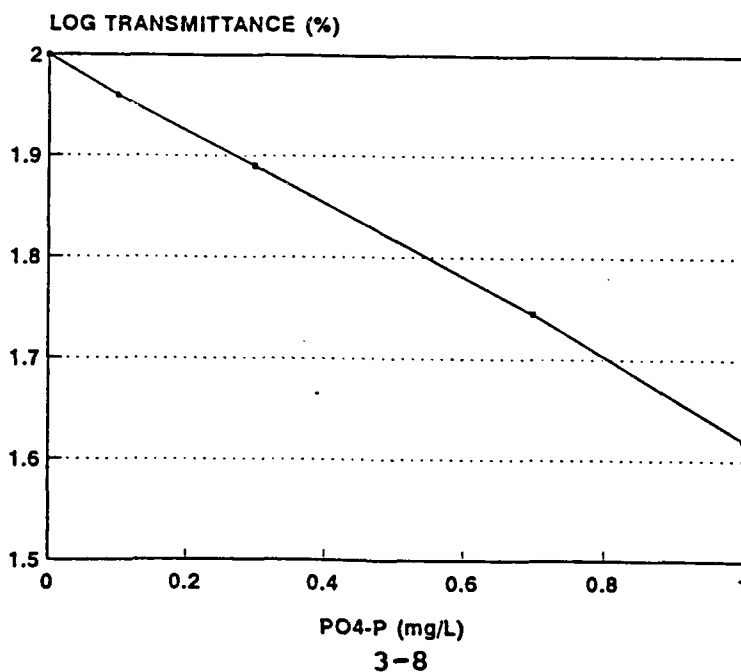
Figure 3.3 - Log Transmittance vs \text{PO}_4\text{-P} for Pilot Study 7
