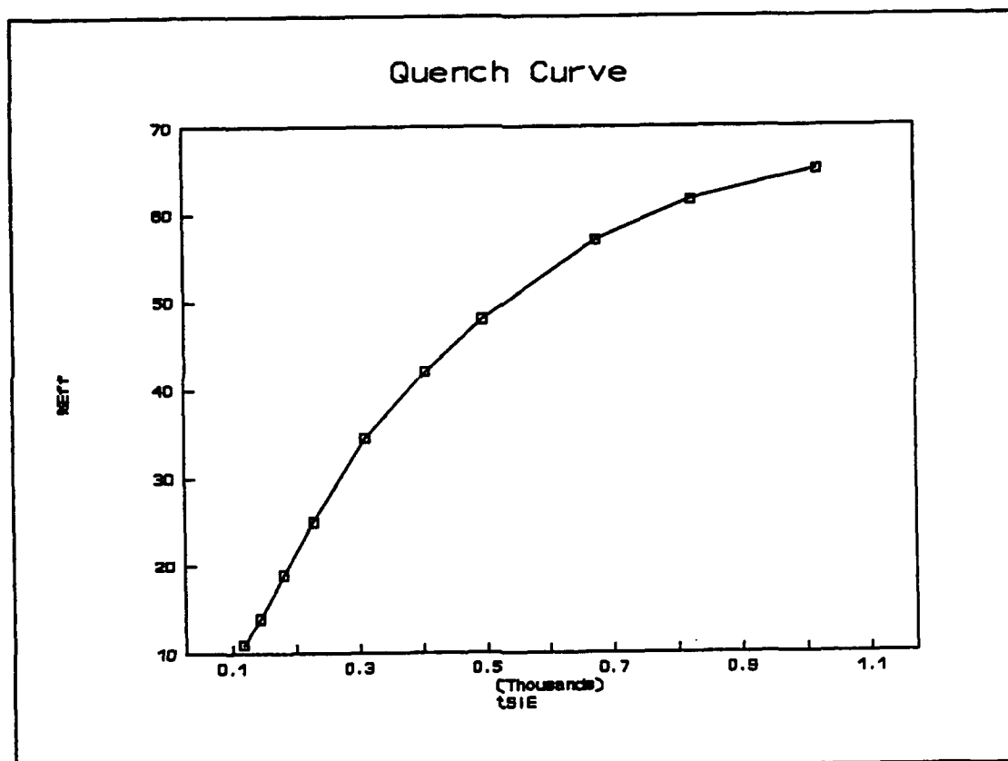
Figure 2-8: Quench Curve
