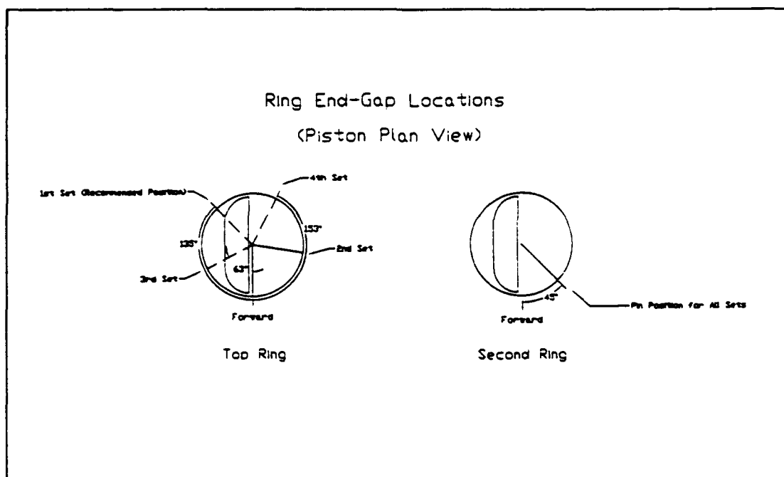
Figure 4-1: Top Ring Gap Locations
