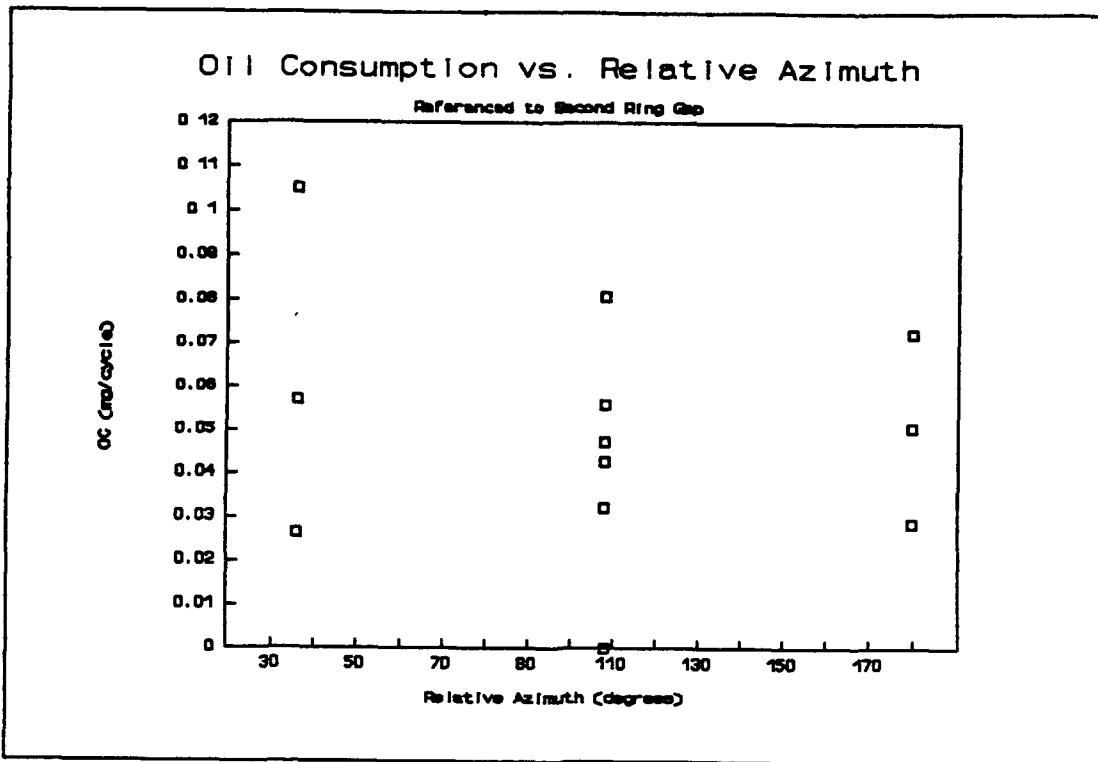
Figure 5-24: OC vs. \theta_2
