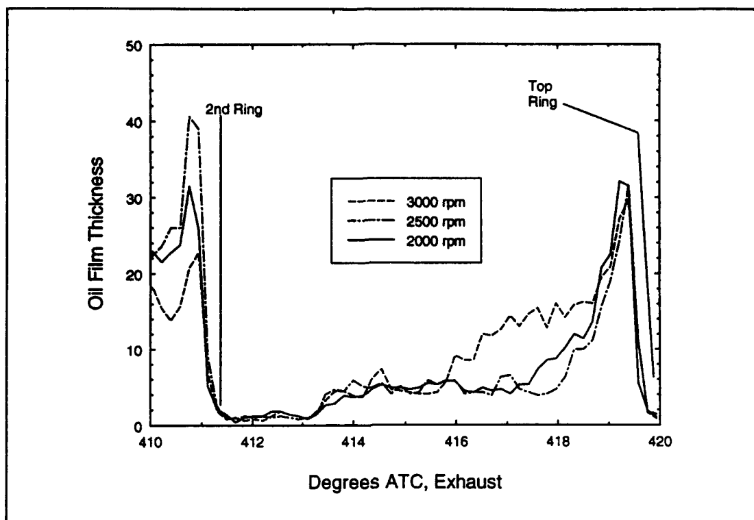
Figure 5-16: 2nd Land Oil Film Thickness, AZ5( \theta=225^\circ )
