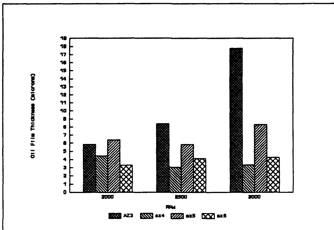
Figure 5-18: Average 2nd Land Oil Film Thickness
