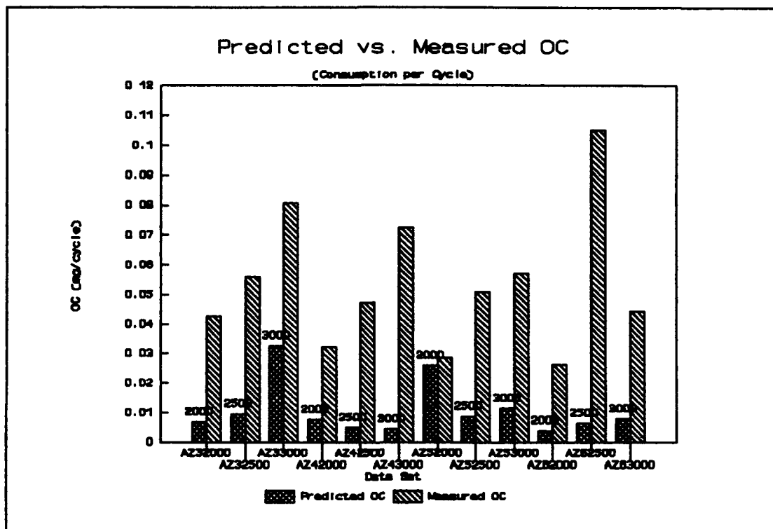
Figure 5-19: Shaw Model Predictions of Oil Consumption
