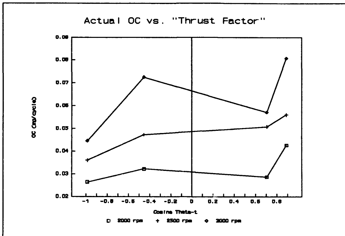
Figure 5-23: Actual OC vs. \theta_t
