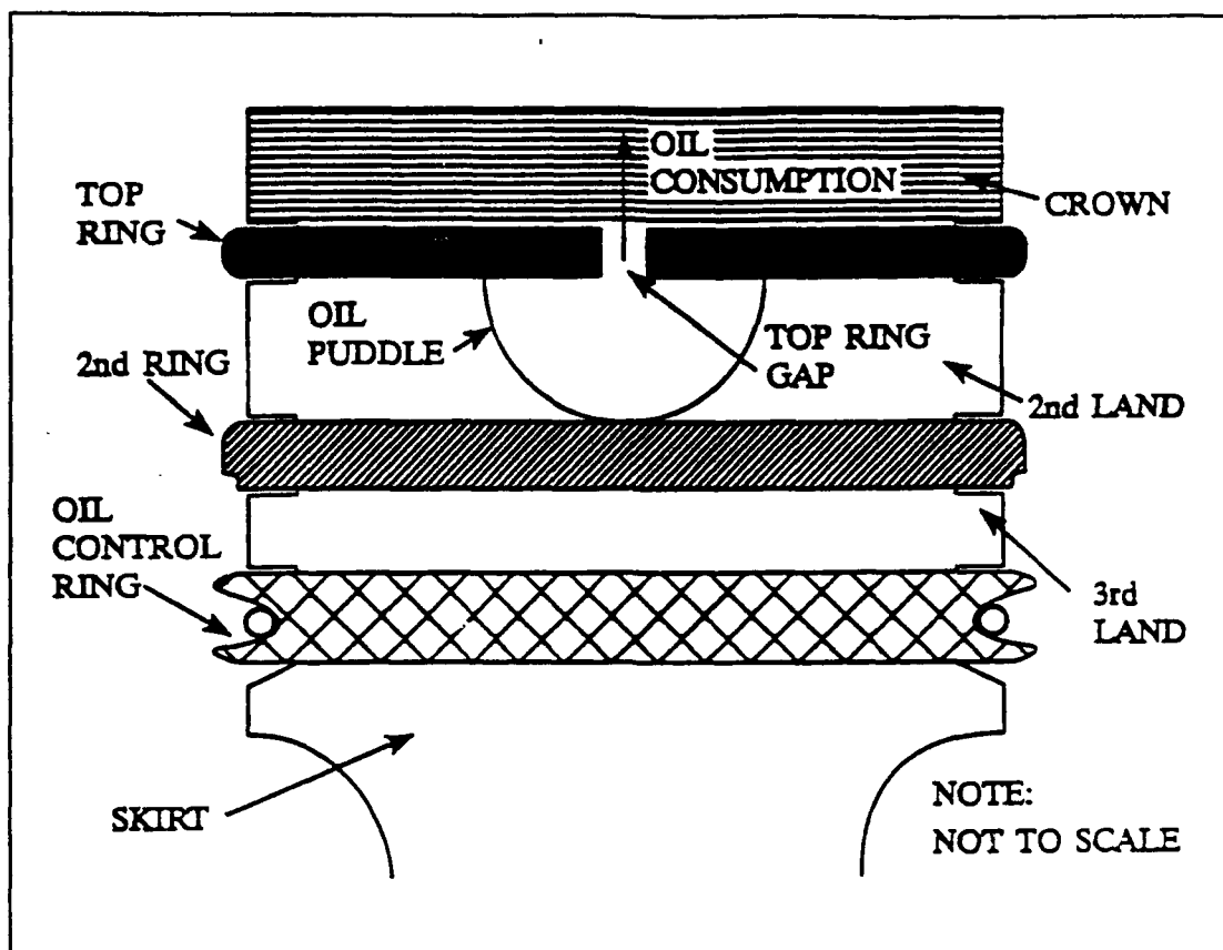
Figure 1-1: Geometry of the Oil Puddle Model
