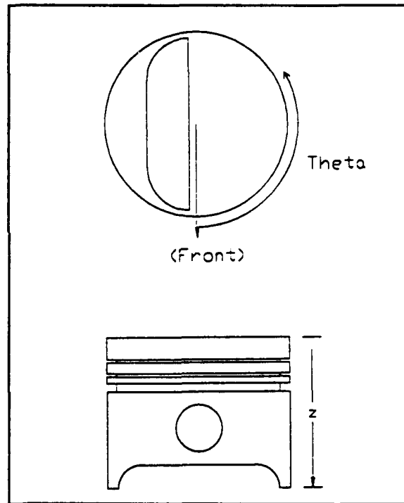
Figure 2-1: Piston Coordinate System
