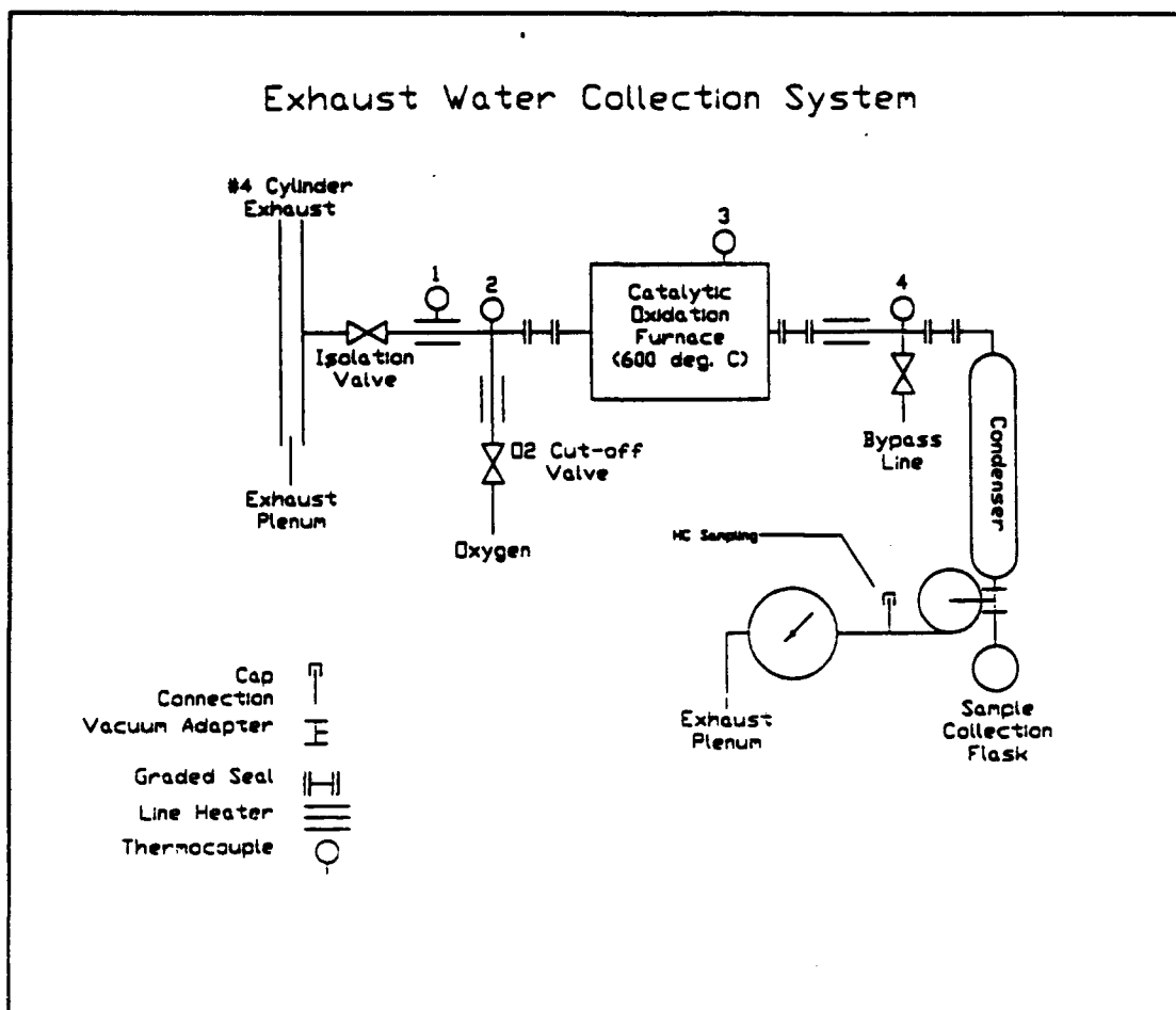
Figure 3-5: WCS Schematic
