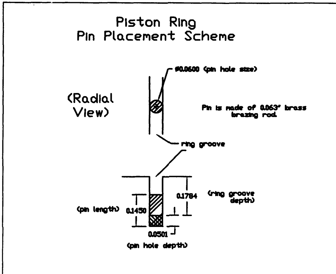
Figure 3-1: Pin Schematic
