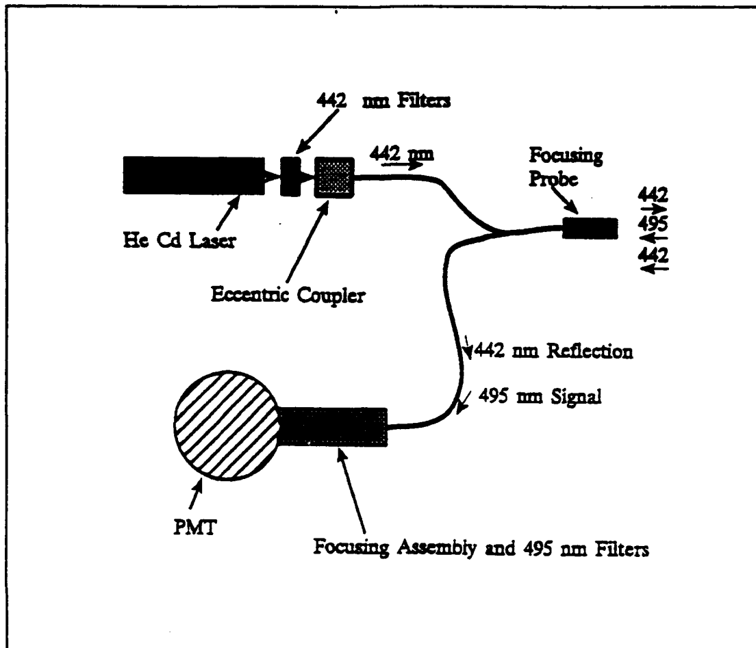
Figure 2-7: LIF Schematic
