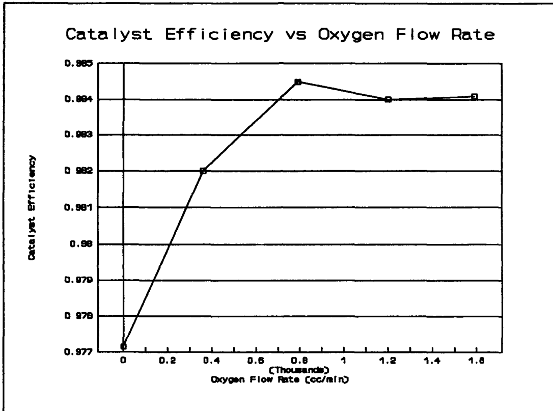
Figure 5-1: Supplemental Oxygen Effect on Catalyst Efficiency.
