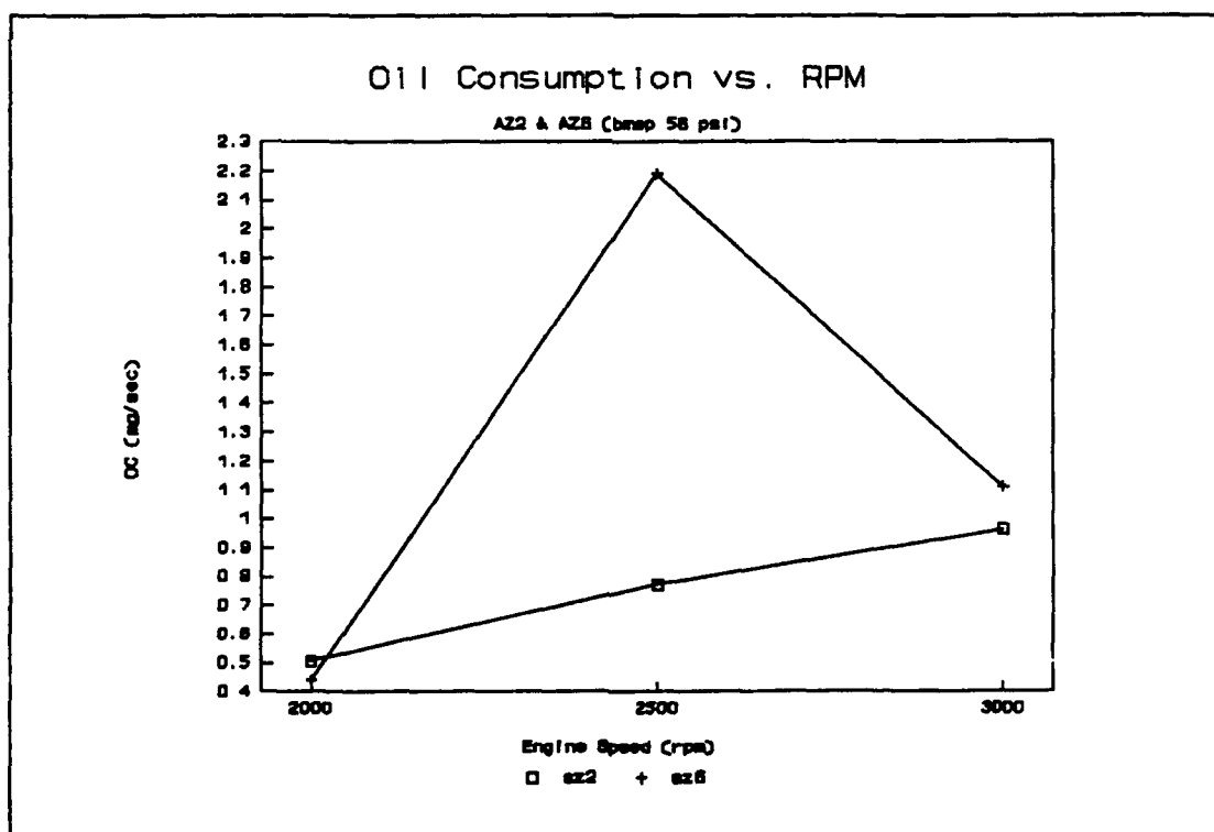
Figure 5-12: OC vs. Engine Speed (Top Gap @ \Theta=81^\circ )
