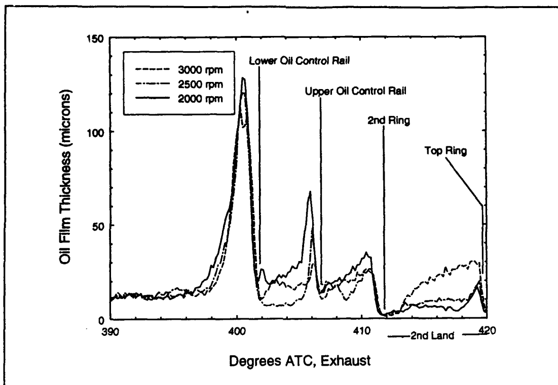
Figure 5-14: Oil Film Thicknesses, AZ3 ( \theta=297^\circ )
