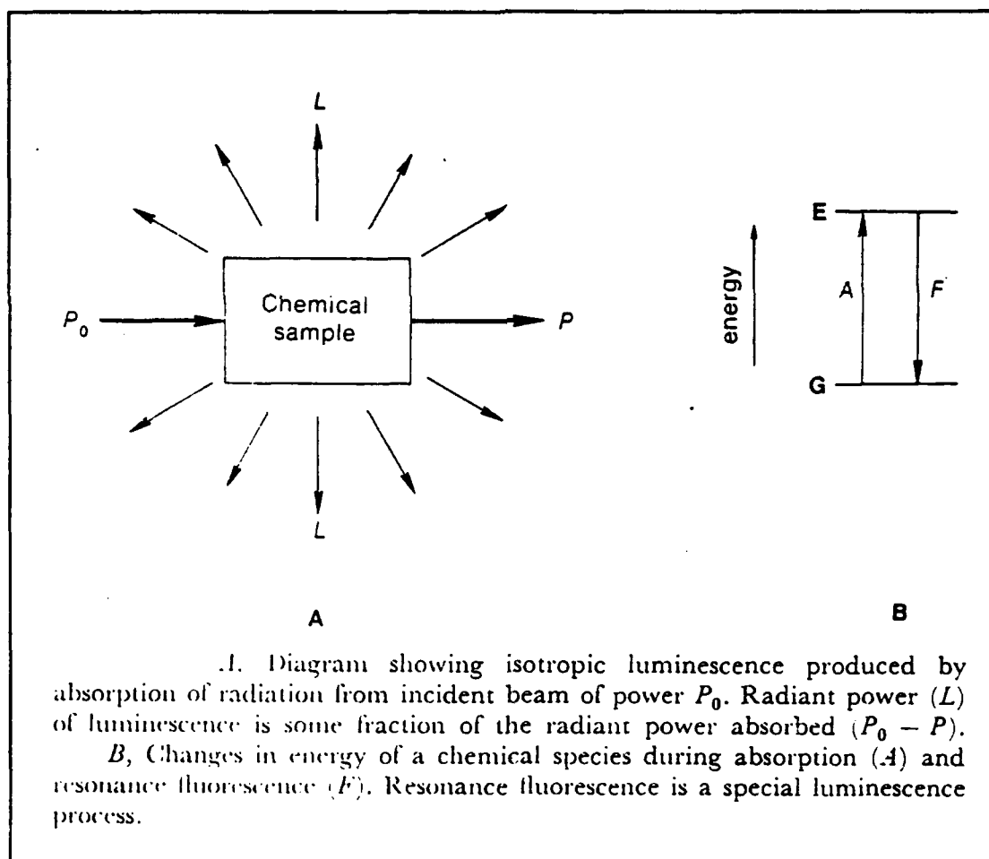
Figure 2-5: Luminescence Process
