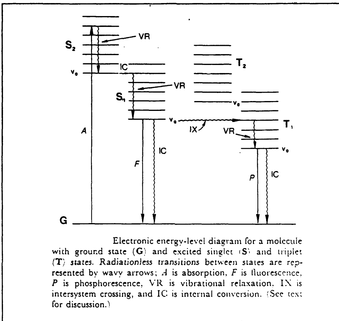
Figure 2-6: Electron Transitions for Luminescent Processes
