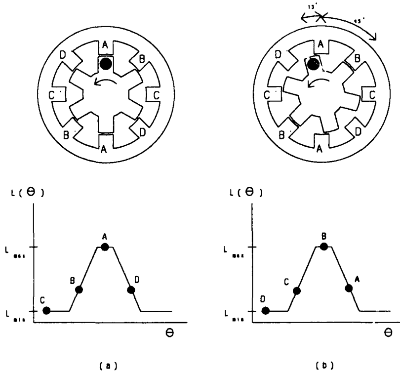
Figure 2.3 (a) Rotor position and inductance of the four phases with phase A aligned. (b) Rotor position and inductances for phase B aligned. The stator flux wave shifted 45° CW; the rotor turned 15° CCW.
