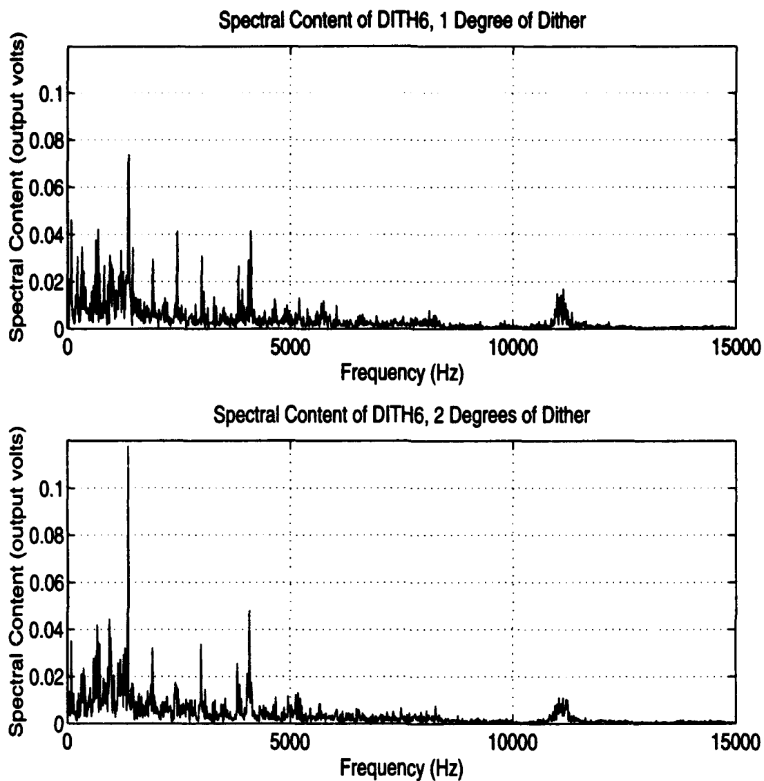
Figure 5.8 Comparison between equal angle trials at dc supply = 30V, chop current = 1.96A, 2700 rpm, scheme DITH6 with 1 degree and 2 degrees of OFF dither.
