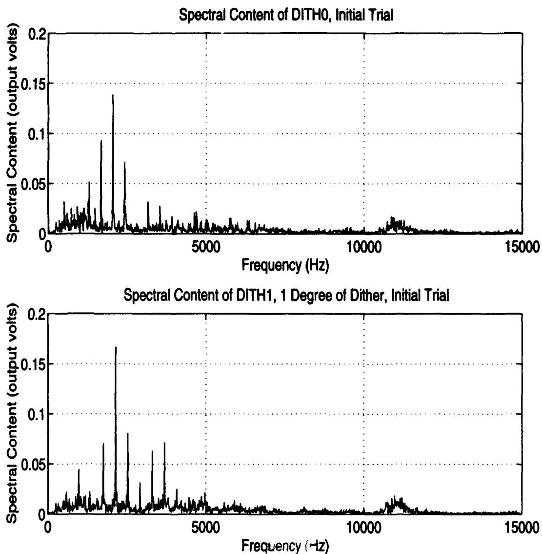
Figure 5.9 Comparison between initial trials without equal angles and before optimizing at dc supply = 30V, chop current = 2.35A, DITH0 no dither and DITH1 with 1 degree of ON dither. DITH0 speed = 1600 rpm, DITH1 speed = 1670 rpm.
