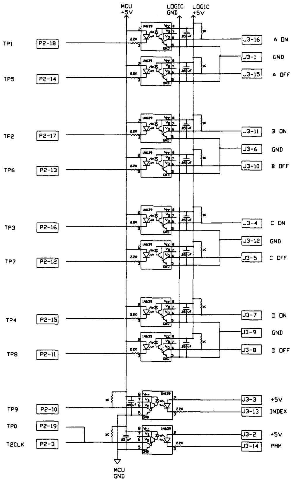
MCU Interface Board
