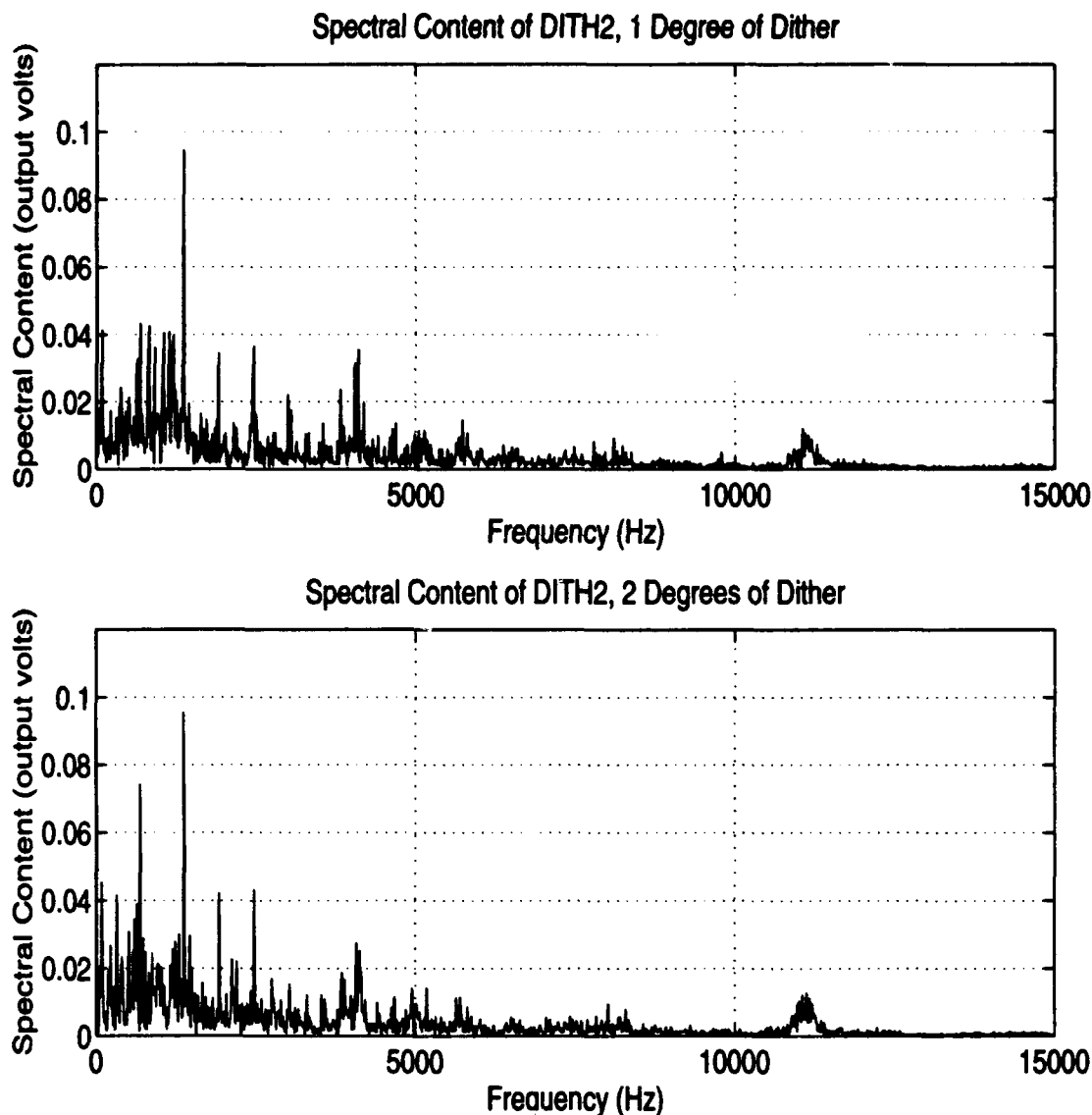
Figure 5.5 Comparison between equal angle trials at dc supply = 30V, chop current = 1.96A, 2700 rpm, scheme DITH2 with 1 degree and 2 degrees of OFF dither.
