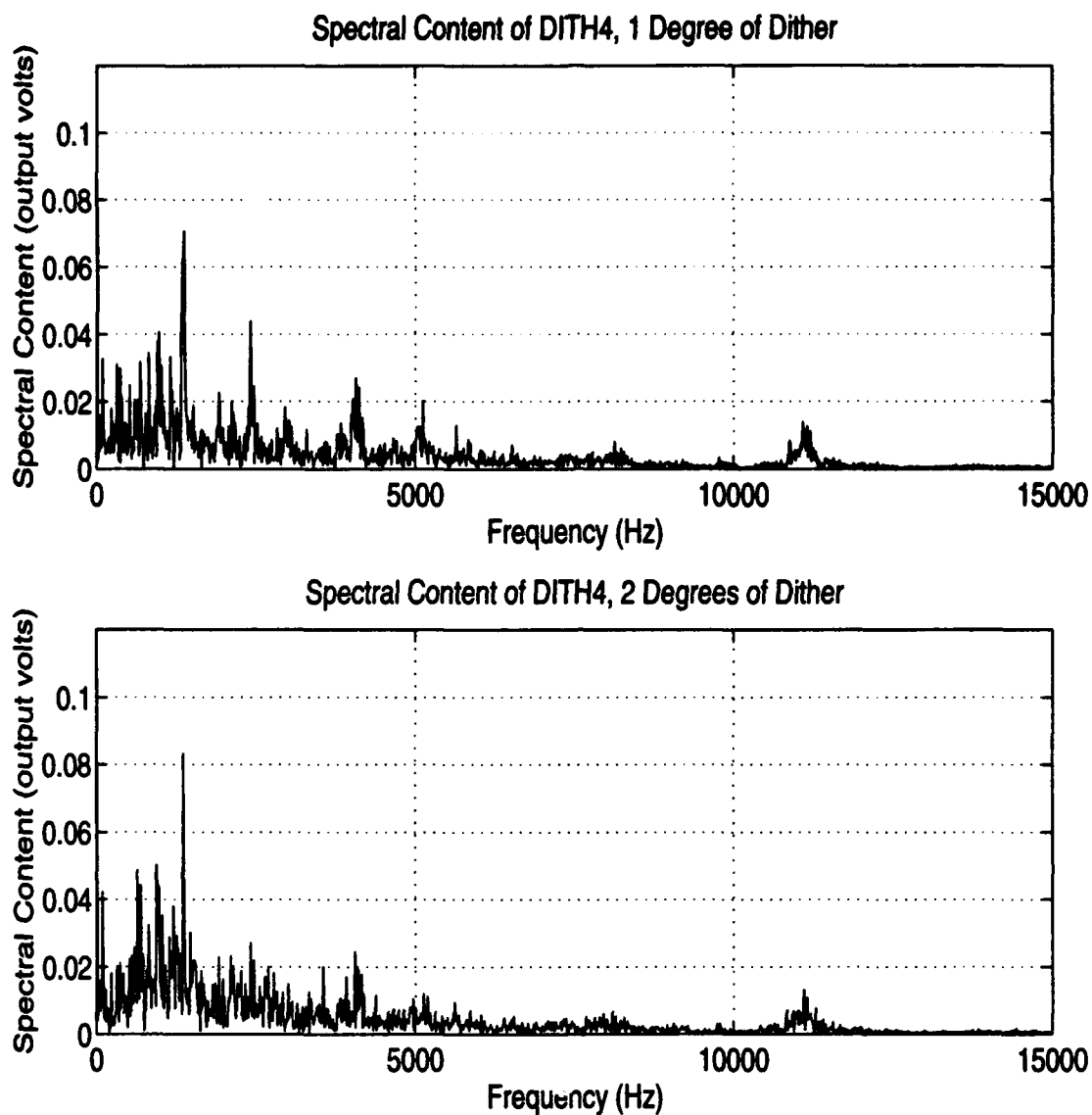
Figure 5.6 Comparison between equal angle trials at dc supply = 30V, chop current = 1.96A, 2700 rpm, scheme DITH4 with 1 degree and 2 degrees of OFF dither.
