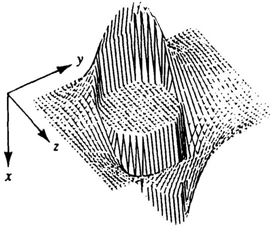
Figure 9. Shear stress \sigma_{xi} , rotating about the z -axis around cylindrical column cavities, showing phasing relationship. Excitation from direction of y -axis.
