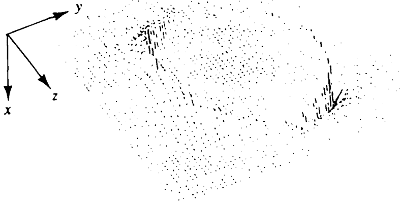
Figure 10. Shear stress \sigma_{xi} , rotating about the z -axis around the upper rim of a cylindrical cavity, showing the phasing relationship. Excitation from above figure in direction of x -axis.
