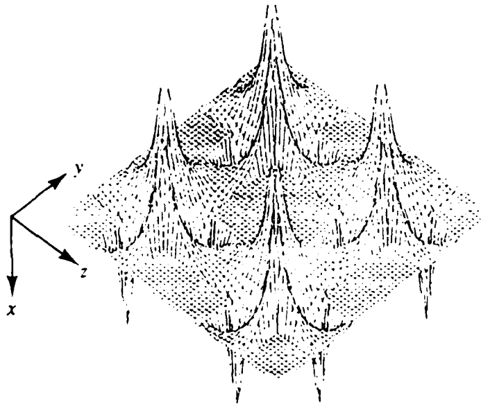
Figure 8. Shear stress \sigma_{yz} rotating about the x -axis around cubical cavities, showing the phasing relationship around and between cavities. Nodal lines are readily visible. Excitation from above figure in direction of x -axis.
