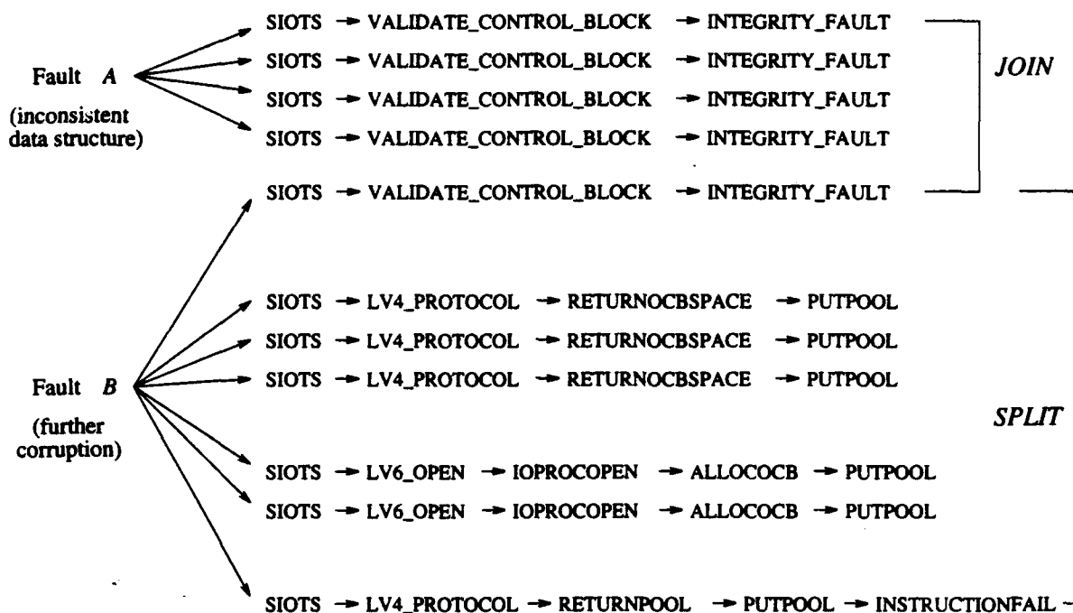
Figure 7.10 Examples of Join and Split
