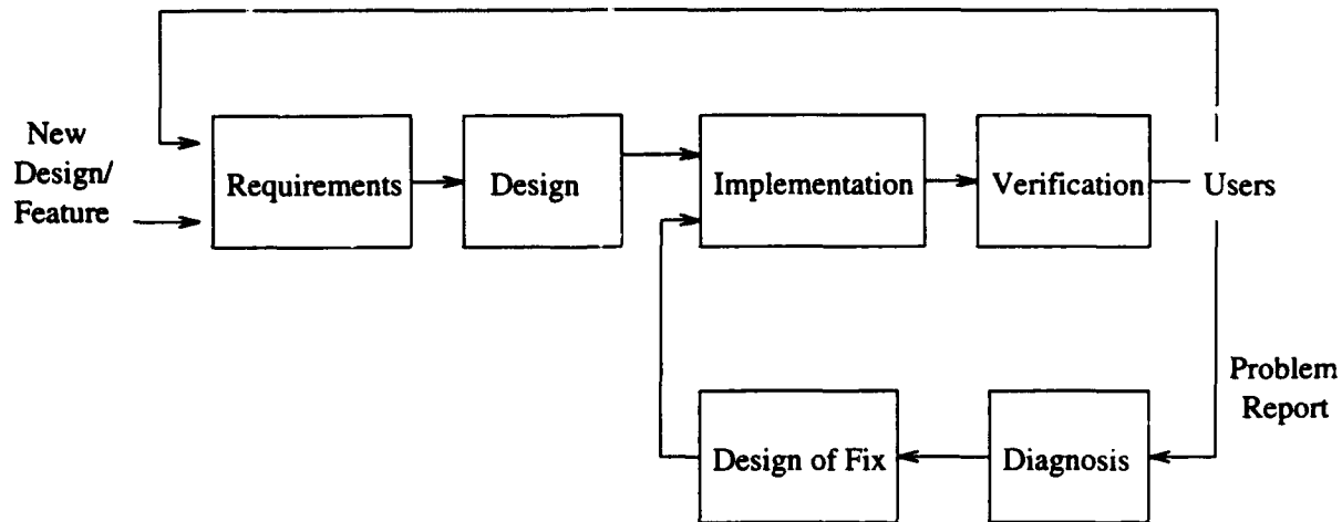
Figure 7.4 Software Development and Service
