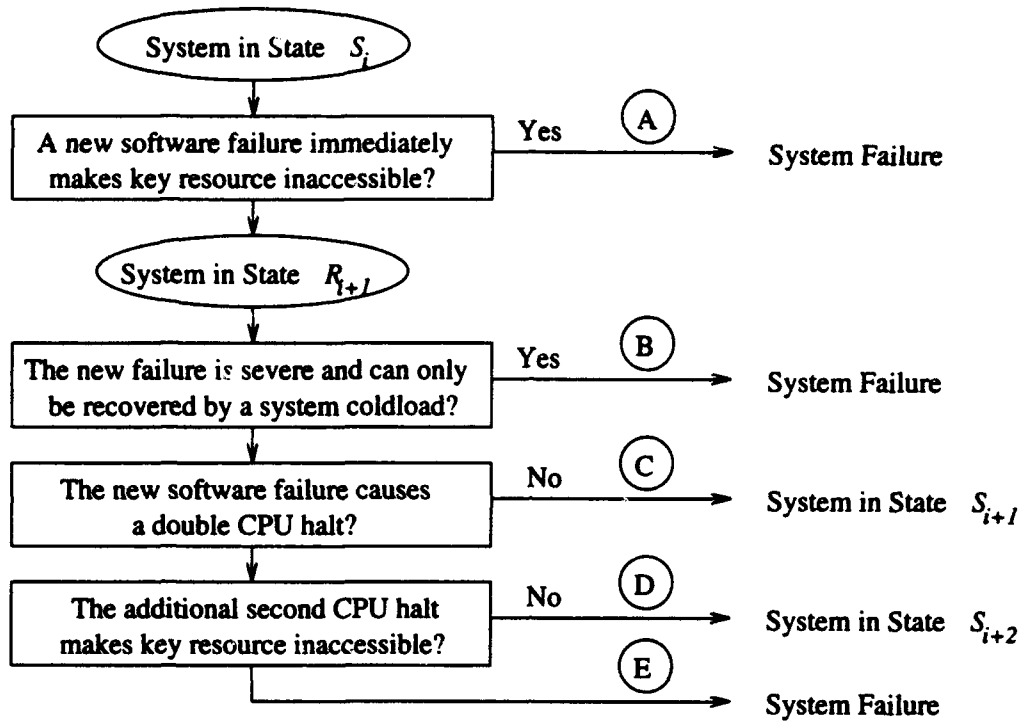
Figure 6.2 Effect of Multiple Independent Software Failures
