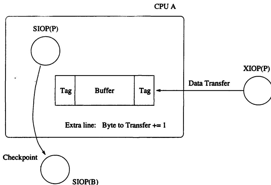
Figure 4.3 Effect of Error Latency
