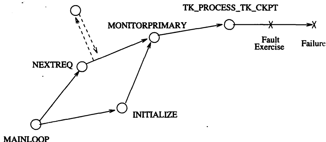
Figure 7.6 Detection near Faulty Code
