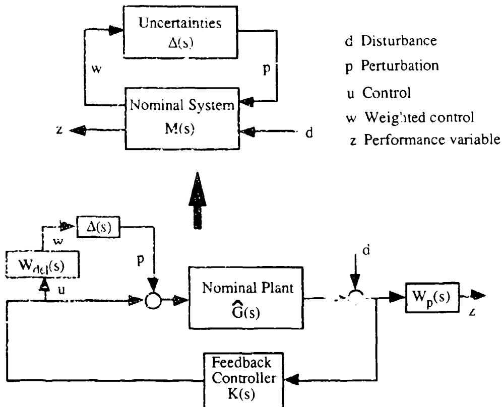
Figure 2-4. Transfer Matrix with Perturbations
