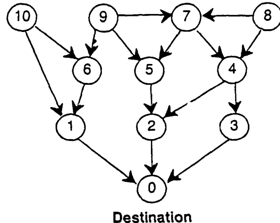
Figure 4: A destination-oriented DAG.
