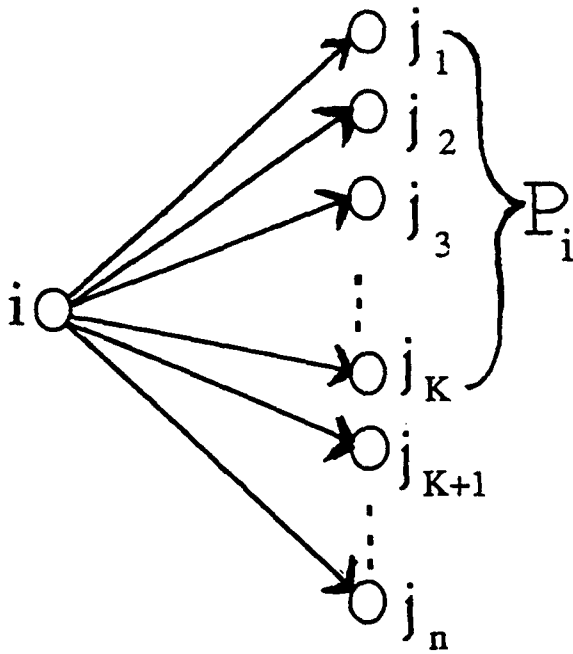
Figure 3: Optimal routing strategy for node i .
