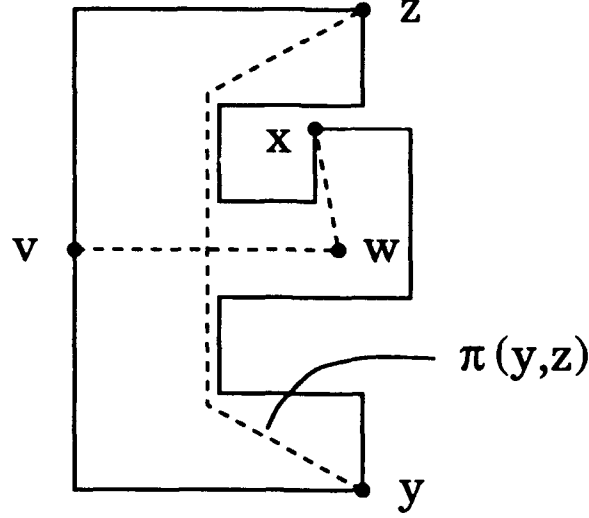
Figure 1: w is visible from x ; v is link-2-visible from x ; y and z are separable from w and link-2-separable from x .
