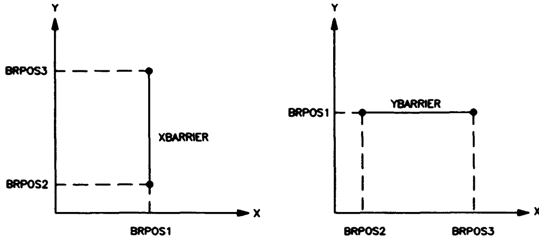
Figure 14-16. Definitions of XBARRIER and YBARRIER
