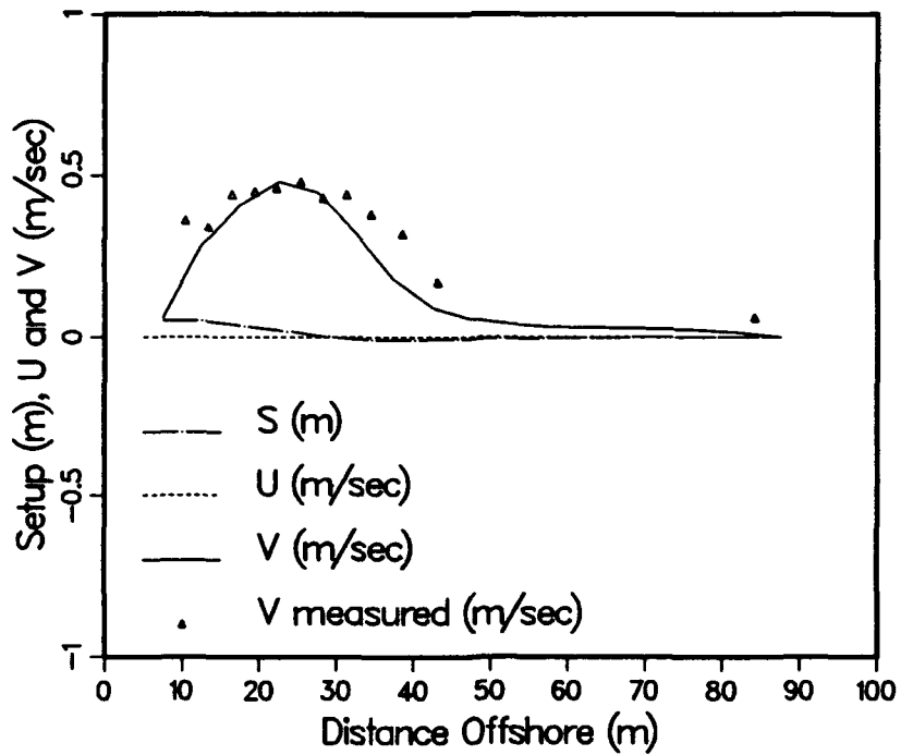
Figure 14-27. WICM results for Leadbetter Beach simulation (driven by STWAVE)
