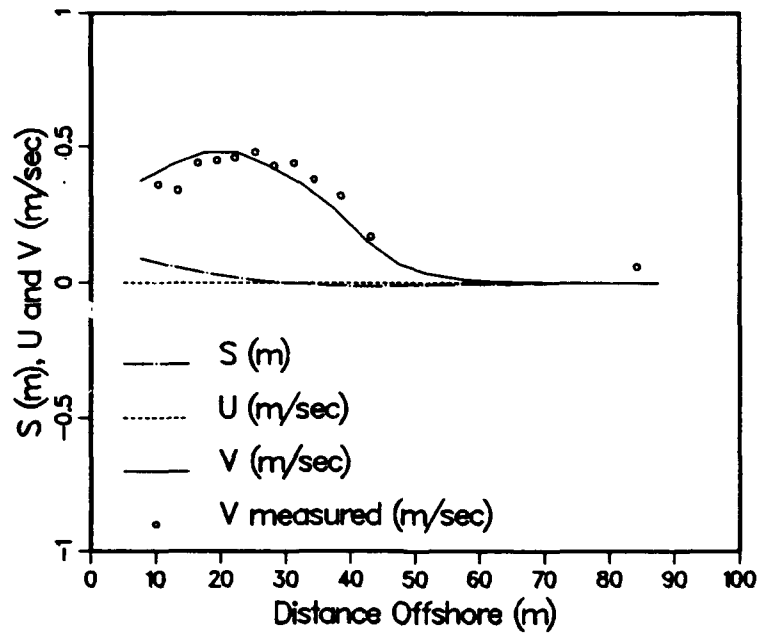
Figure 14-25. WICM results for Leadbetter Beach simulation (driven by RCPWAVE)
