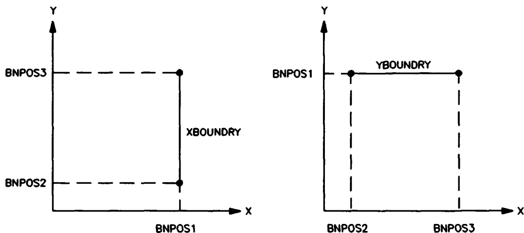
Figure 14-18. Definition of XBOUNDRY and YBOUNDRY
