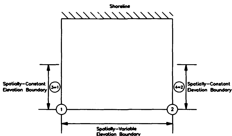
Figure 14-19. Example showing use of BDNFN1, BDNFN2, and FUNNO variables
