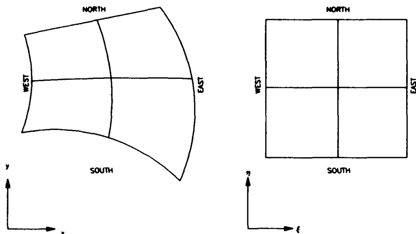
Figure 14-5. Physical and transformed planes
