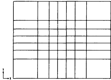
Figure 14-3. Stretched Cartesian grid
