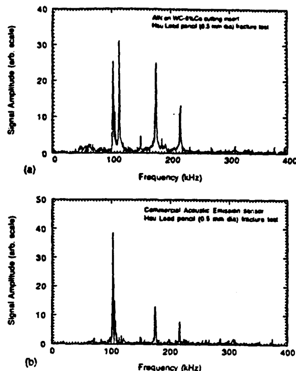
FIG. 7. Frequency domain signals detected by (a) the AlN thin film sensor on WC-Co cutting insert (b) a commercial AE sensor attached to the tool holder as shown in Fig. 1. Signals were band pass filtered (100–500 kHz). Mechanical pencil lead fracture test of Hsu (see the text for details). Frequency content is virtually identical. Source of the dominant peak just above 100 kHz observed in the signal from AlN on WC-Co insert has not been identified.
