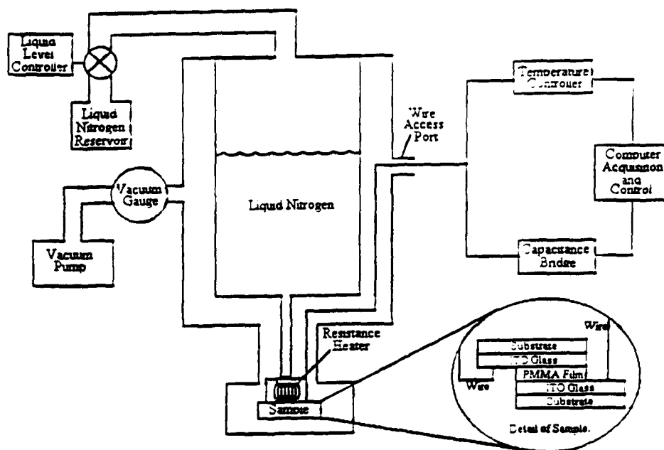
Figure 1. Experimental dewar system
