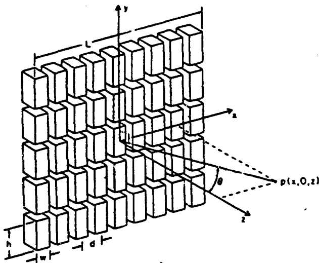
Figure 17. Stack of five linear planar phased arrays.
