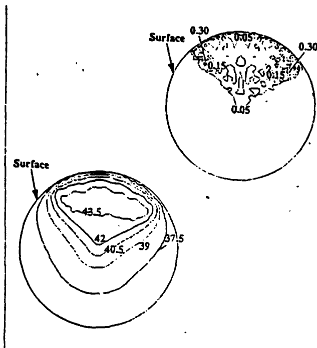
Figure 7. Top panel: SAR distribution ( W/cm^3 ) required to maintain steady state temperature equilibrium 42^\circ C \leq T \leq 44^\circ C for treatment of a quadrant of the breast. Bottom panel: The resulting steady state temperature distribution. The maximum temperature is 43.7^\circ C .
