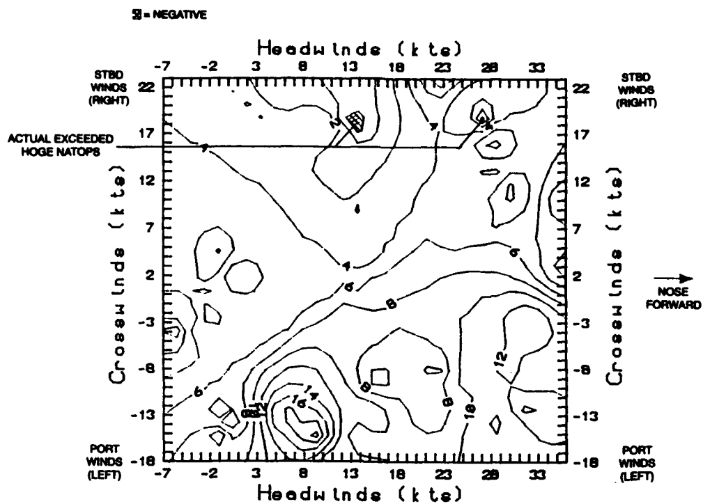
Figure 9 VARIATION OF CH-53E TEST HOVER TORQUE WITH NATOPS HOGUE TORQUE PREDICTIONS
