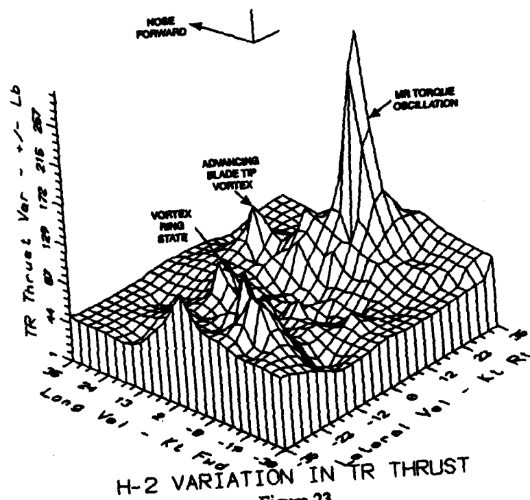
Figure 23 H-2 VARIATION IN TR THRUST
