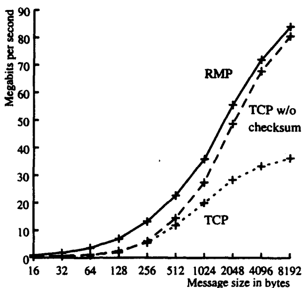
Figure 2: CAB-to-CAB throughput
