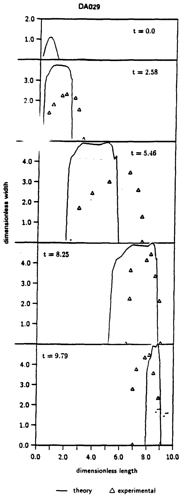
Figure 4: Sequence of nondimensional computed and experimental pile width and computed pile height at frame time increments for DA029
