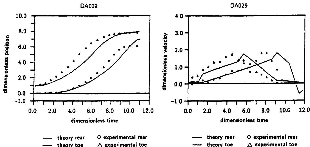
Figure 3: Theoretical predictions and experimental values of nondimensional position and velocity of the leading and trailing edge as a function of nondimensional time for experiment DA029
