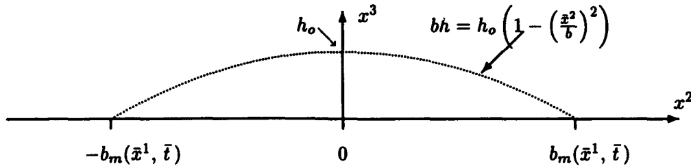
Figure 1: Approximation of pile shape in the \bar{x}^1 plane
