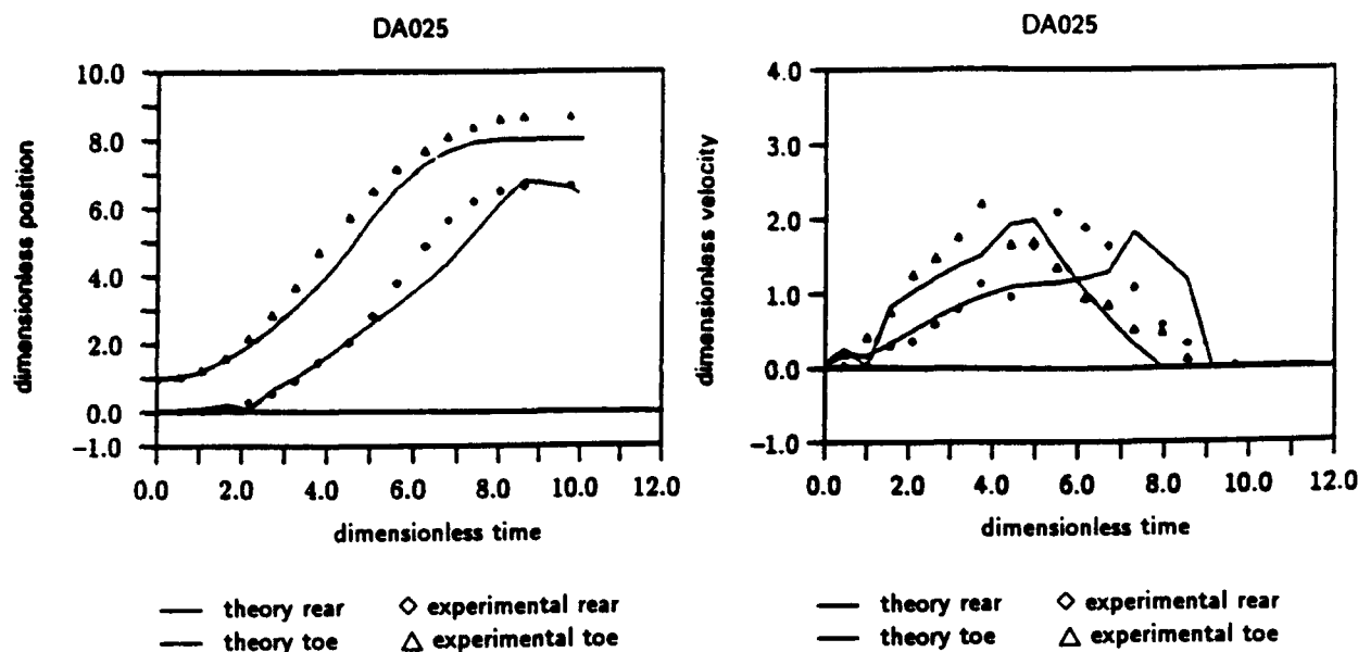
Figure 5: Theoretical predictions and experimental values of nondimensional position and velocity of the leading and trailing edge as a function of nondimensional time for experiment DA025
