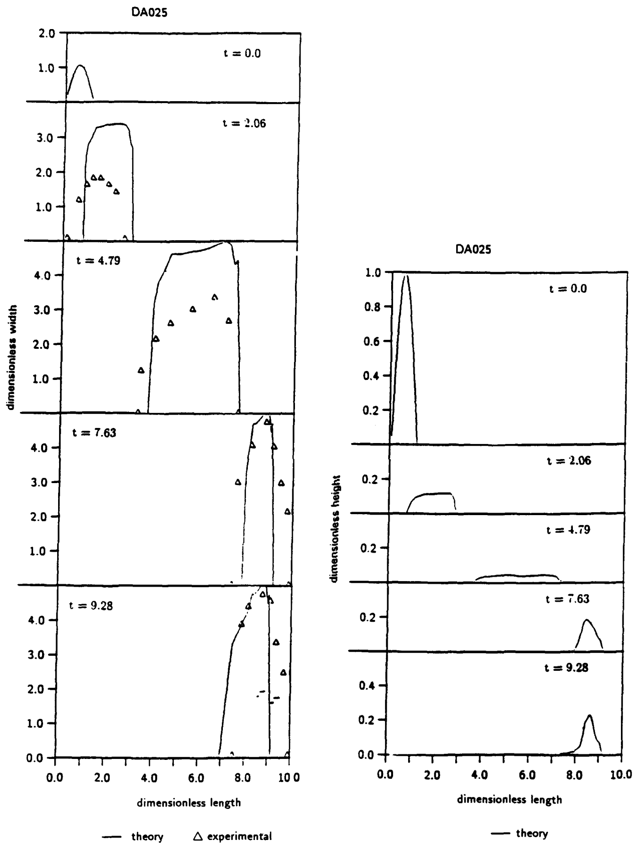
Figure 6: Sequence of nondimensional computed and experimental pile width and computed pile height at frame time increments for DA025
