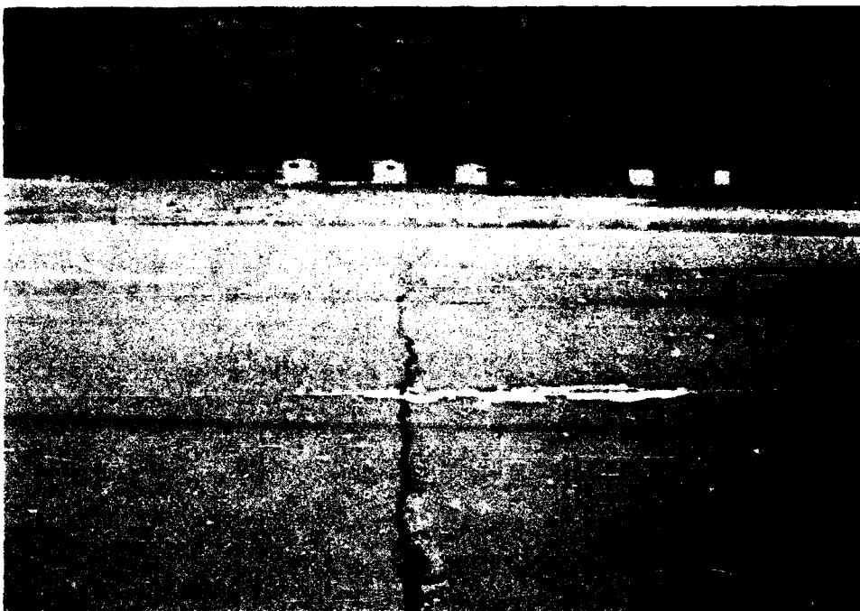
Figure 17. Typical transverse crack (reflected) in interior portion of runway (Item 2)
