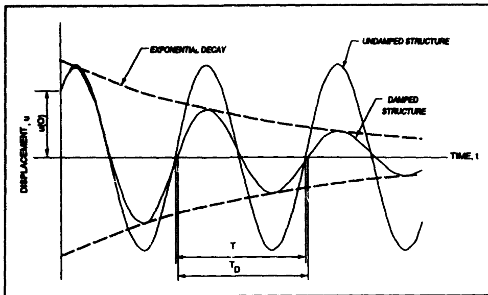
Figure 3. Damped oscillations
