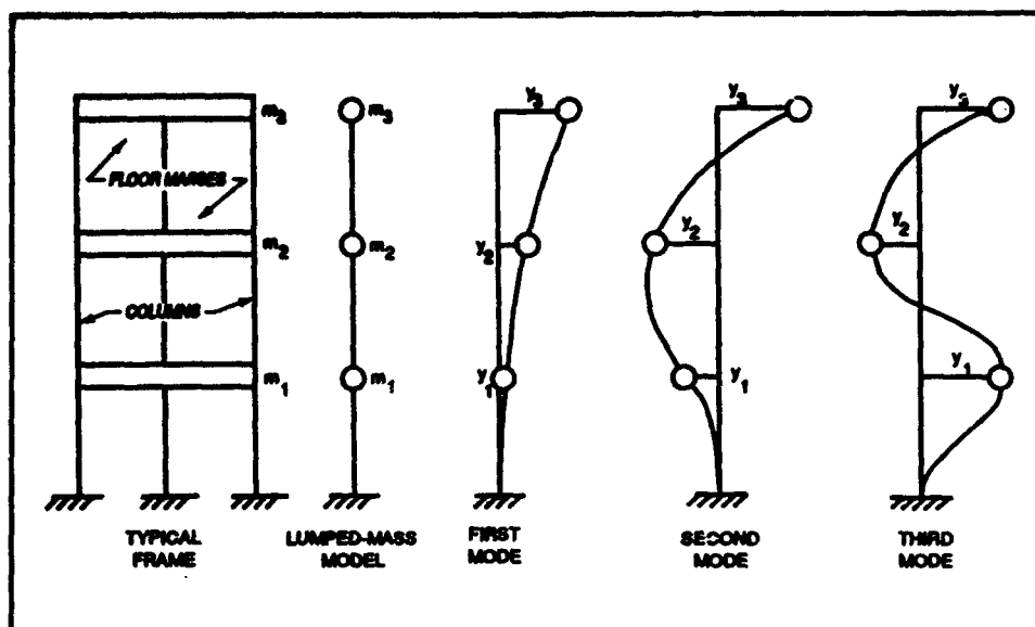
Figure 32. Lumped-mass system
