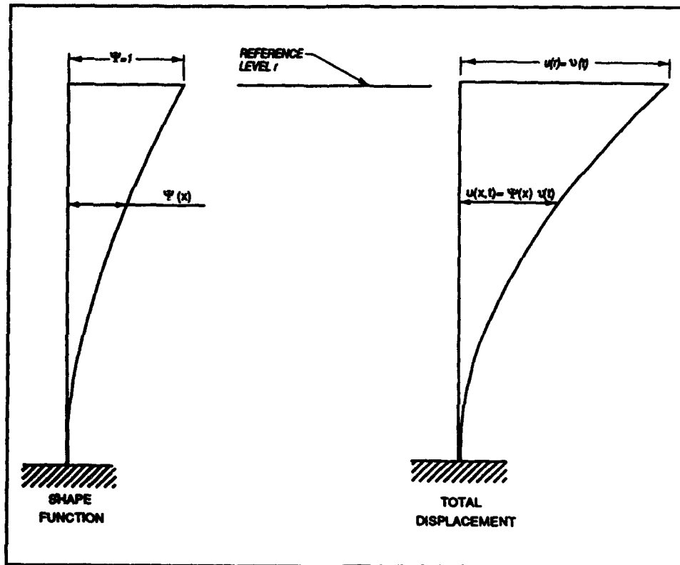
Figure 20. Shape function
