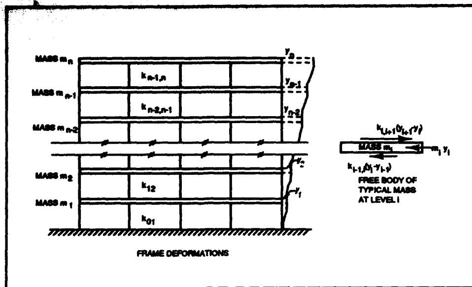
Figure A-1. General lumped-mass building
