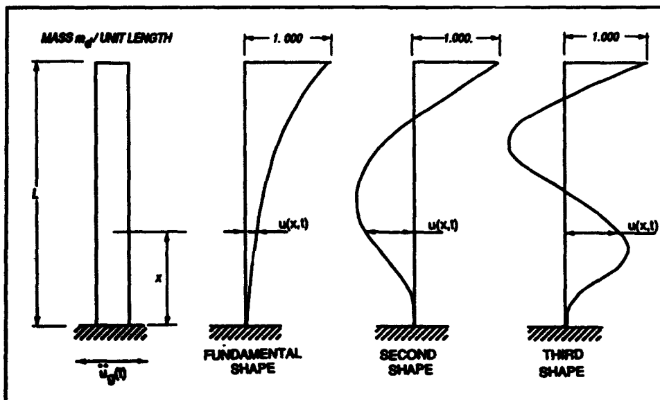
Figure 19. Distributed-mass system
