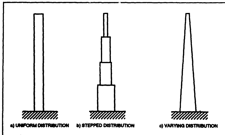
Figure 31. Distributed-mass systems
