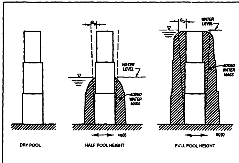
Figure 25. Added mass due to acceleration of water
