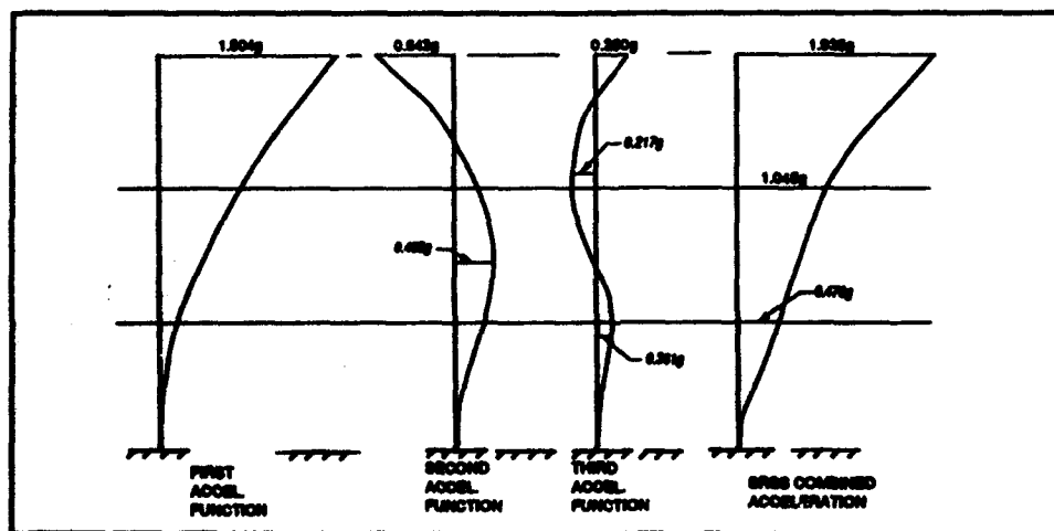
Figure 29. Acceleration functions
