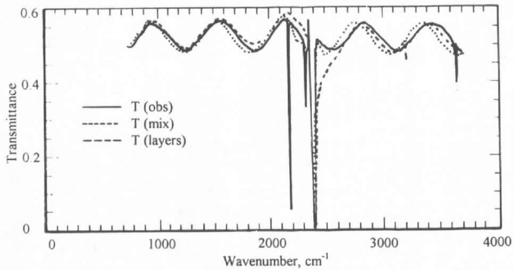
Figure 25. Calculated transmittance of 6.602- \mu m N_2/CO/CO_2 film.
