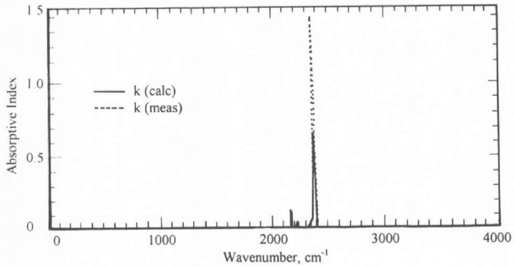
Figure 24. k (calc) and k (meas) of 20K N_2/CO/CO_2 film.
