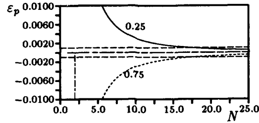
Figure 2: (b) Phase error as function of resolution for the Upwind Leapfrog scheme.
