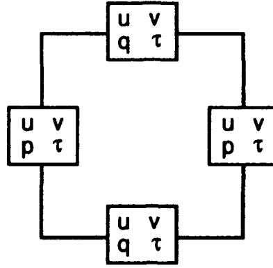
Figure 9: Staggered storage for elastodynamic waves.
