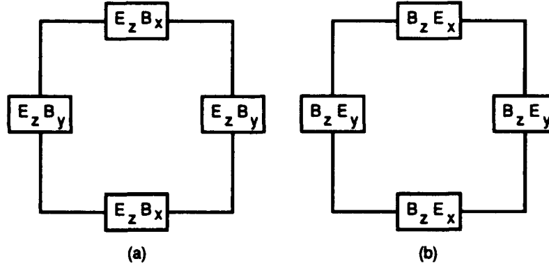
Figure 8: Staggered storage for (a) electrically, and (b) magnetically polarised electromagnetic waves.
