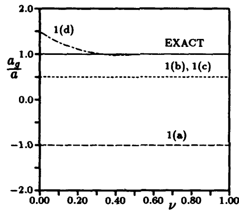
Figure 4: Group velocities of the four schemes for short waves.
