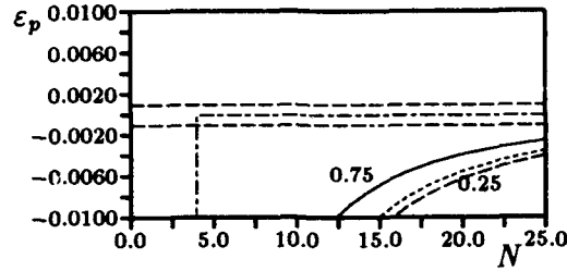
Figure 2: (a) Phase error as function of resolution for the regular Leapfrog scheme. The dashed horizontal lines correspond to one part per thousand.
