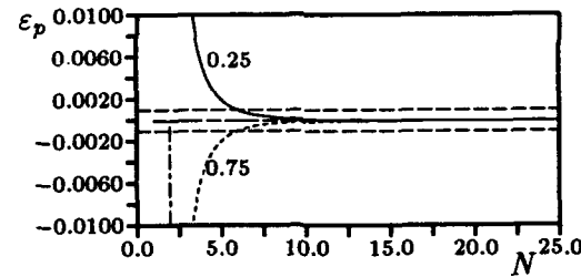
Figure 2: (c) Phase error as function of resolution for the Upwind Leapfrog scheme extended in space.
