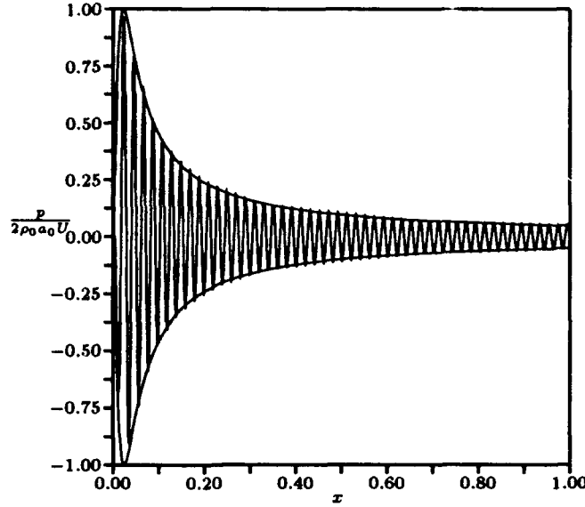
Figure 11: Pressure distribution on the axis of symmetry due to a wall-mounted oscillating piston.
