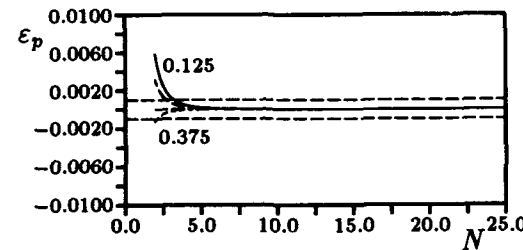
Figure 2: (d) Phase error as function of resolution for the Upwind Leapfrog scheme extended in time. Note that the Courant numbers have been halved.
