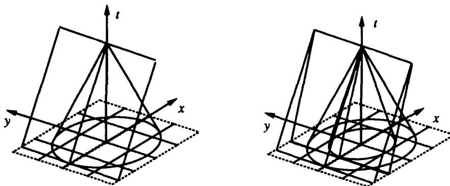
Figure 6: Characteristic planes for waves moving in the positive x -direction, and the characteristic cones. Acoustic problem at left and elastodynamic problem at right.
