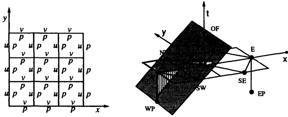
Figure 7: The storage of unknowns on a square grid, and the stencil used to update a u, p point in the second-order scheme. The shaded plane shows a wave moving in the positive x -direction.
