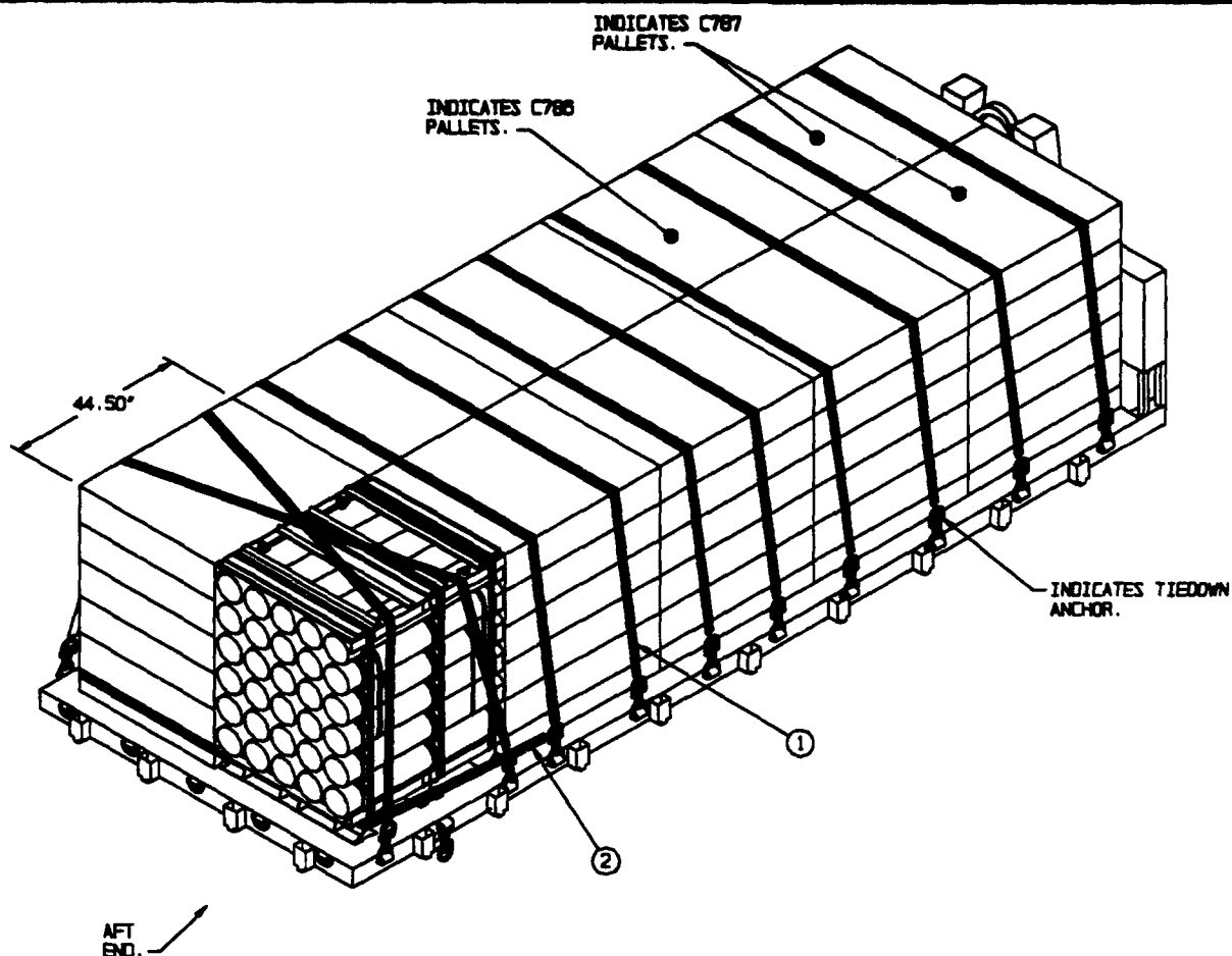
ISOMETRIC VIEW
