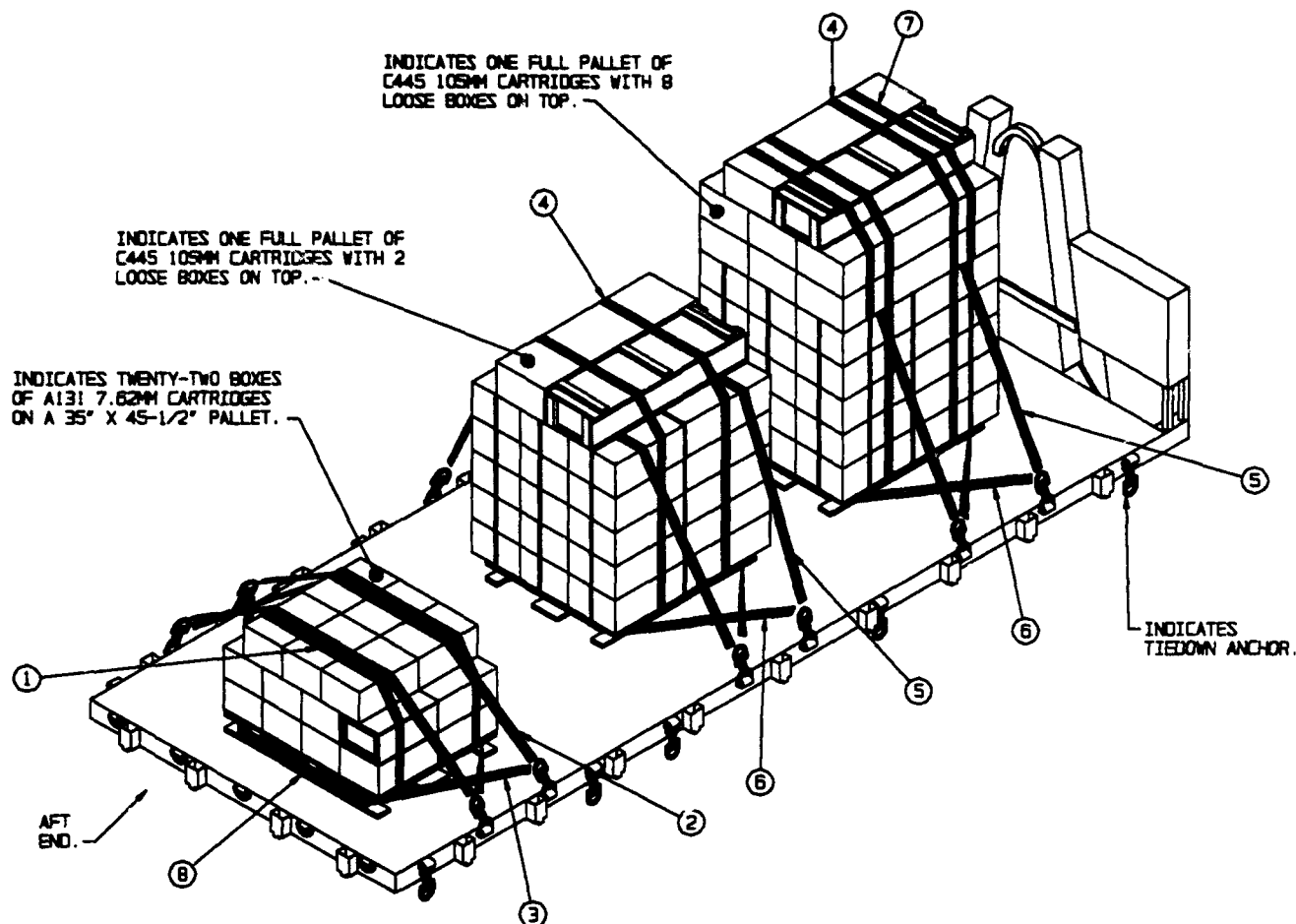
ISOMETRIC VIEW
