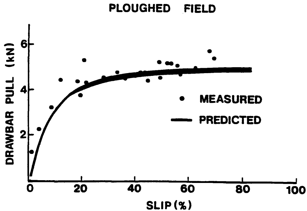
Figure 20. Comparison of the measured and predicted performance of a wheeled tractor on a plowed field
