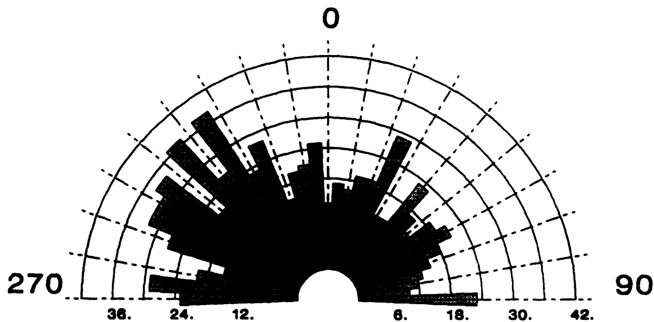
Figure 4. Frequency and Orientation of Fracture Traces and Lineaments in the Nkawkaw Area.
