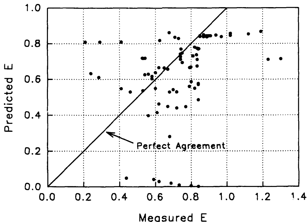
Figure D5. There's adjustment to the Avery and Novak equation for ogee spillways. Predicted values of gas transfer versus measured values
