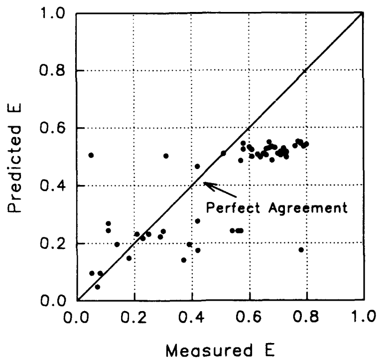
Figure D17. Holler equation for weirs. Predicted values of gas transfer versus measured values
