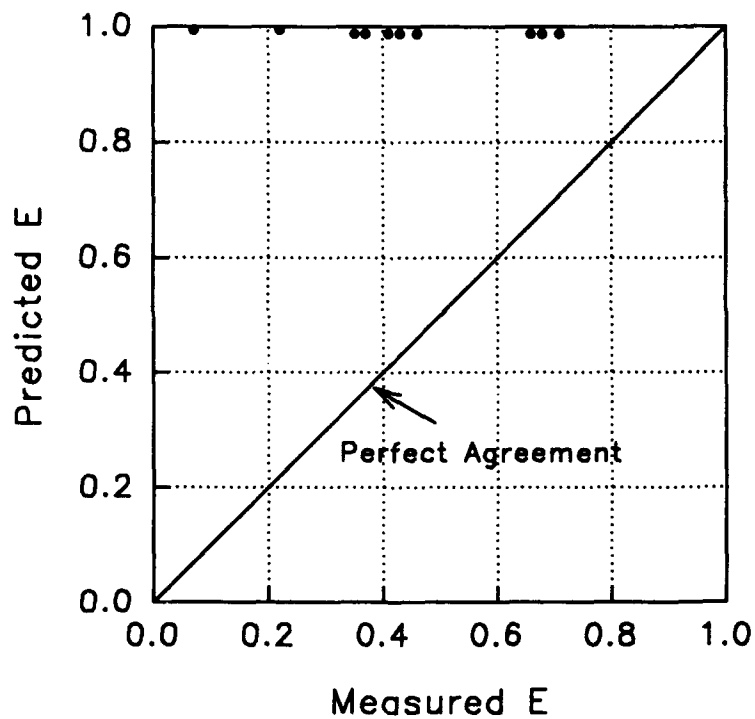
Figure D26. Forsee equation for gated sills. Predicted values of gas transfer versus measured values
