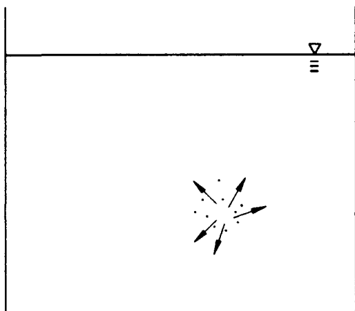
Figure 1. Transport due to diffusion in quiescent water (after Tsivoglou and Wallace 1972)
