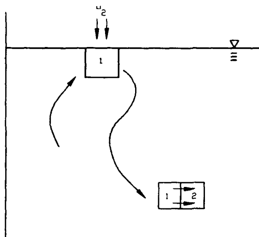
Figure 2. Transport due to diffusion and turbulent mixing
