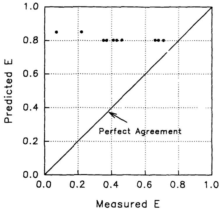
Figure D22. Tsivoglou and Wallace equation for gated sills. Predicted values of gas transfer versus measured values
