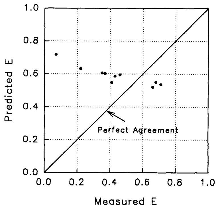
Figure D11. Thene equation for gated sills. Predicted values of gas transfer versus measured values
