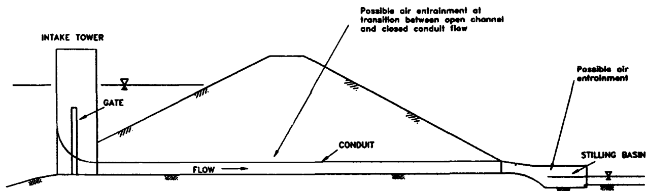
Figure 7. Transitional flows through a gated conduit
