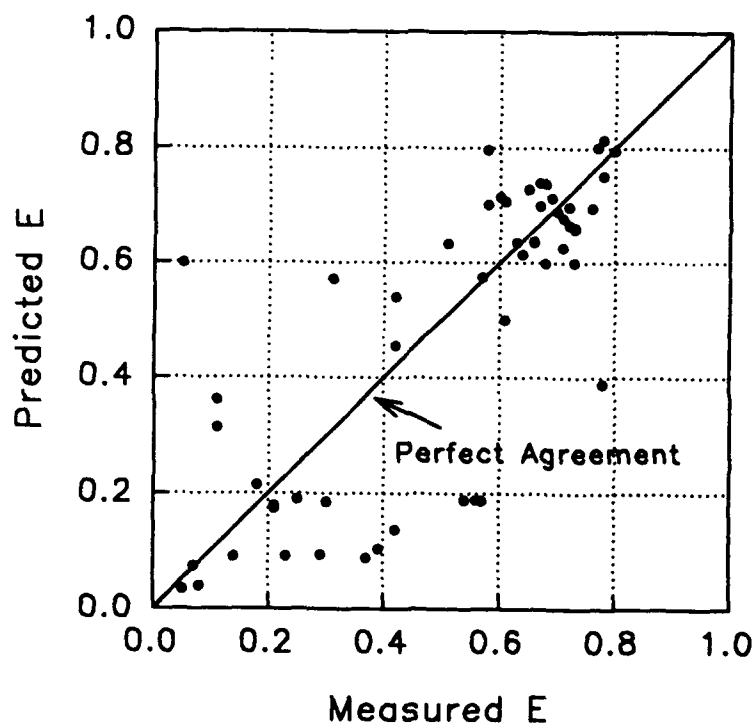
Figure D13. Nakasone equation for weirs. Predicted values of gas transfer versus measured values
