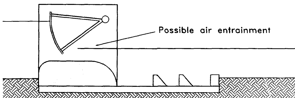
Figure 4. Open channel flow at gated structure (gated sill) (after ASCE 1991)
