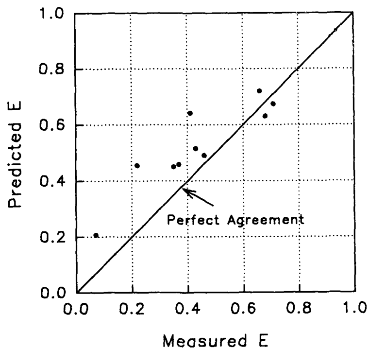
Figure D30. Preul and Holler equation for gated sills. Predicted values of gas transfer versus measured values
