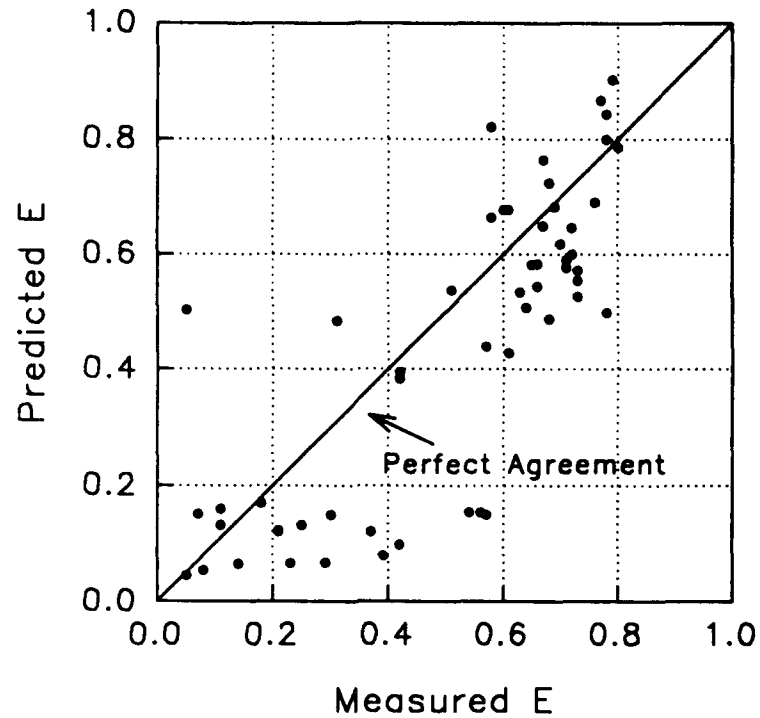
Figure D10. Thene equation for weirs. Predicted values of gas transfer versus measured values
