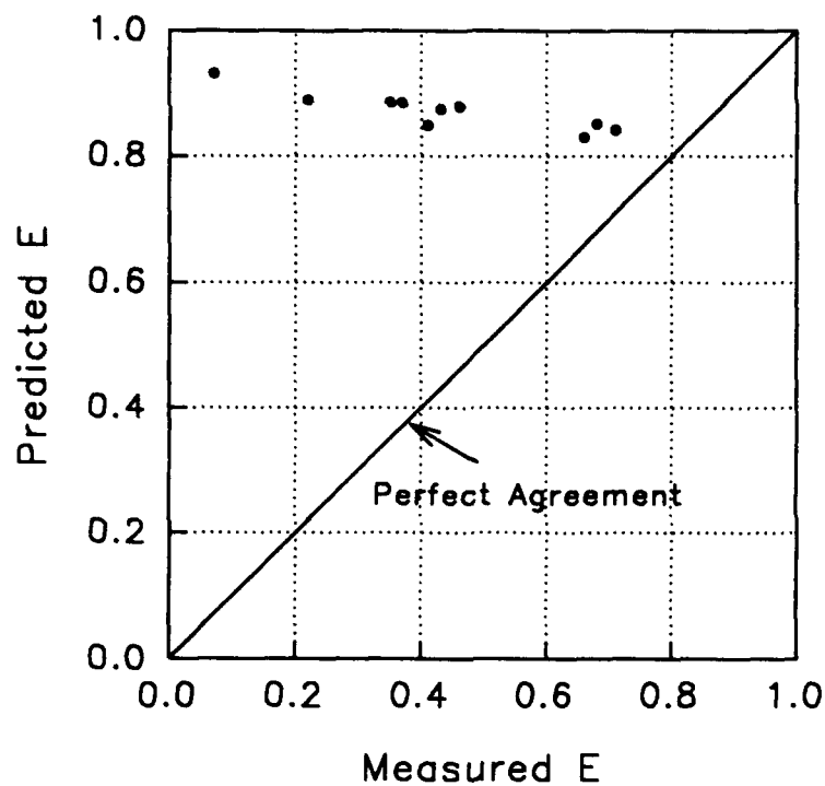
Figure D33. Rindels and Gulliver equation for gated sills. Predicted values of gas transfer versus measured values
