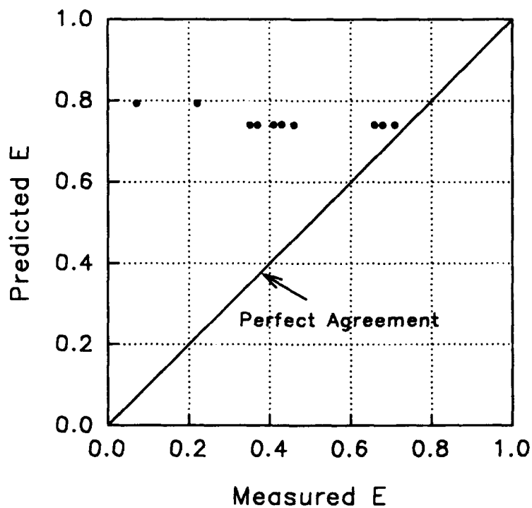
Figure D40. Wilhelms and Smith equation for gated sills. Predicted values of gas transfer versus measured values
