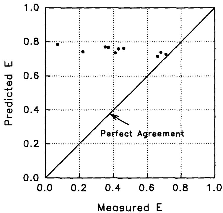
Figure D36. Wilhelms equation for gated sills. Predicted values of gas transfer versus measured values
