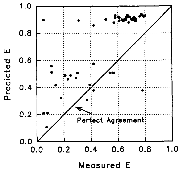
Figure D25. Forsee equation for weirs. Predicted values of gas transfer versus measured values
