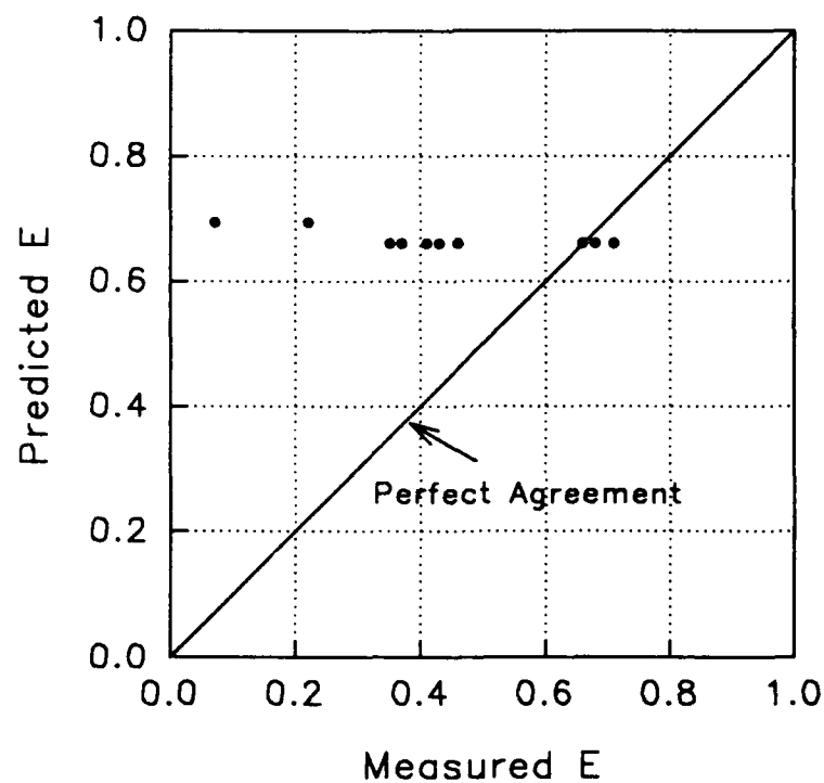
Figure D18. Holler equation for gated sills. Predicted values of gas transfer versus measured values
