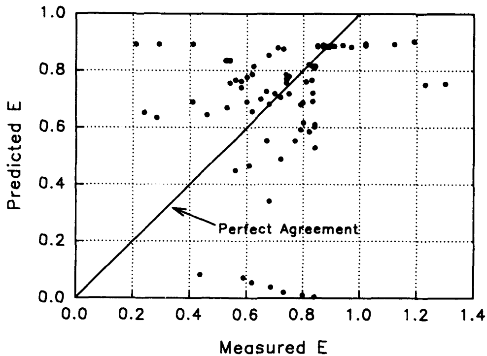
Figure D1. Avery and Novak equation for ogee spillways. Predicted values of gas transfer versus measured values
