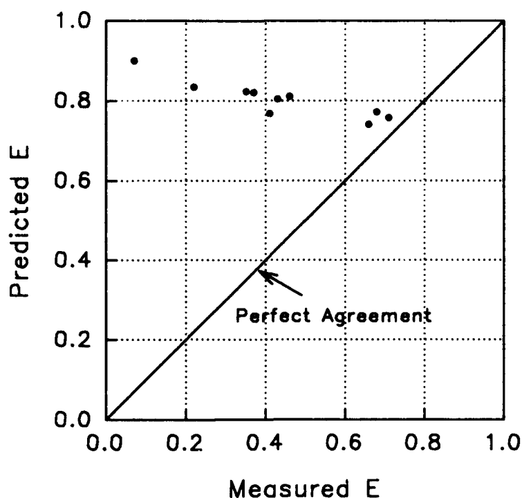
Figure D14. Nakasone equation for gated sills. Predicted values of gas transfer versus measured values
