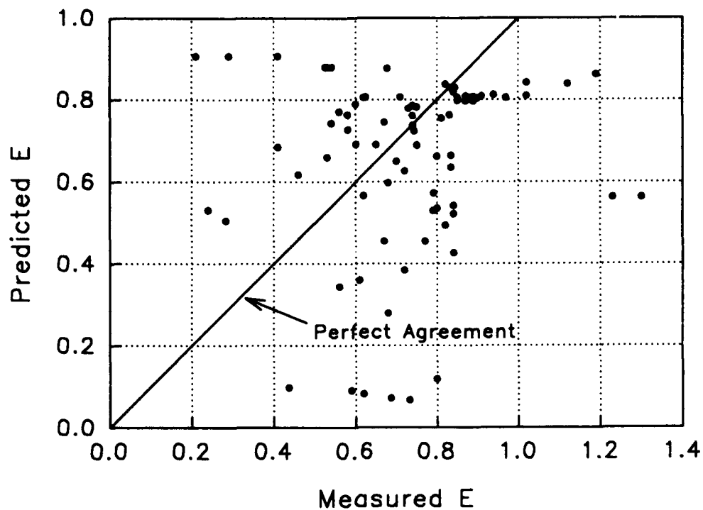
Figure D8. Thene equation for ogee spillways. Predicted values of gas transfer versus measured values
