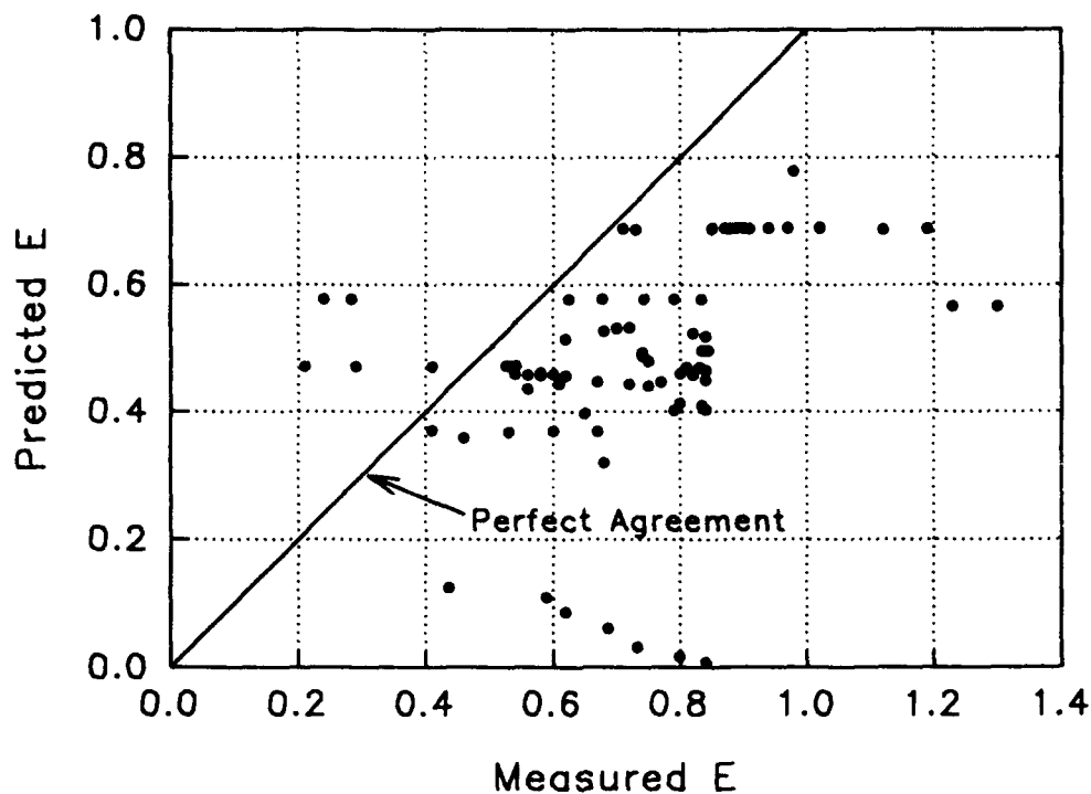
Figure D15. Holler equation for ogee spillways. Predicted values of gas transfer versus measured values
