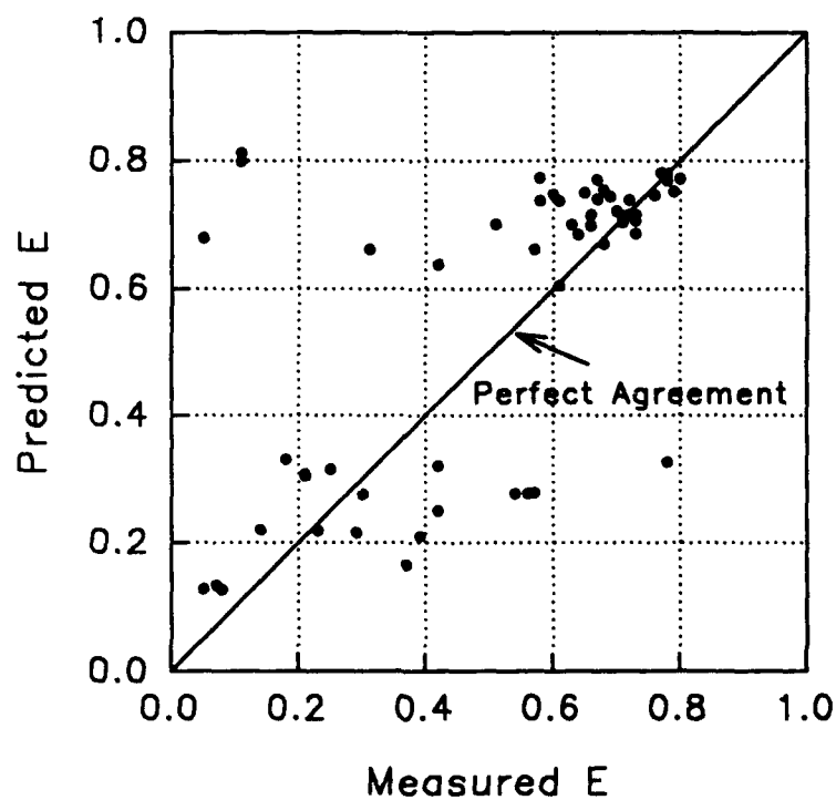
Figure D32. Rindels and Gulliver equation for weirs. Predicted values of gas transfer versus measured values
