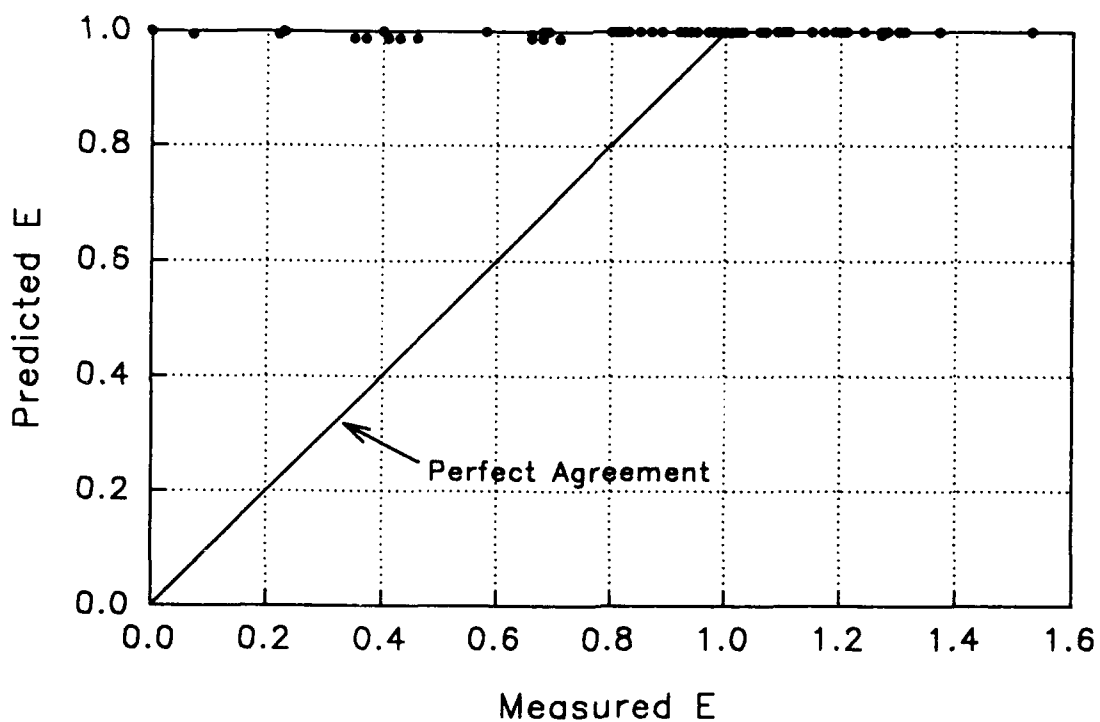
Figure D24. Foree equation for gated conduits. Predicted values of gas transfer versus measured values
