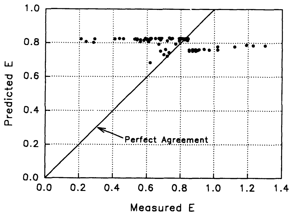
Figure D34. Wilhelms equation for ogee spillways. Predicted values of gas transfer versus measured values
