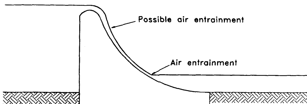
Figure 3. Open channel flow on a spillway (after ASCE 1991)
