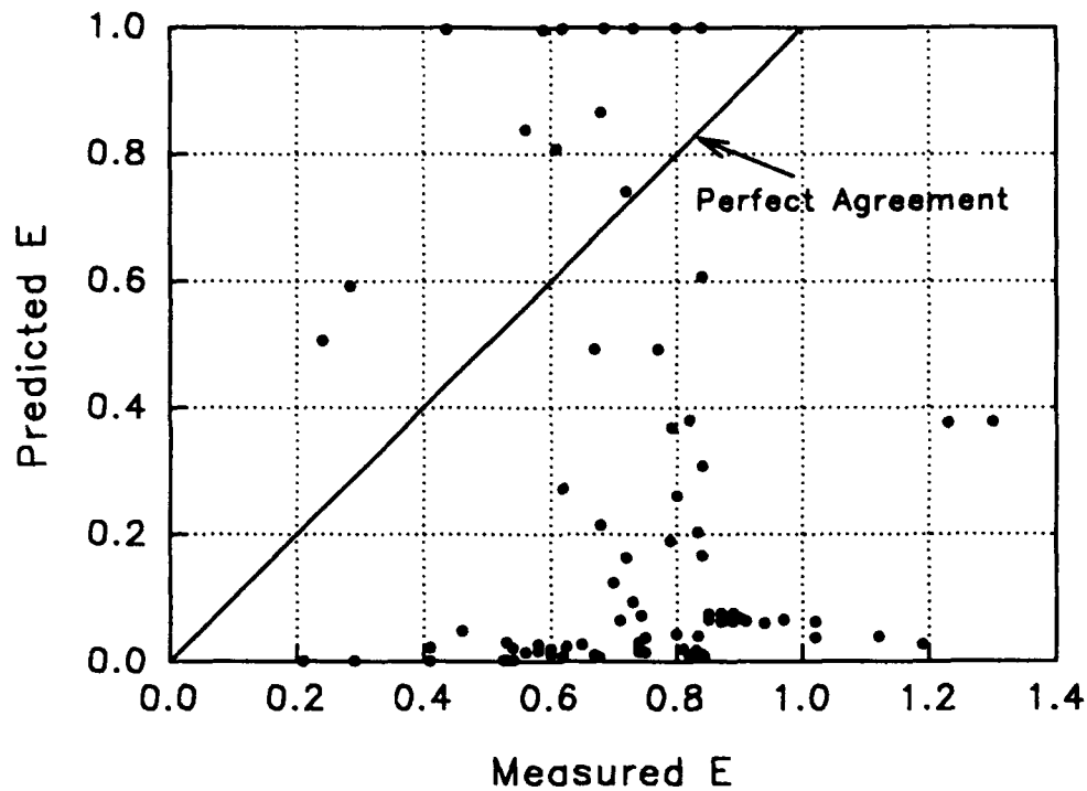
Figure D27. Preul and Holler equation for ogee spillways. Predicted values of gas transfer versus measured values
