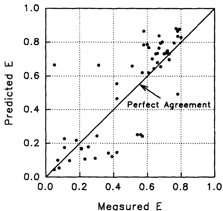
Figure D3. Avery and Novak equation for weirs. Predicted values of gas transfer versus measured values
