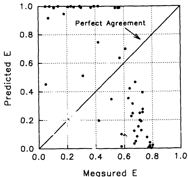
Figure D29. Preul and Holler equation for weirs. Predicted values of gas transfer versus measured values
