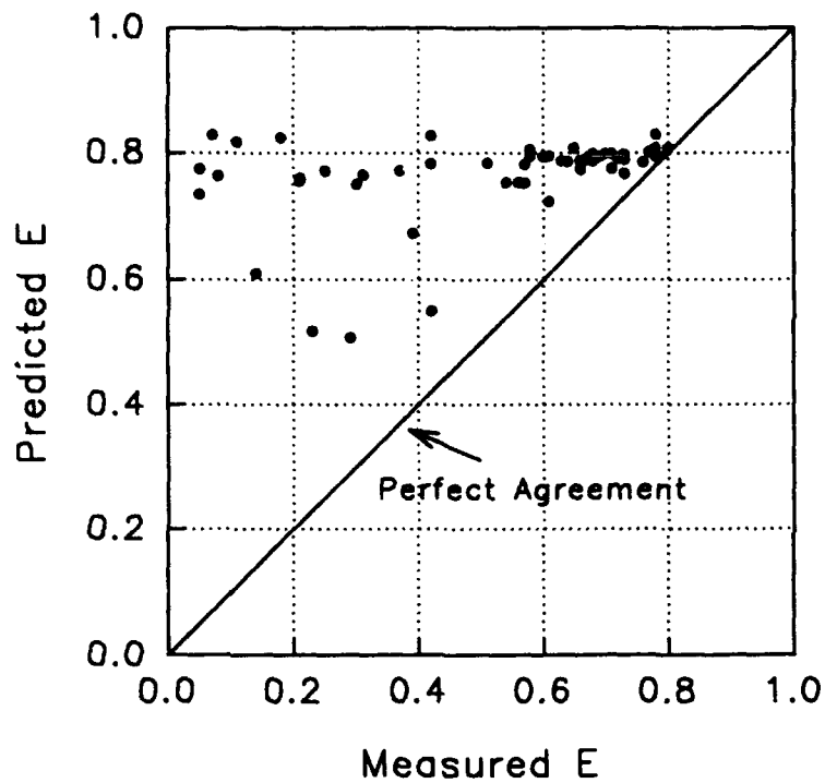
Figure D35. Wilhelms equation for weirs. Predicted values of gas transfer versus measured values
