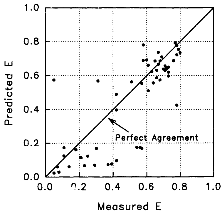
Figure D6. Thene's adjustment to the Avery and Novak equation for weirs. Predicted values of gas transfer versus measured values
