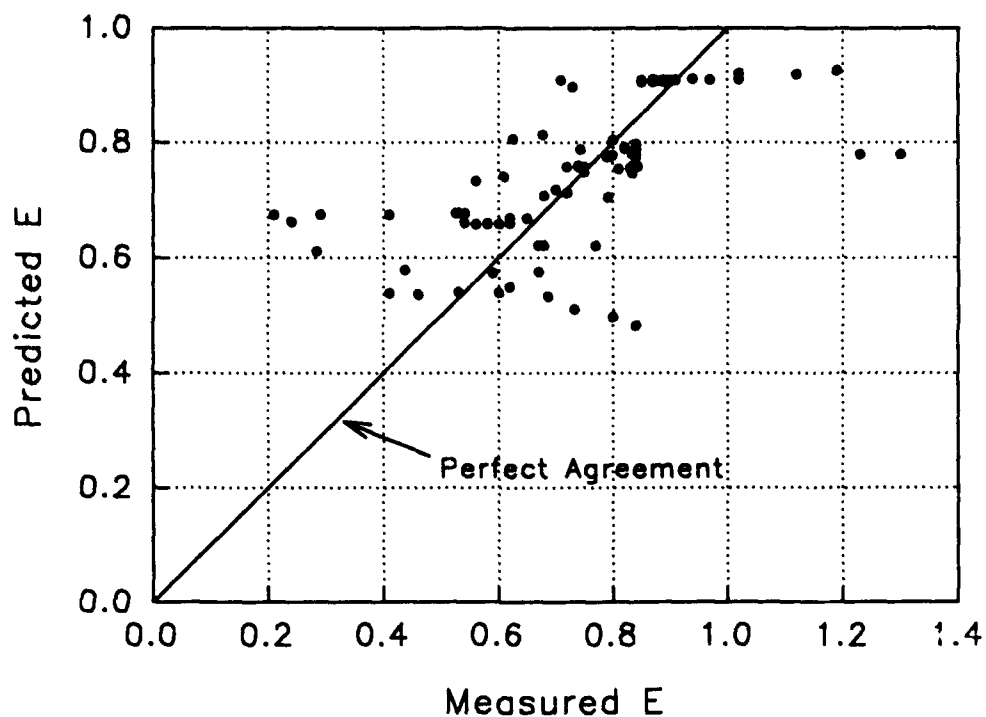
Figure D31. Rindels and Gulliver equation for ogee spillways. Predicted values of gas transfer versus measured values
