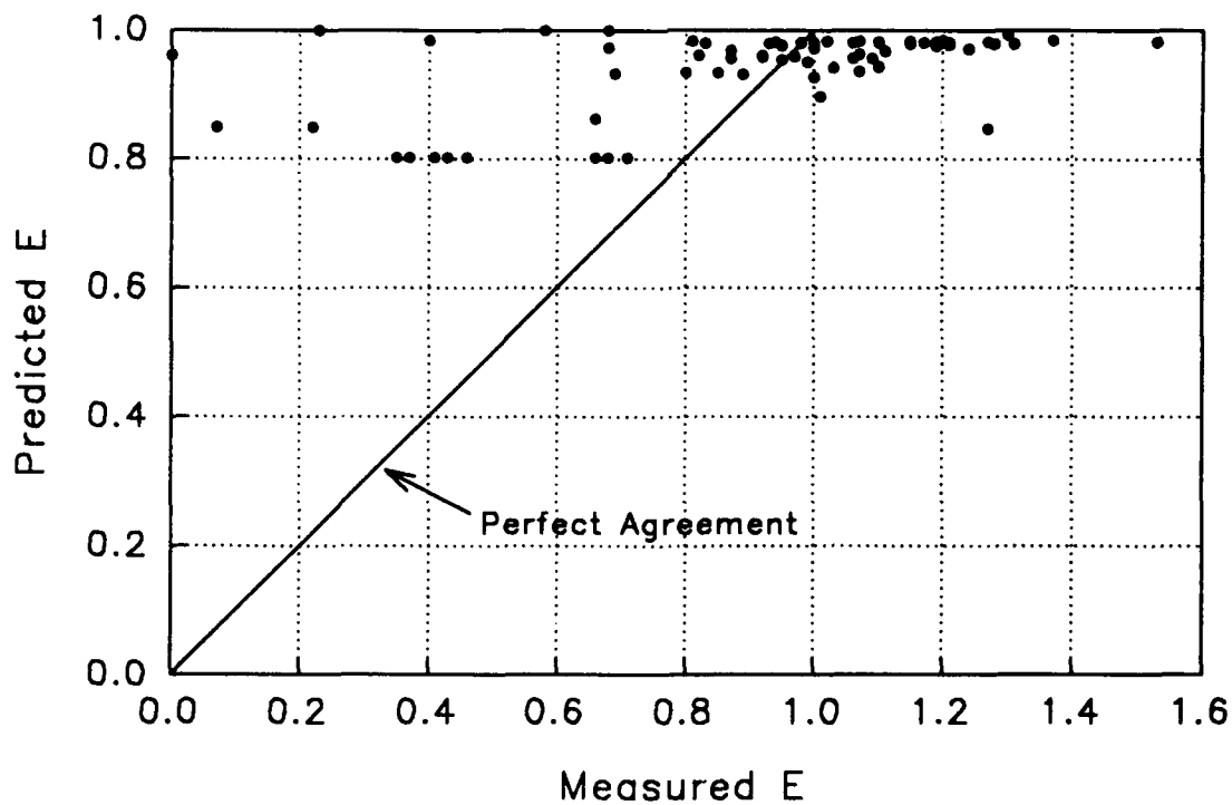
Figure D20. Tsivoglou and Wallace equation for gated conduits. Predicted values of gas transfer versus measured values
