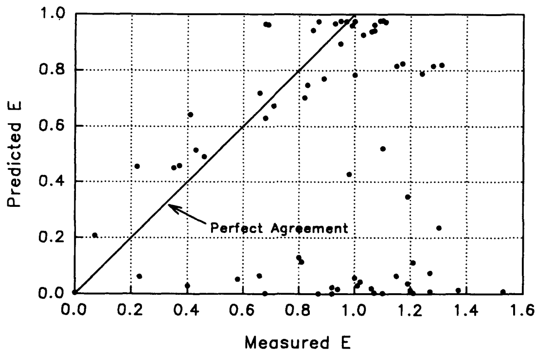
Figure D28. Preul and Holler equation for gated conduits. Predicted values of gas transfer versus measured values
