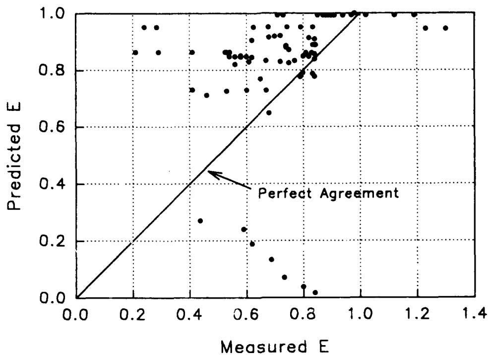
Figure D23. Foree equation for ogee spillways. Predicted values of gas transfer versus measured values
