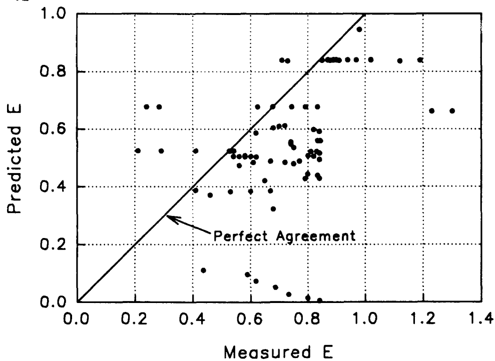
Figure D19. Tsivoglou and Wallace equation for ogee spillways. Predicted values of gas transfer versus measured values
