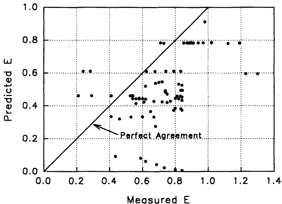
Figure D37. Wilhelms and Smith equation for ogee spillways. Predicted values of gas transfer versus measured values
