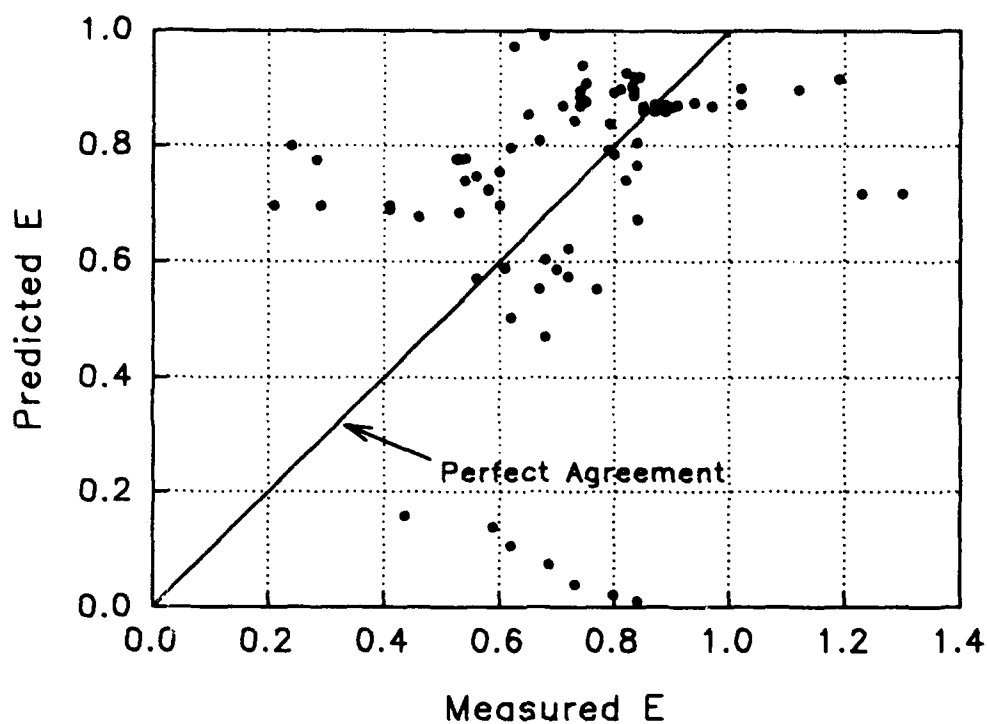
Figure D12. Nakasone equation for ogee spillways. Predicted values of gas transfer versus measured values
