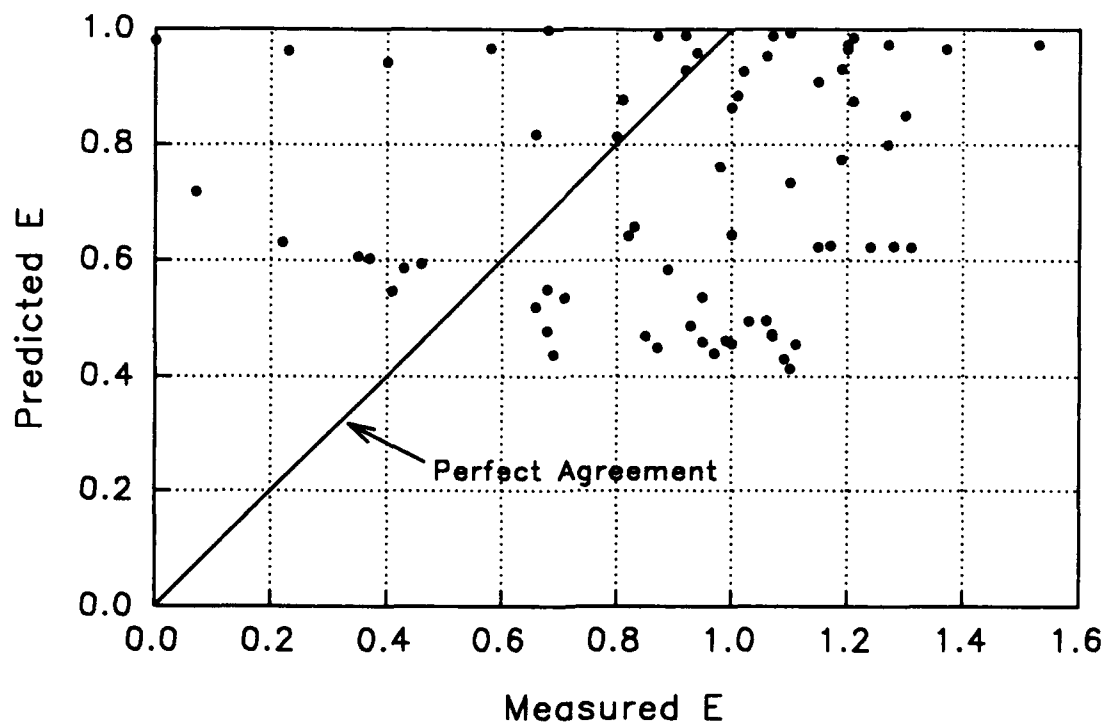
Figure D9. Thene equation for gated conduits. Predicted values of gas transfer versus measured values
