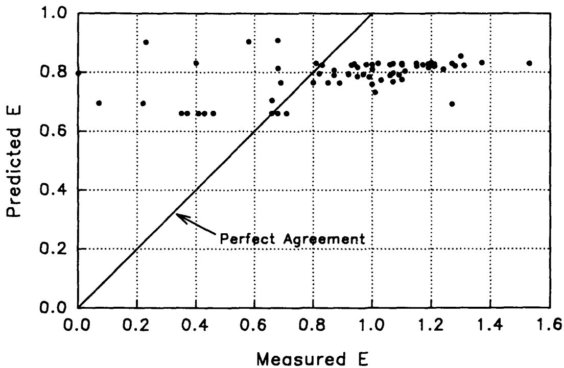
Figure D16. Holler equation for gated conduits. Predicted values of gas transfer versus measured values
