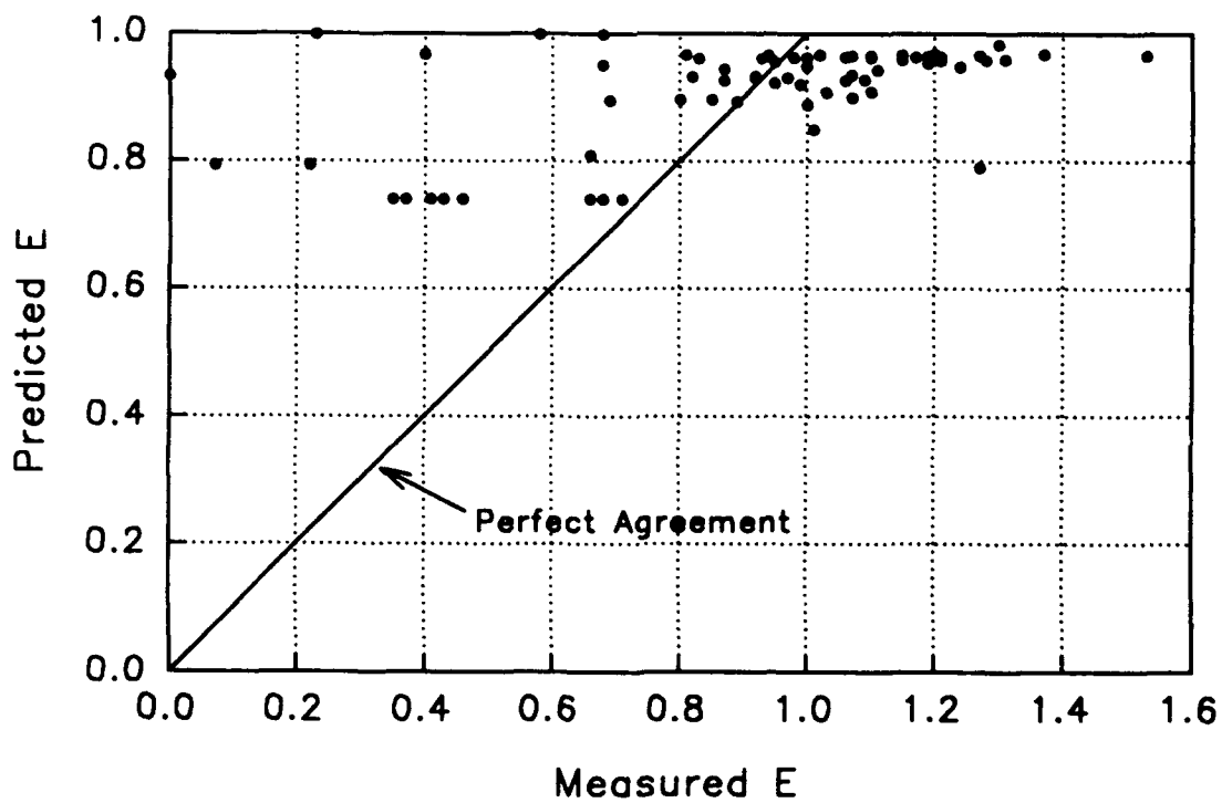
Figure D2. Avery and Novak equation for gated conduits. Predicted values of gas transfer versus measured values
