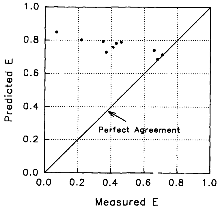
Figure D7. Thene's adjustment to the Avery and Novak equation for gated sills. Predicted values of gas transfer versus measured values
