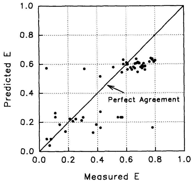
Figure D21. Tsivoglou and Wallace equation for weirs. Predicted values of gas transfer versus measured values
