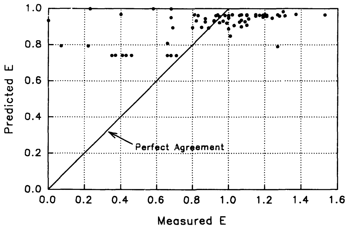
Figure D38. Wilhelms and Smith equation for gated conduits. Predicted values of gas transfer versus measured values
