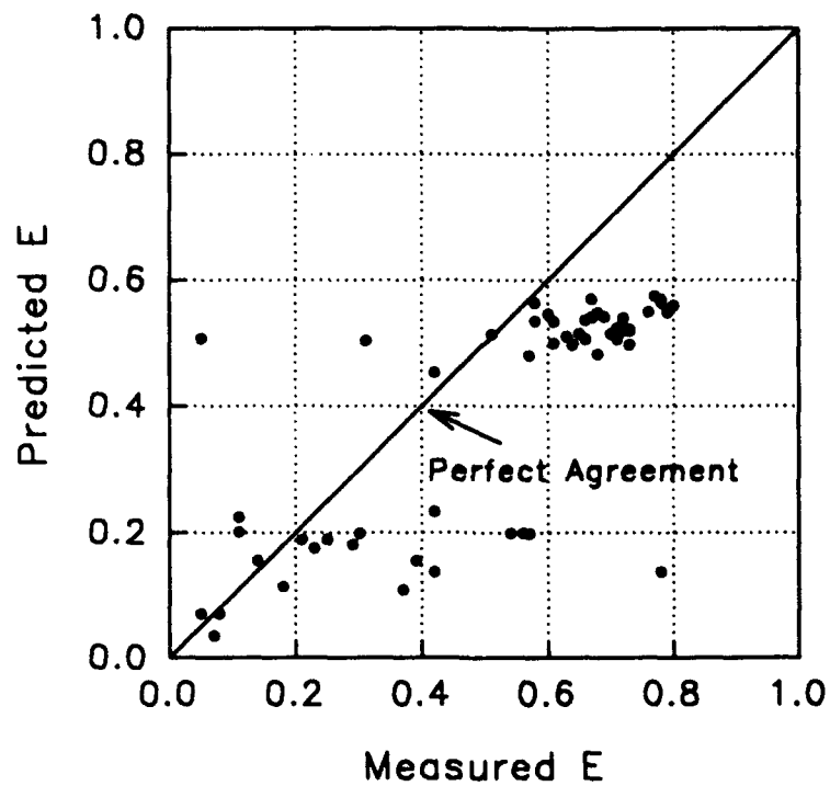
Figure D39. Wilhelms and Smith equation for weirs. Predicted values of gas transfer versus measured values
