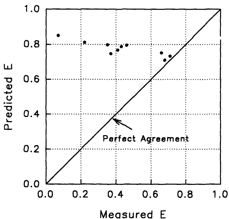
Figure D4. Avery and Novak equation for gated sills. Predicted values of gas transfer versus measured values
