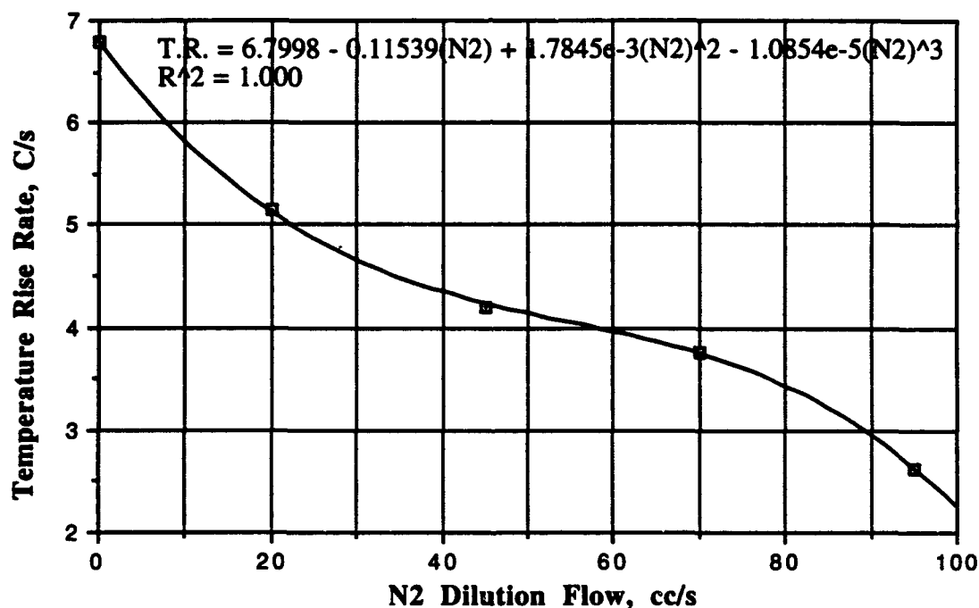
Figure 6: Dilution Effects on Sampling Temperature Rise, Height = 66 mm
