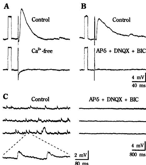
FIG. 3. Effect of \text{Ca}^{2+} -free solution or glutamate and GABA A antagonists on PSPs recorded with the whole-cell patch-clamp technique. (A) The upper trace shows an excitatory PSP evoked by extracellular stimulation dorsal to the SCN. The excitatory PSP was completely blocked (lower trace) after 17 min (range of 0–26 min; n = 4 ) in \text{Ca}^{2+} -free solution. Full recovery was obtained after 10 min in normal \text{Ca}^{2+} solution (not shown). The membrane potential in both traces was -66 mV. (B) The upper trace shows an evoked excitatory PSP from another neuron, which was blocked in a 100 \mu\text{M} 2-amino-5-phosphonopentanoic acid (AP-5), 50 \mu\text{M} 6,7-dinitroquinoxaline-2,3-dione (DNQX), and 50 \mu\text{M} bicuculline (BIC) mixture in normal \text{Ca}^{2+} (lower trace) after 13 min (range of 9–13 min; n = 3 ). The membrane potential in both traces was -78 mV. (C) The three upper left traces show continuous recordings of spontaneous PSPs in the same neuron as in B. The lower left trace shows two spontaneous PSPs at faster sweep speed and higher gain. The three right traces show a continuous recording during complete blockade of spontaneous PSPs after 12 min (range of 9–14 min; n = 6 ) in the antagonist mixture and normal \text{Ca}^{2+} . All traces in C were recorded at a membrane potential of -78 mV. Traces in A and B contain a calibration pulse (10 mV, 10 ms) before the truncated stimulus artifact.
