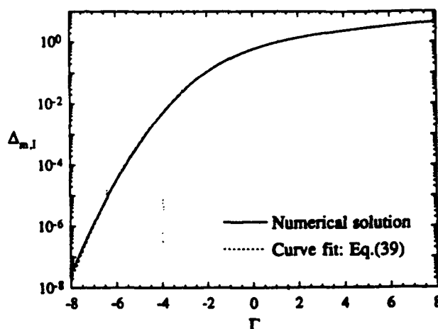
Fig. 7 Functional relation between the ignition Damköhler number \Delta_{mJ} and \Gamma for the intermediate case for q = 1 .
