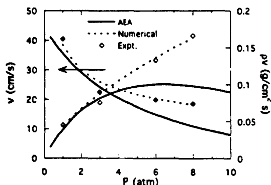
Fig. 7. Comparison of experimentally measured velocity and burning rate with values obtained numerically and with present asymptotic theory. Solid diamonds denote velocity.
