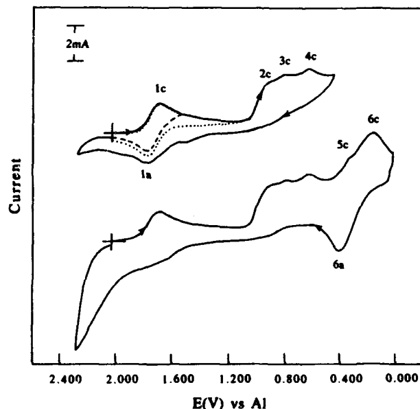
Fig. 7. Cyclic voltammograms of 19.1 \times 10^{-3} \text{M} \text{WOCl}_4 at a glassy carbon electrode in \text{AlCl}_3\text{-NaCl}_{\text{melt}} at 175°C. Scan rate was 0.050 V/s.
