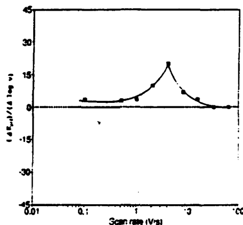
Fig. 3. Plot of the function (\Delta E_{p/2})/(\Delta \log v) vs. the scan rate for the first reduction wave obtained by CV for Nb(V) in AlCl 3 -NbCl 5 . The Nb(V) concentration was 2.91 \times 10^{-2} M , the working electrode was a tungsten wire, the temperature was 178°C, and the scan rate ranged from 0.1 to 50 V/s. The dotted line represents the curve expected in the complete absence of complicating factors.
