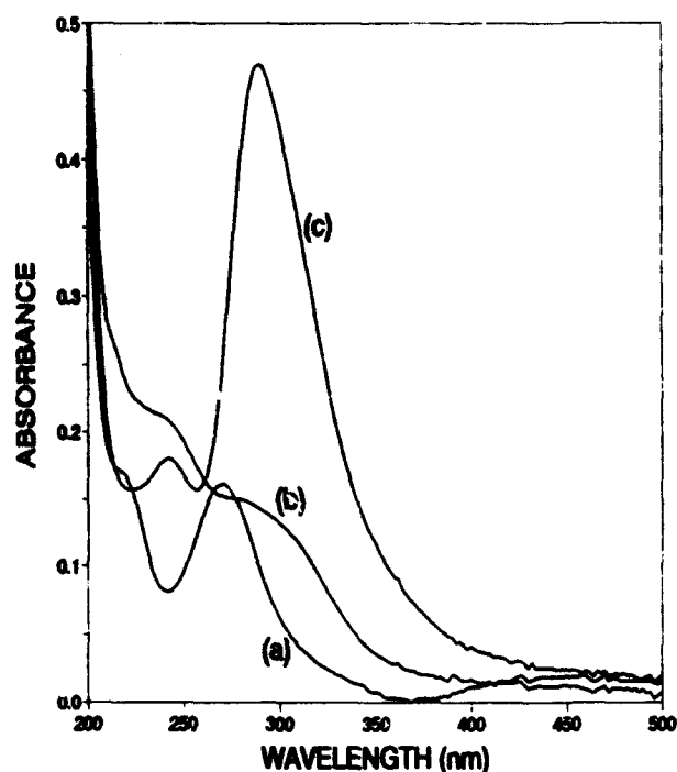
Fig. 3. UV-visible absorption spectra of niobium (V) species in a basic melt, \text{AlCl}_3\text{-NaCl}_{\text{melt}} (2.317 g), at 200°C: (a) the initial melt containing 0.17 mM \text{NbOCl}_2 ; (b) 16 min; and (c) 45 min after the introduction of 10 \mu\text{l} \text{CCl}_4 ; the quartz cell path length was 2 mm.
