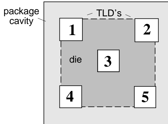
Figure 2. Arrangement of TLD's in package cavity.
