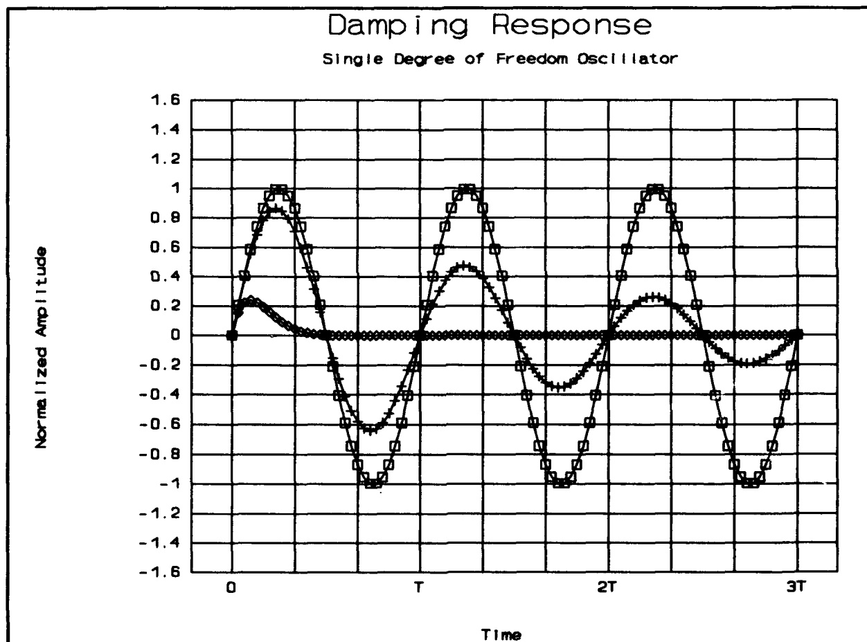
Figure 10 Response of SDOF Oscillator With Various Degrees of Damping
