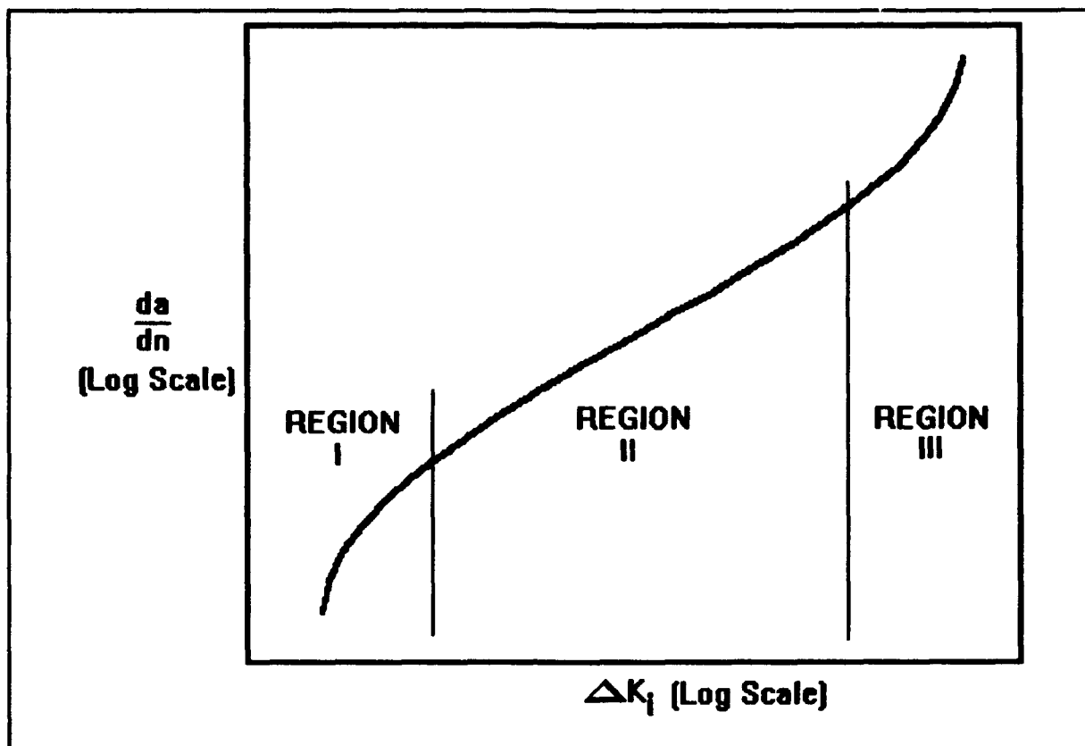
Figure 12 Schematic Representation of Crack Growth in Steels
