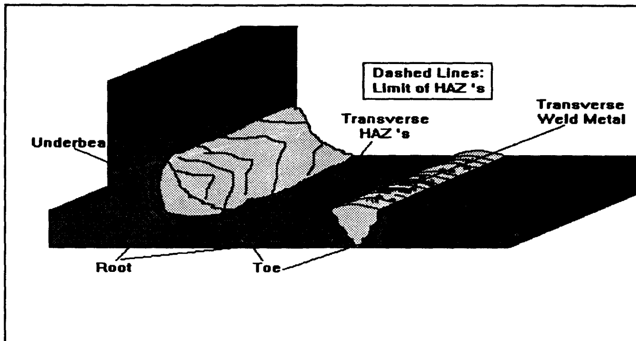
Figure 5 Locations of Delayed Cracks Around Fillet and Butt Welds
