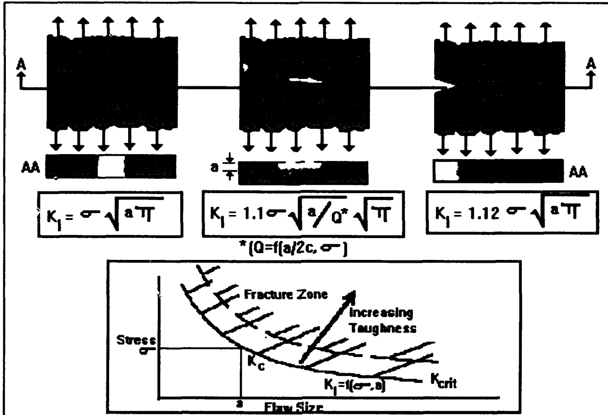
Figure 17 K_I for various cracks, stress/ flaw size/ toughness curves.
