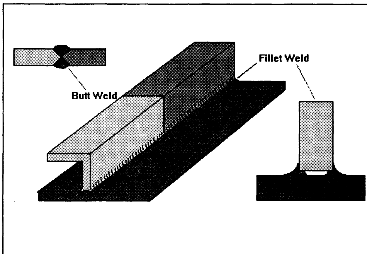
Figure 19 Weld Joint Geometry Sketch
