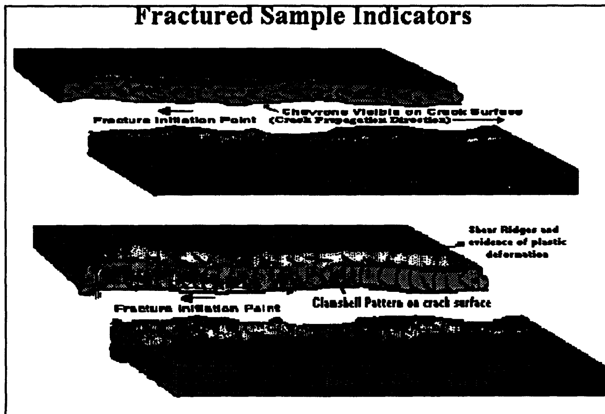
Figure 16 Fracture Mode Identification Sketch
