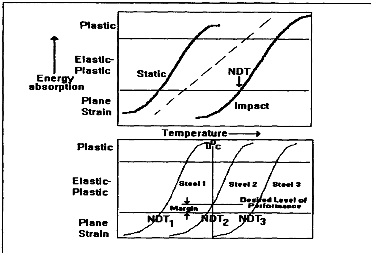
Figure 18 Brittle Fracture Transition Curves
