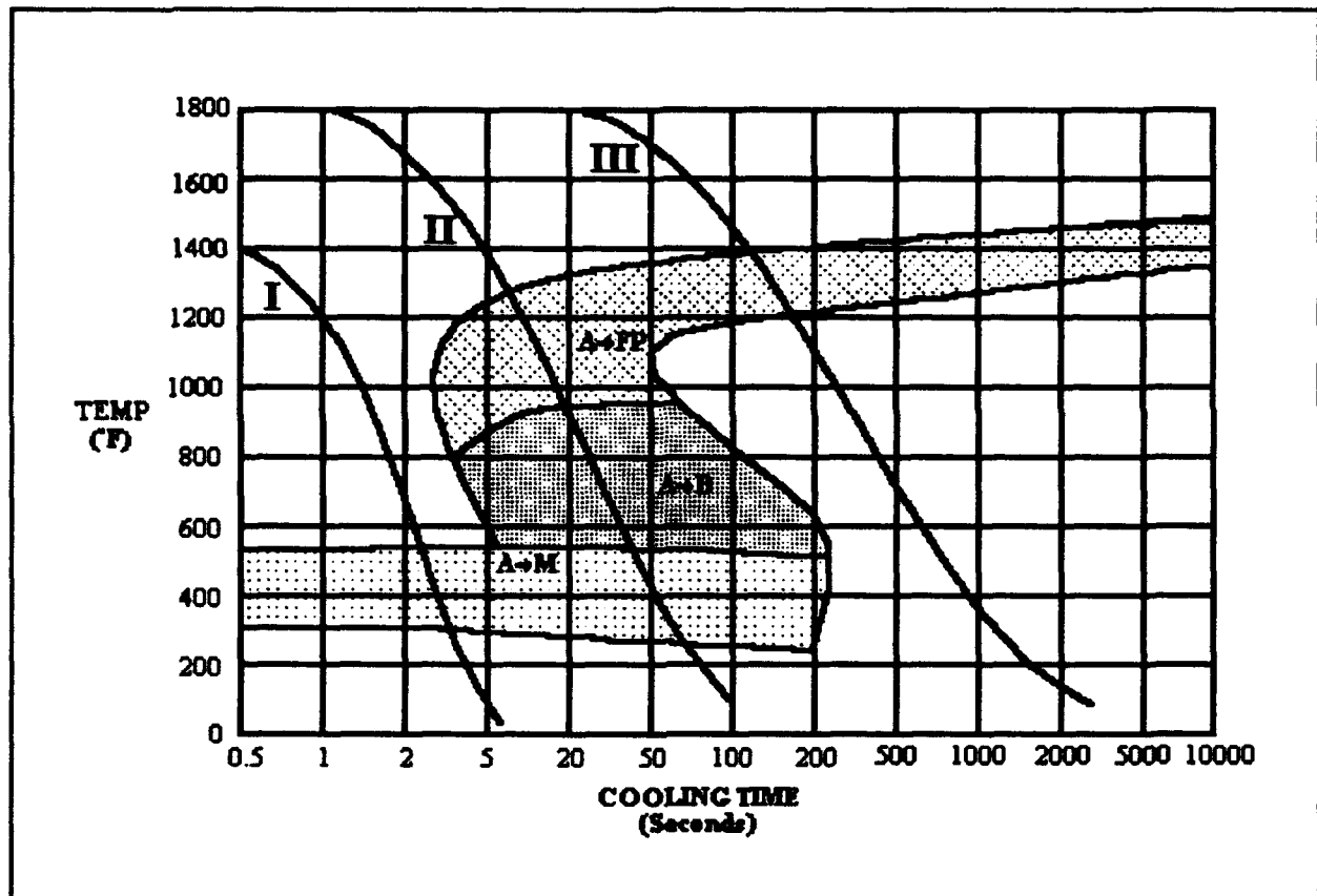
Figure 6 Steel Crystalline Transformation/ Cooldown Curves
