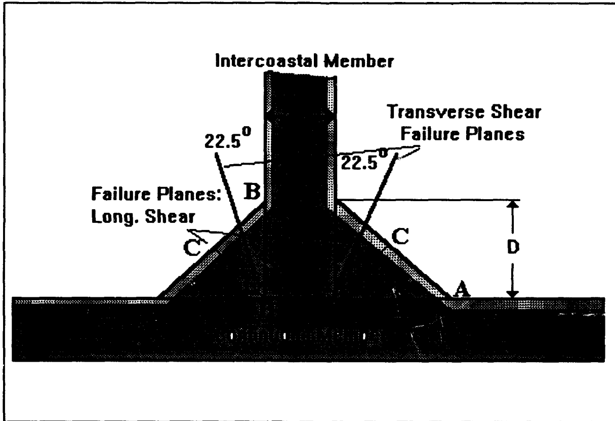
Figure 3 Fillet weld failure planes
