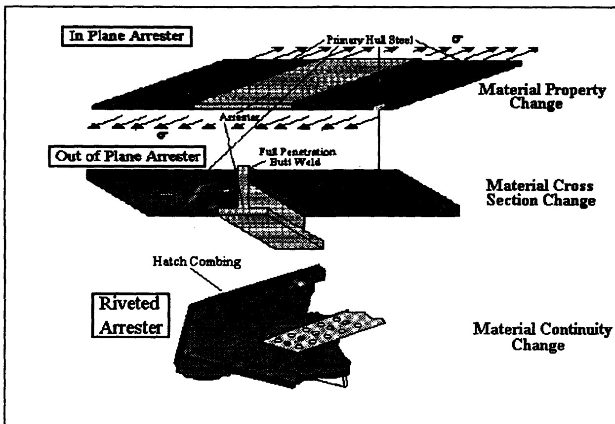
Figure 14 Crack Arrest Schemes
