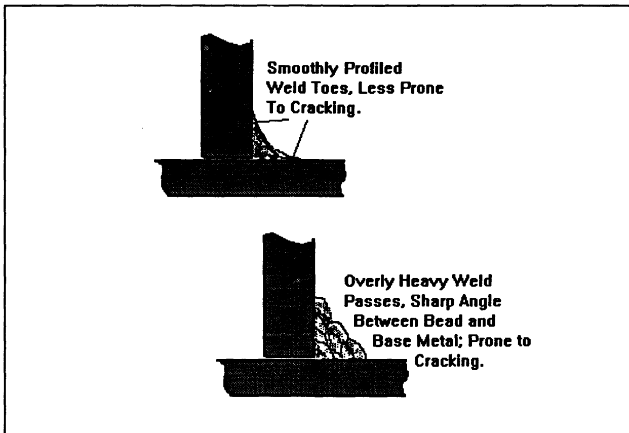
Figure 4 Favorable vs. Unfavorable Fillet Weld Profiles
