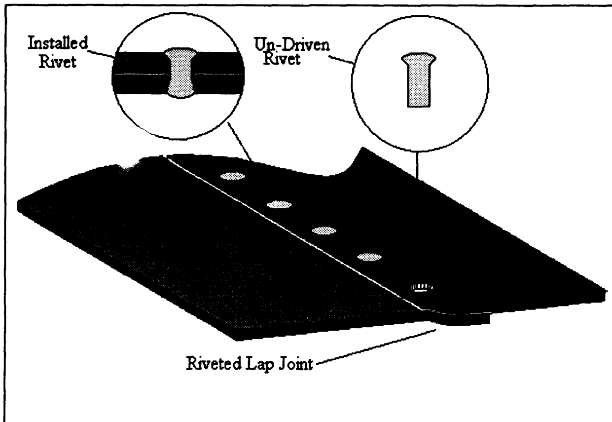
Figure 7 Riveted Lap Joint
