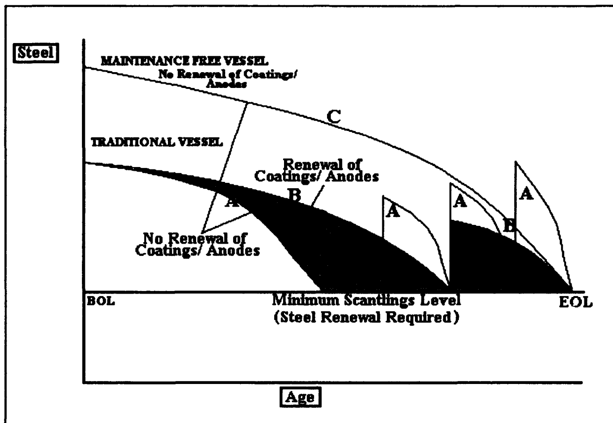
Figure 1 Comparison of Traditional Minimum Scantlings Vessel with "Maintenance-Free" Design.
