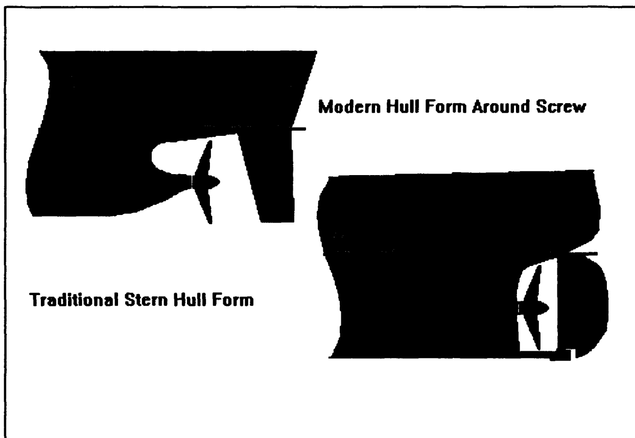
Figure 11 Modern vs. Traditional Merchant Ship Stern Configurations
