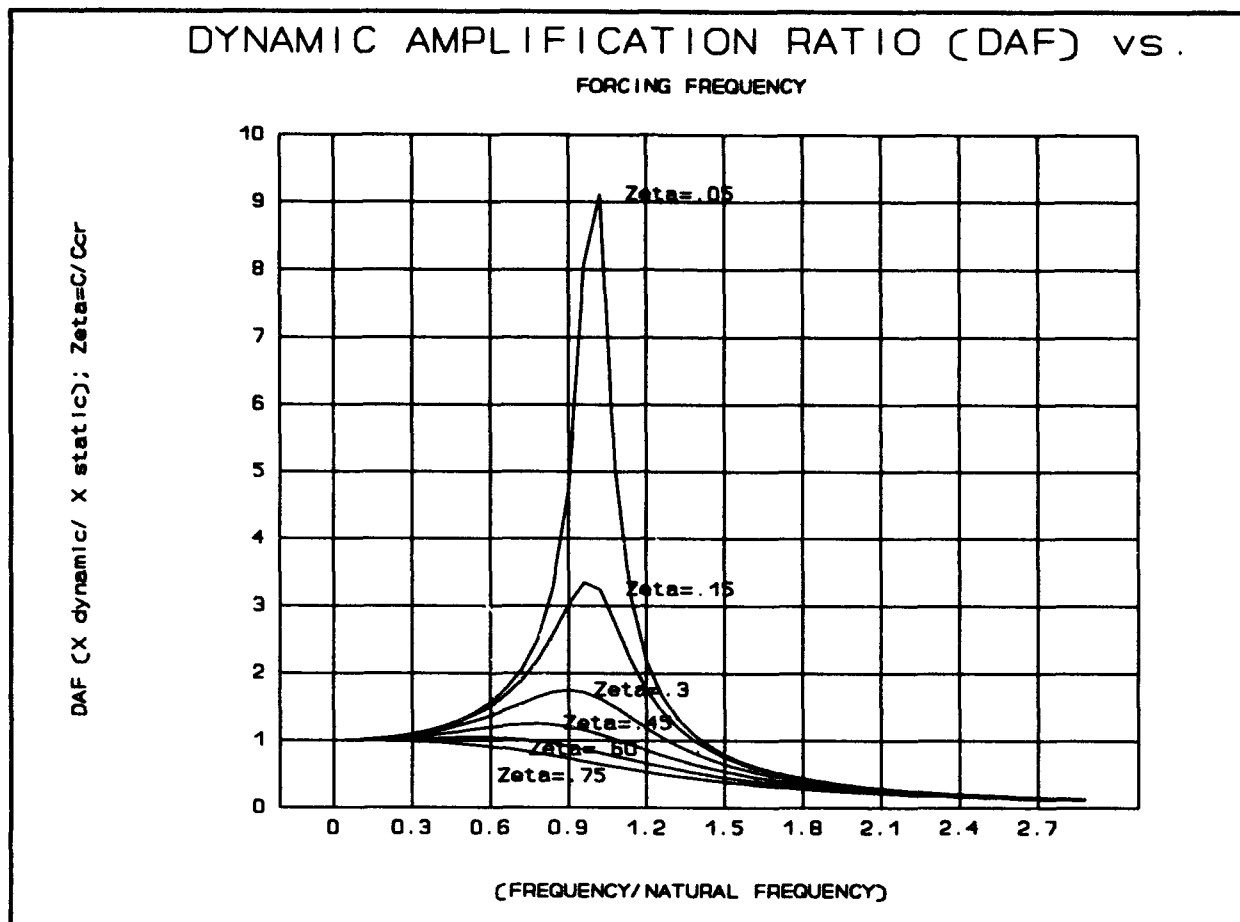
Figure 8 Dynamic Amplification vs. Frequency as a Function of Damping Ratio
