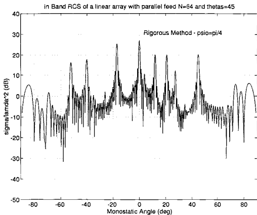
Figure 20. Inband RCS of a Linear Array with a Parallel Feed for N = 64 , \theta_s = 45^\circ , \psi_c = \pi/4 (Rigorous Method).
