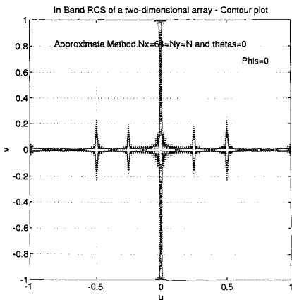
Figure 14. Inband RCS of a Two-Dimensional Array with a Parallel Feed for N_x = N_y = 64 , \theta_s = 0^\circ , \phi_s = 0^\circ . Contour Plot at 20 dB Level (Approximate Method).
