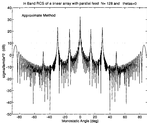
Figure 9. Inband RCS of a Linear Array with a Parallel Feed for N=128 . \theta_0 = 0^\circ (Approximate Method).
