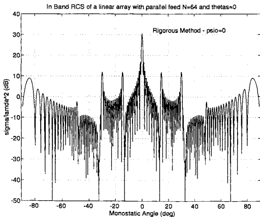
Figure 17. Inband RCS of a Linear Array with a Parallel Feed for N = 64 , \theta_s = 0^\circ , \psi_n = 0 (Rigorous Method).
