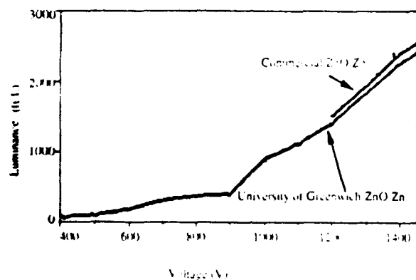
FIG. 3. Brightness-voltage characteristics for ZnO:Zn commercial phosphors.
