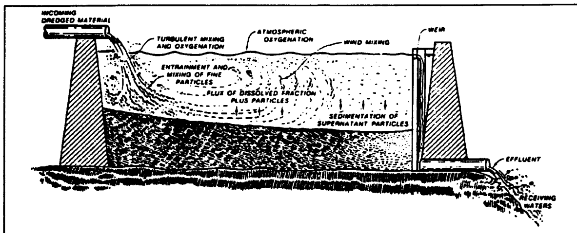
Figure 4. Schematic of an active CDF
