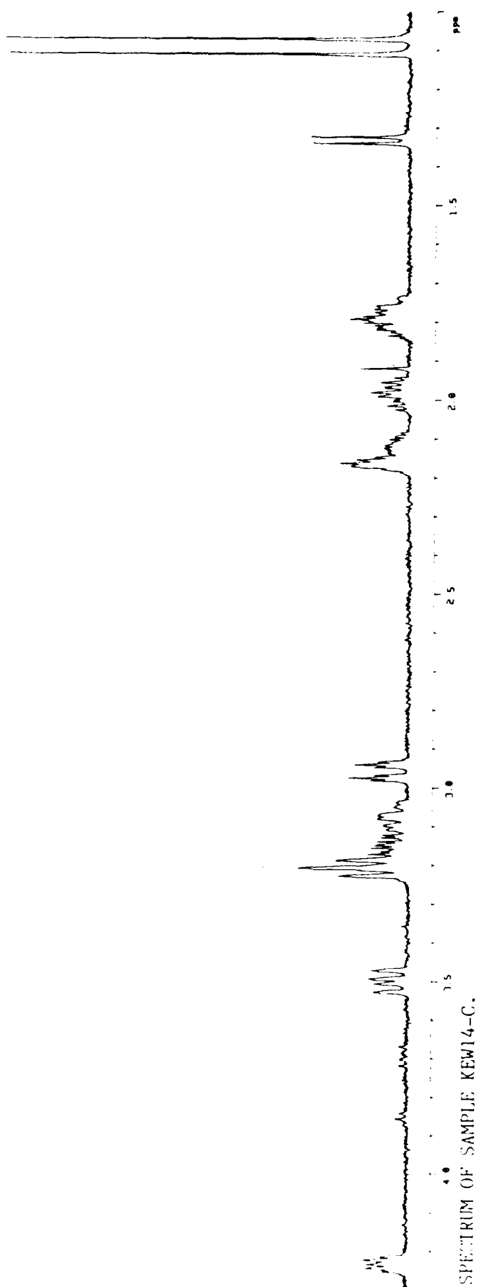
SPECTRUM OF MIXTURE OF AUTHENTIC COMPOUNDS.
