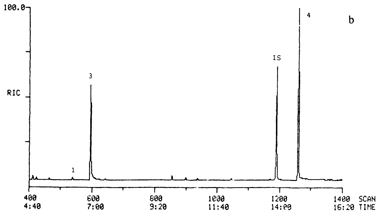
Figure F-14. a) GC/ITD/EI (Method GC2/MS2) and b) GC/MS/CI/SIM (Method GC3/MS3) Chromatograms of NMR Water Sample KFW-14C, TMS Derivative. Peak Numbers are Identified in Table 2.
