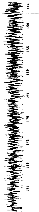
SPECTRUM OF SAMPLE W15-G.
