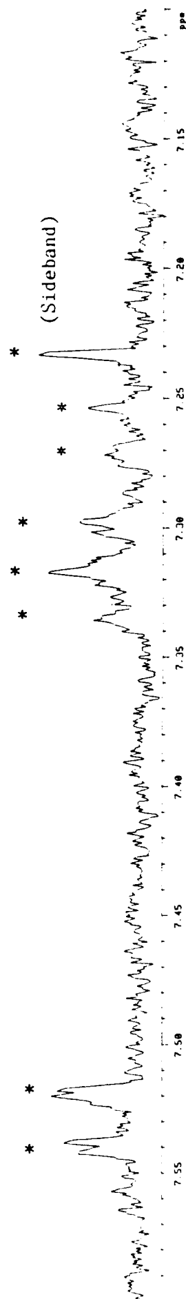
SPECTRUM OF SAMPLE SN15-C.
