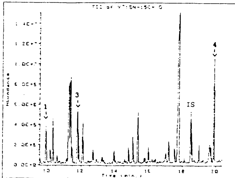
Figure F-21. GC/MSD/EI (Method GC1/MS1) Chromatogram of Water Extract SN-15C* of Soil Sample SN-15, TMS Derivative. Peak Numbers are Identified in Table 2.
