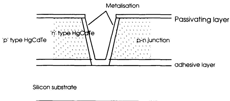
Figure 1: Construction of a photodiode using the 'loophole' technique
