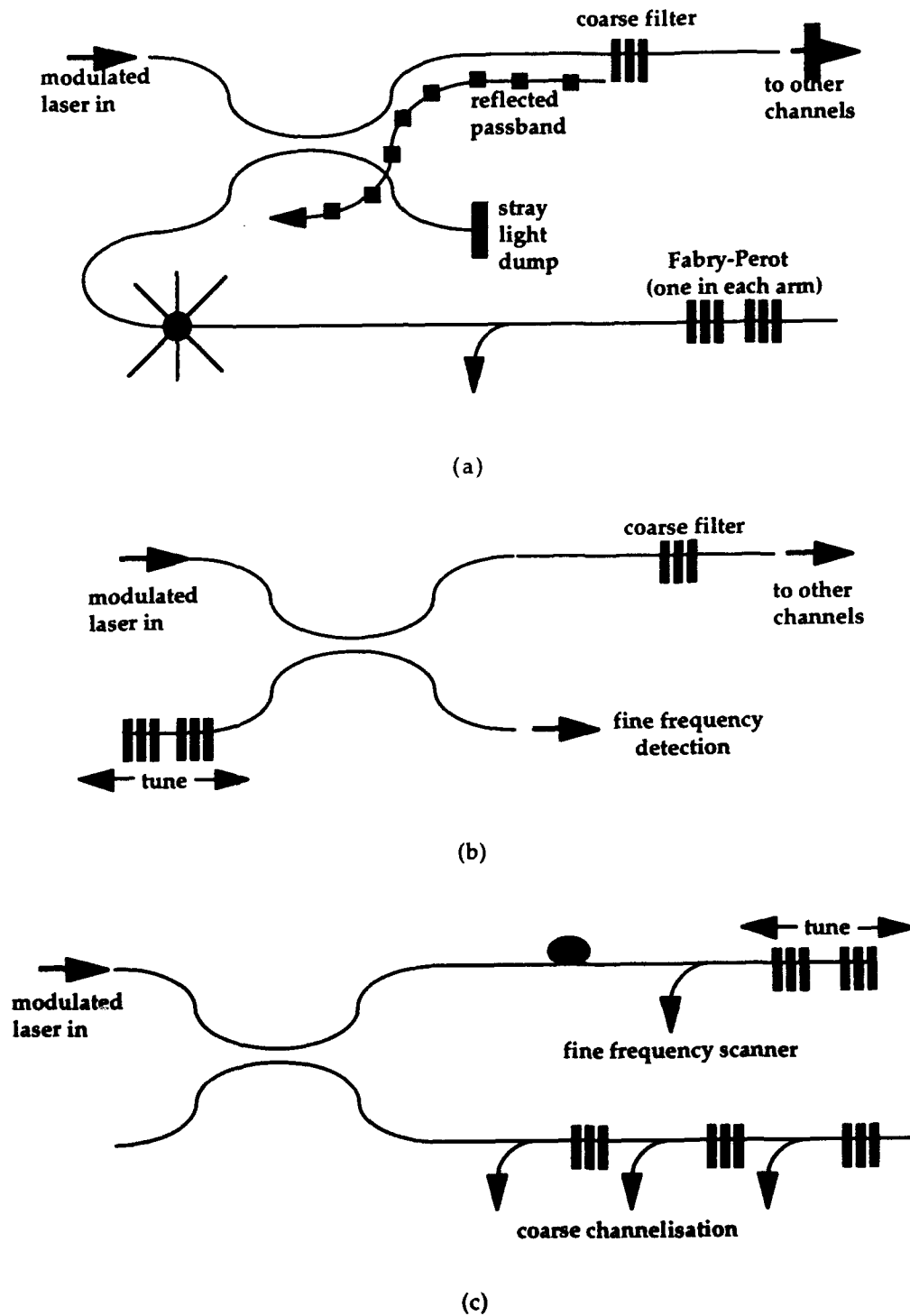
Figure 11 Various architectures for obtaining fine frequency resolution used wideband gratings. The polarisation controlling components are not shown.
