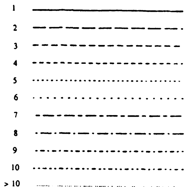
Figure 1. Representations of polyhedron edges joining neighboring points in order of increasing lengths.
