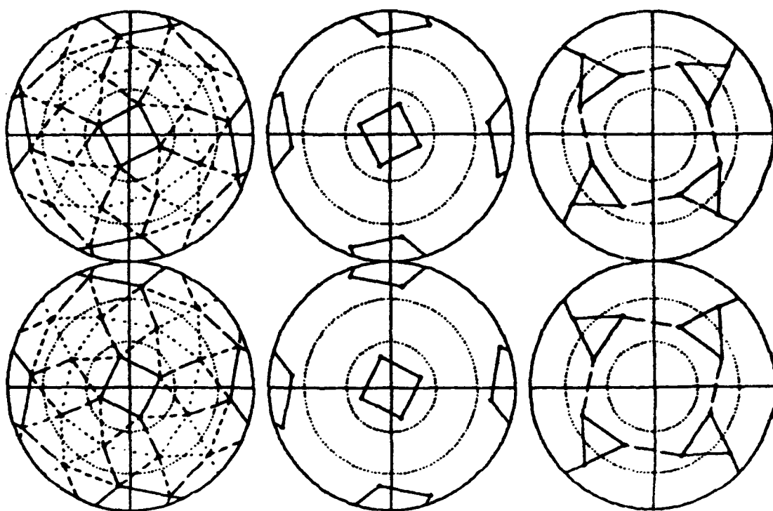
Figure 9. The equilibrium figure for N = 44 with its isoenergy subsets shown to the right. From left to right, the cube has highest individual particle energies, the cuboctahedron is next and the truncated octahedron has lowest individual particle energies.
