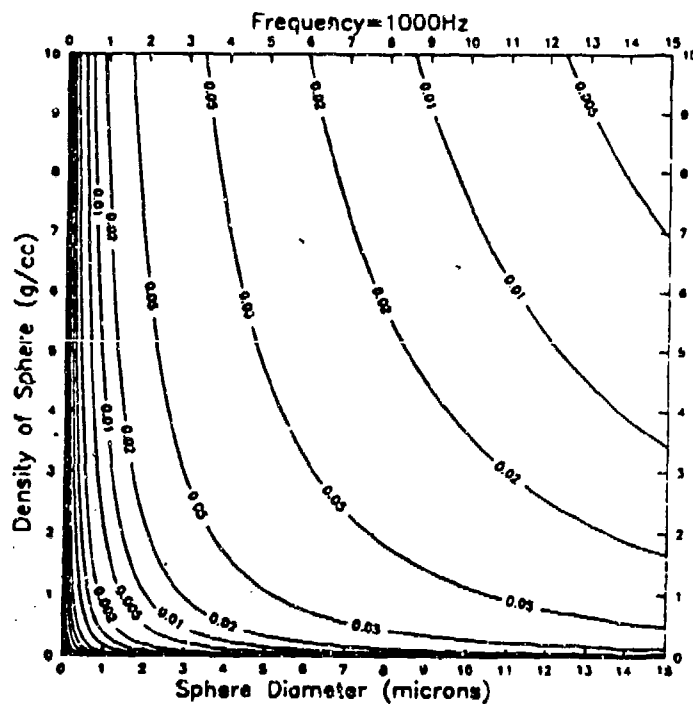
Figure 16. Aerosol Sound Absorption Coefficient ( \text{m}^2/\text{g} )
