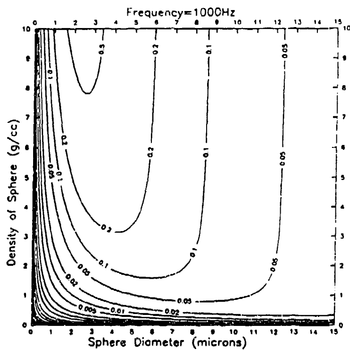
Figure 15. Aerosol Sound Absorption Coefficient ( \text{m}^2/\text{m}^3 )
