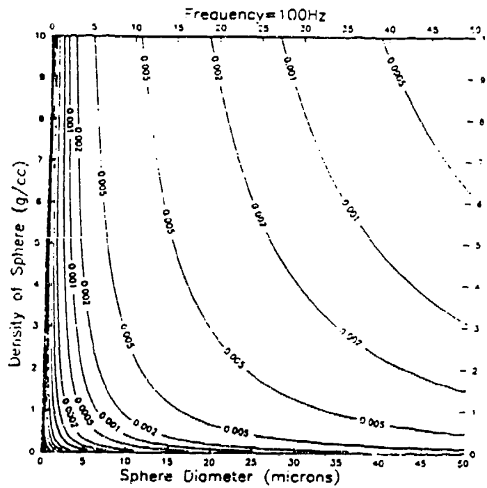
Figure 14. Aerosol Sound Absorption Coefficient ( \text{m}^2/\text{g} )
