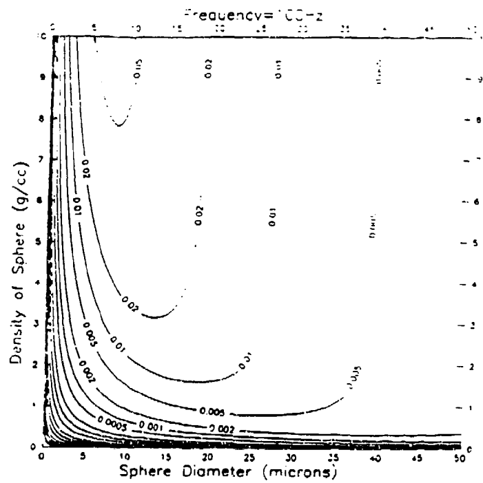
Figure 13. Aerosol Sound Absorption Coefficient ( \text{m}^2/\text{cc} )
