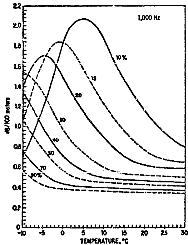
Figure 2. Attenuation of sound in air vs. temperature for various values of relative humidity and 1000 Hz frequency, at atmospheric pressure.
