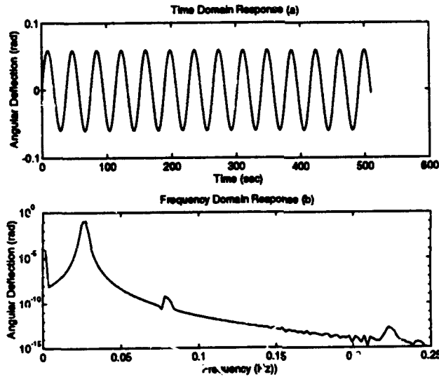
Figure 4: Tower Natural Frequency, C_D = 0
