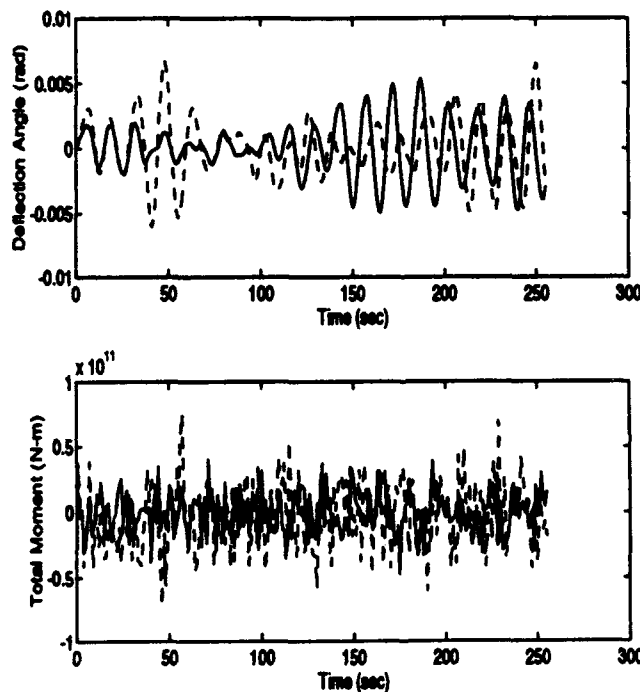
Figure 13: Tower Response - Deflection angle and Total Moment for H_s = 15 (dashed line) and 9 (solid line) (m)
