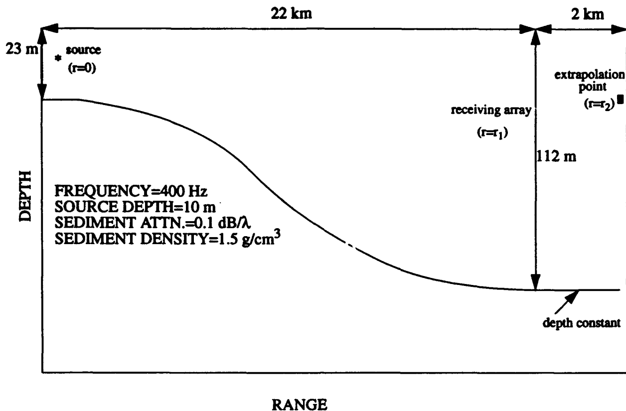
Figure 4.7. Model parameters for extrapolation test. The depth is artificially held constant between receiving array and extrapolation point.
