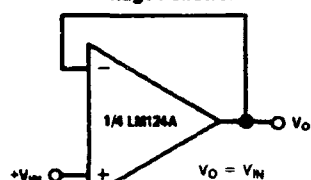
Voltage Follower
