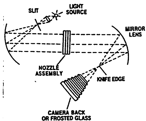
Figure 3. Schlieren configuration
