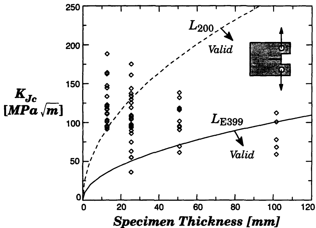
FIG. 6—Variation of fracture toughness with specimen thickness for A533-B at -75°C.
